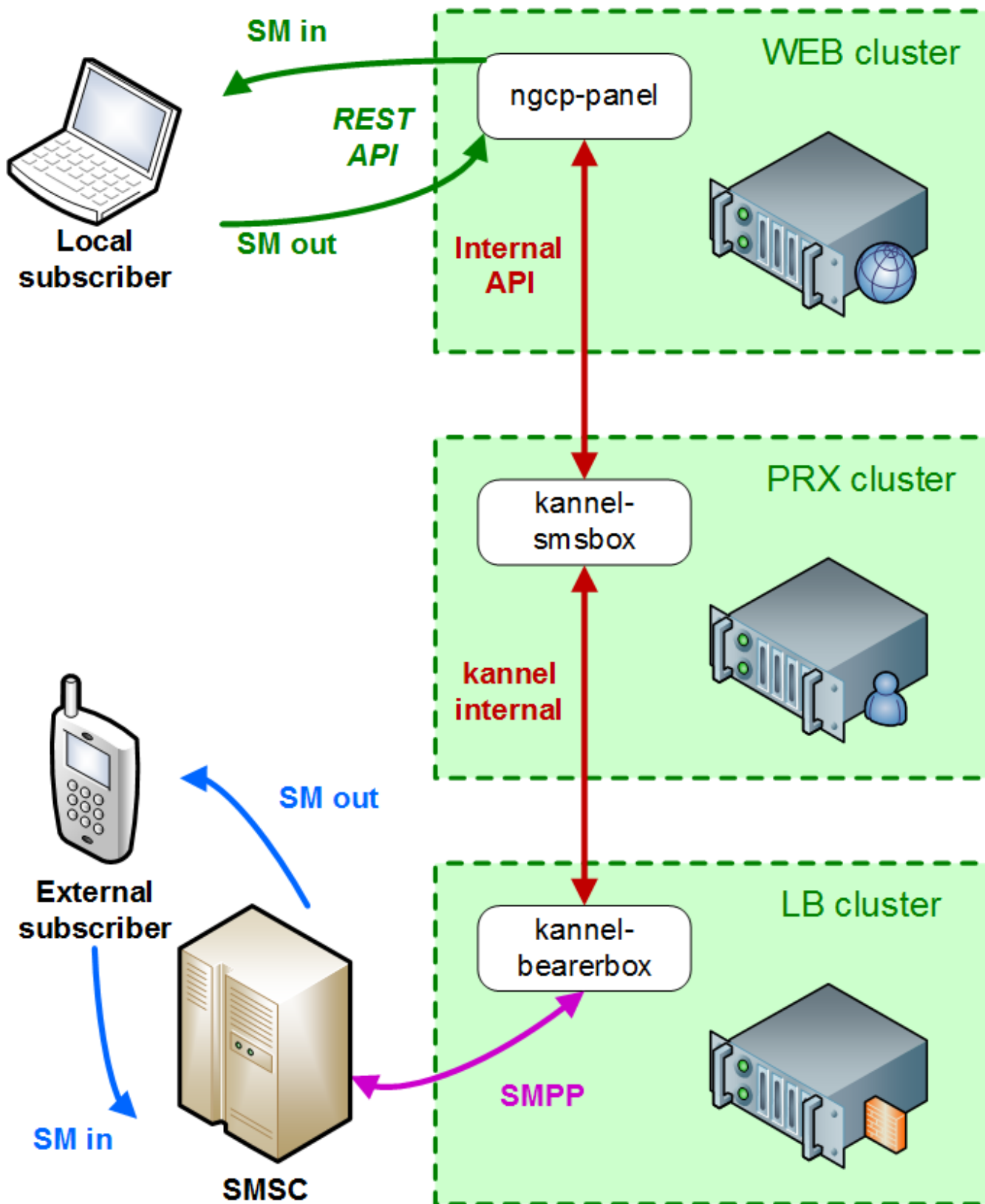
Figure 178. SMS Interaction
