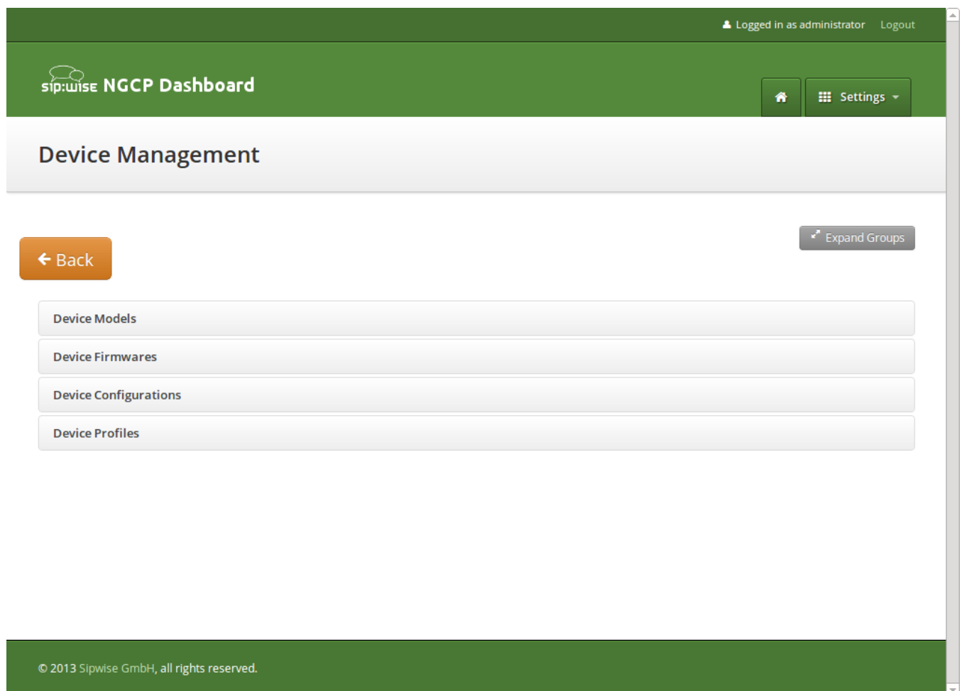
Figure 155. Device Management
