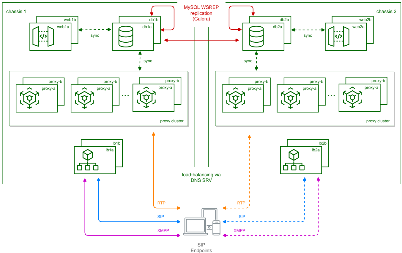
Figure 12. Scaling beyond one chassis
