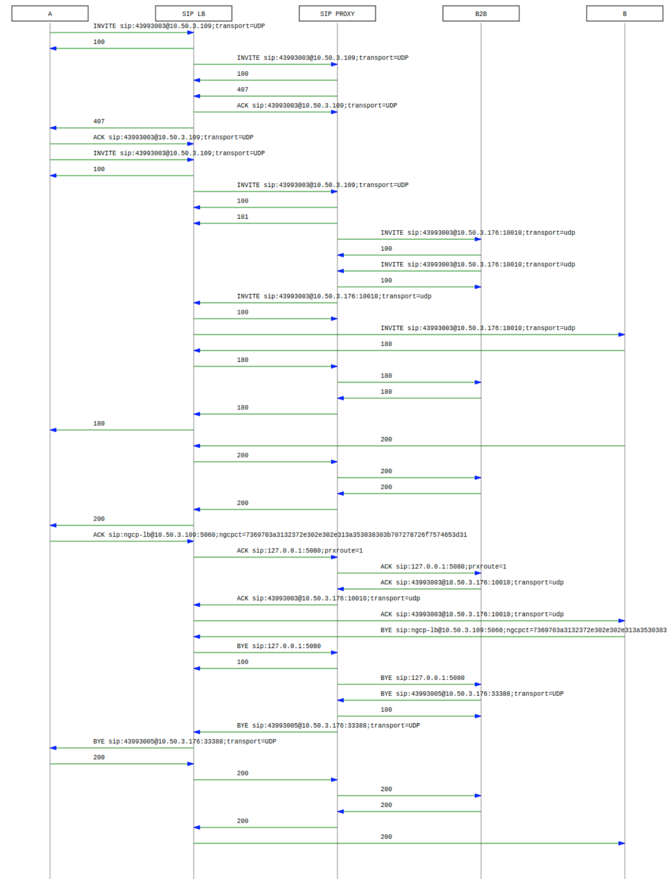
Figure 178: Basic Call Call-Flow
