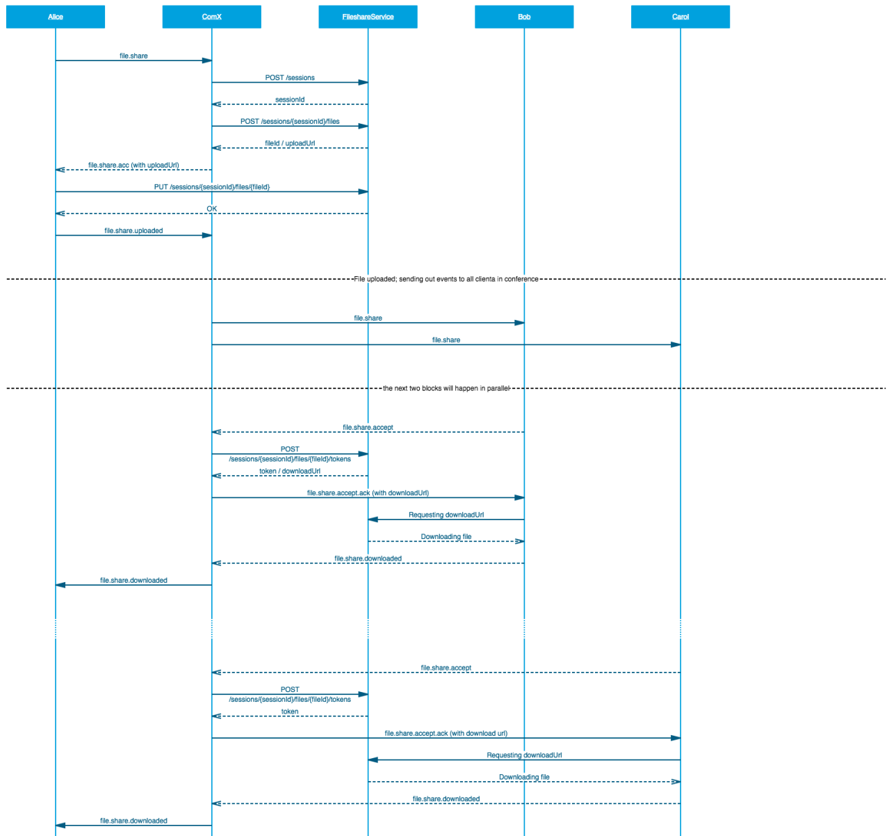
Figure 193: Sequence Detailed
