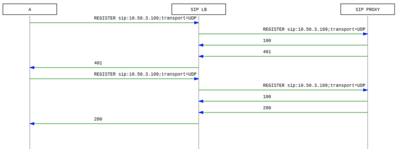
Figure 73: Registration Call-Flow
