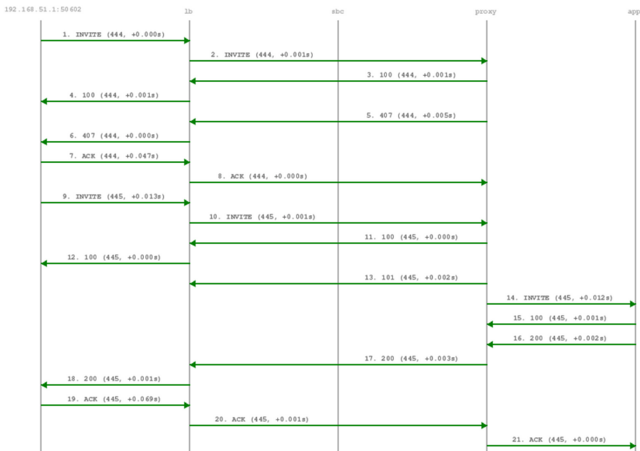
Figure 76: Voicebox Call-Flow
