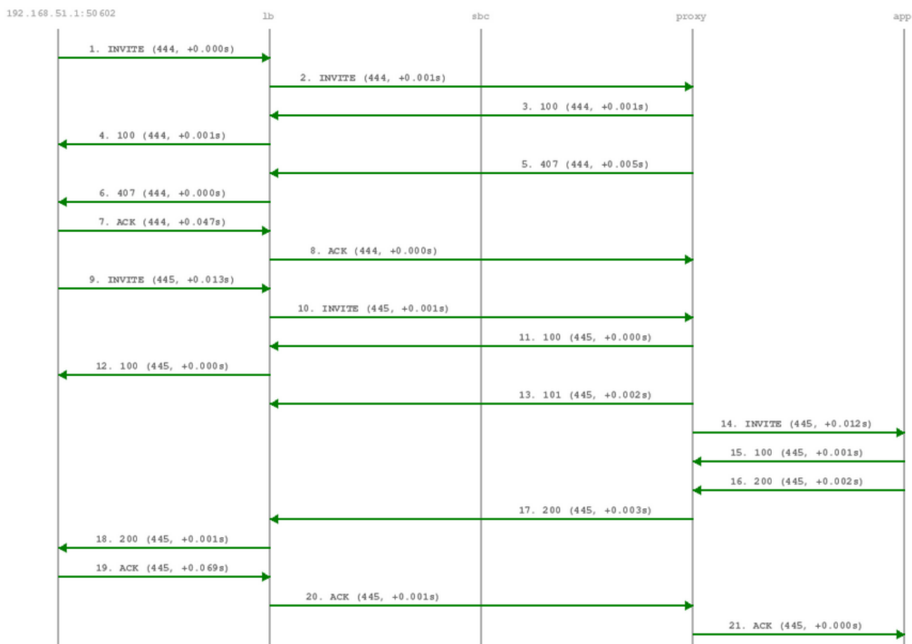
Figure 76: Voicebox Call-Flow
