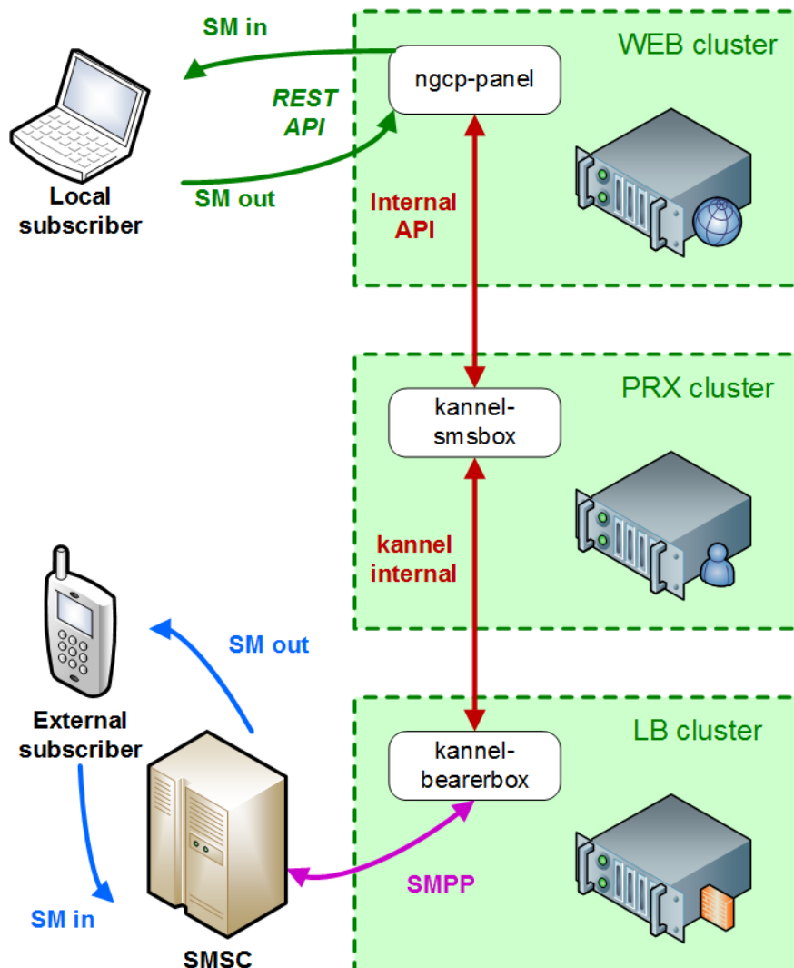
Figure 68: SMS Interaction
