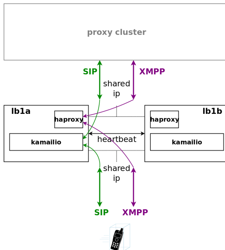
Figure 8: Load Balancer Overview
