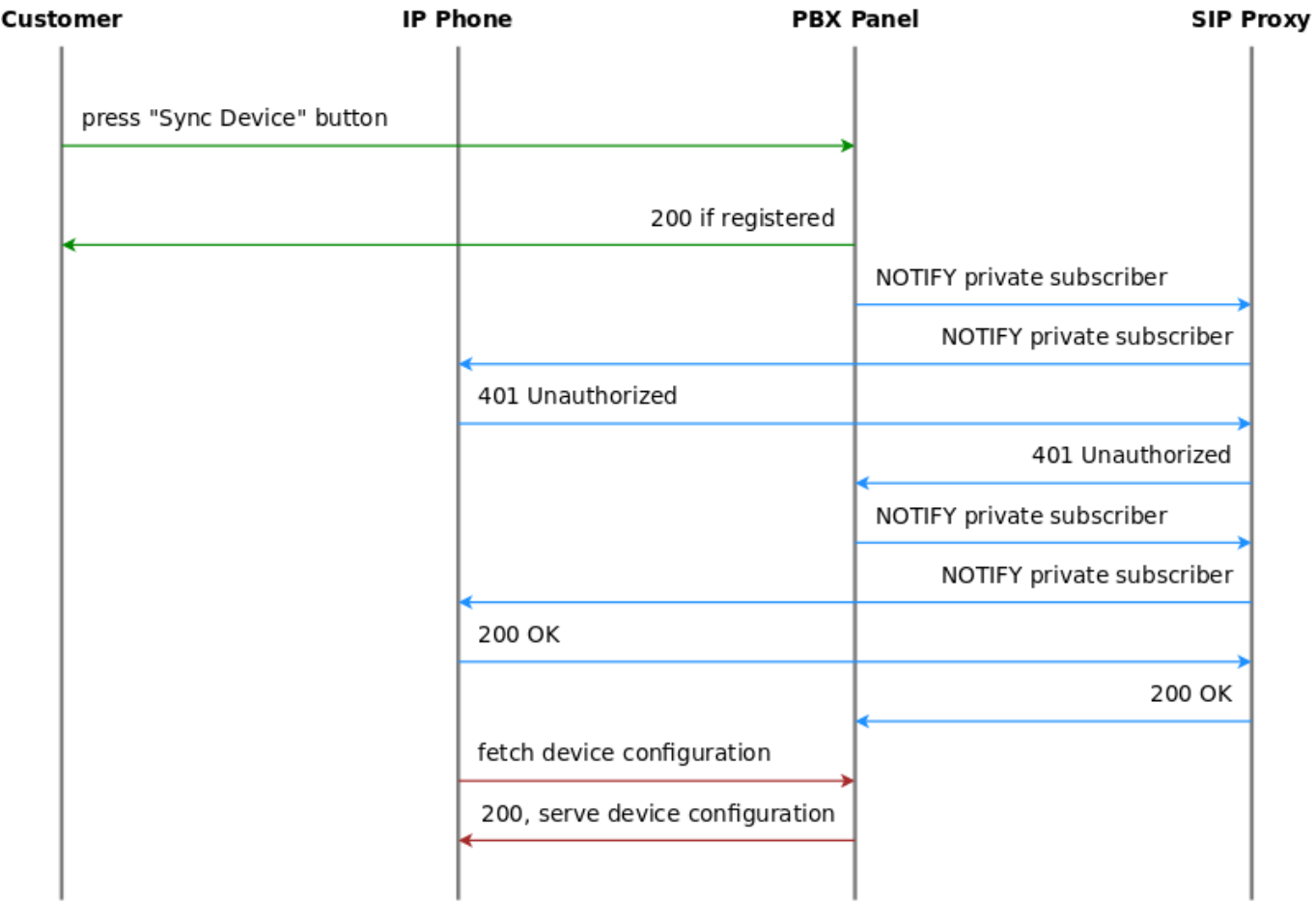
Figure 144: Resync a registered PBX device
