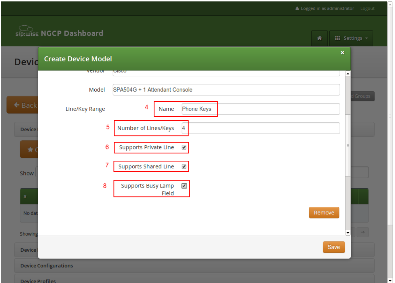
Figure 170: Create Device Model Part 2
