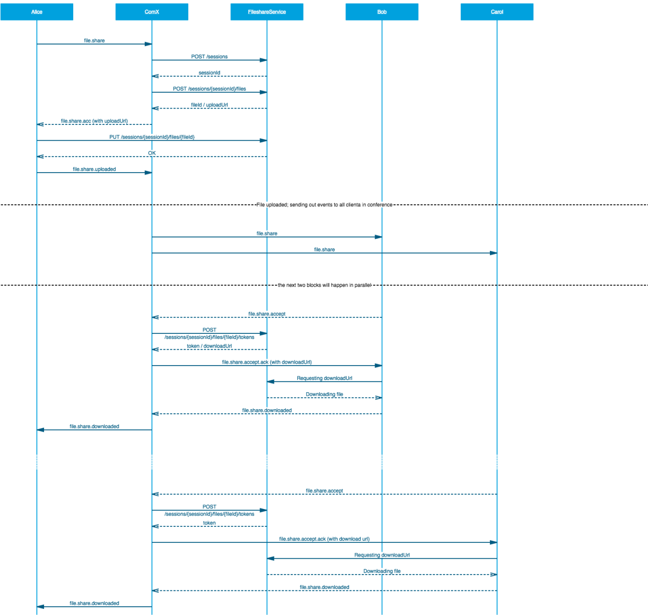
Figure 180: Sequence Detailed
