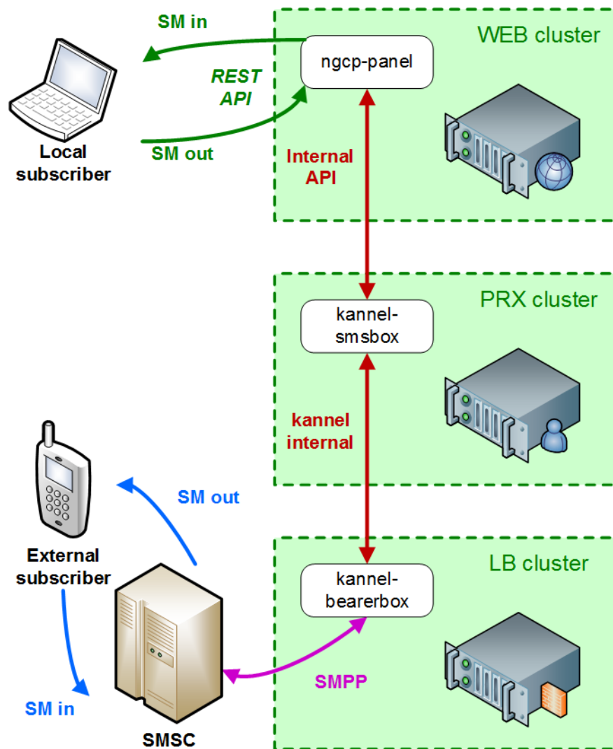
Figure 66: SMS Interaction
