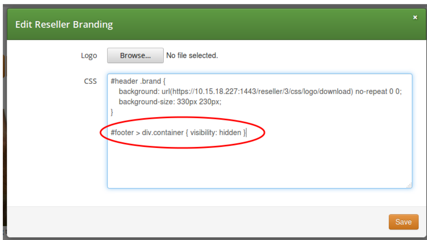
Figure 67: CSC Customisation: Hide copyright notice
