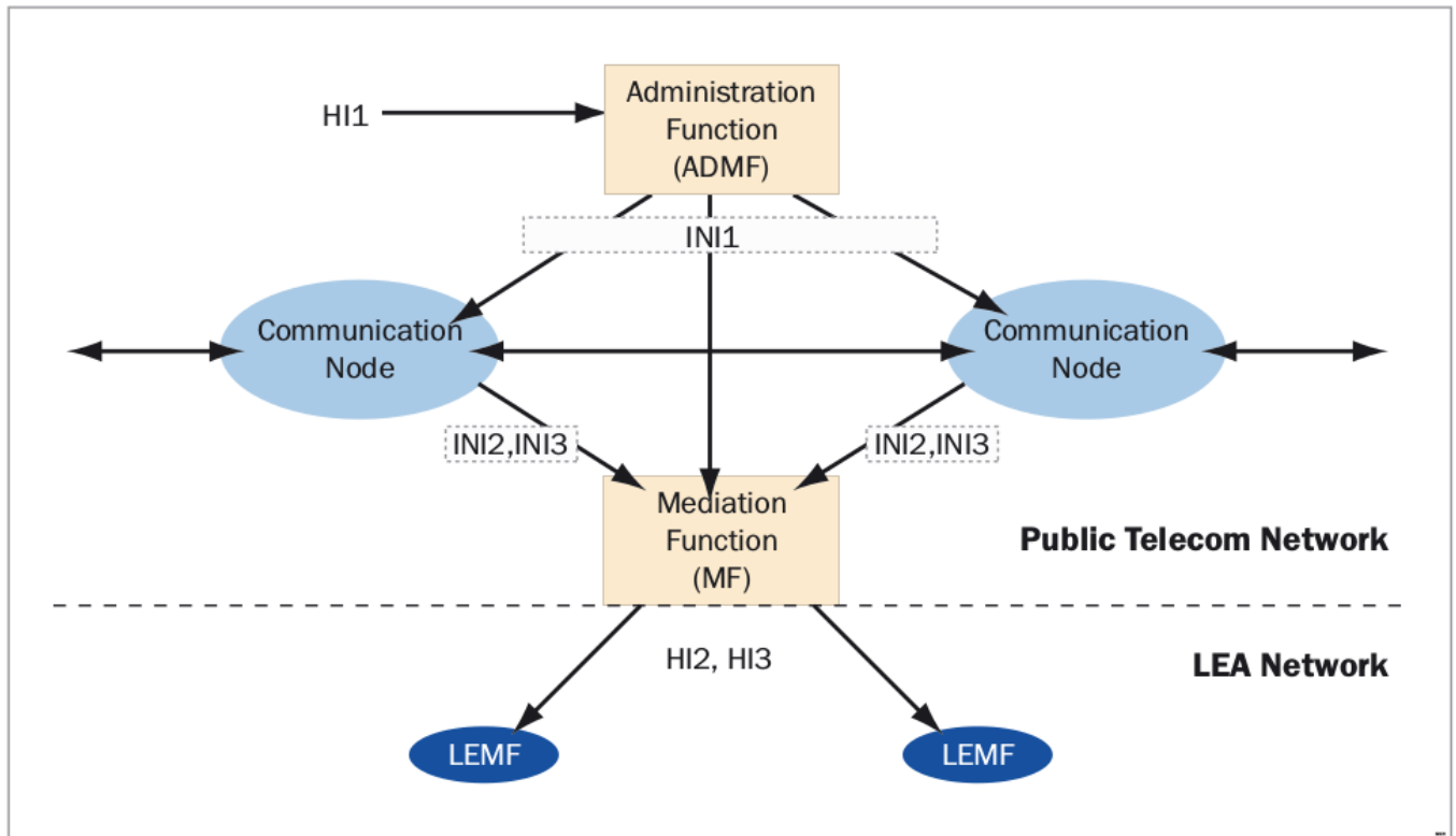
Figure 138: LI: ETSI Interfaces
