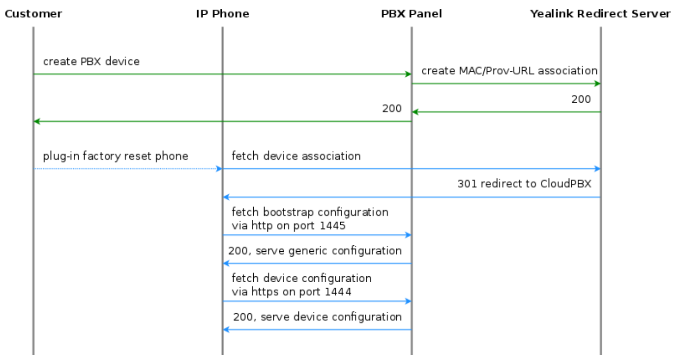
Figure 133: Initially bootstrap a Yealink phone
