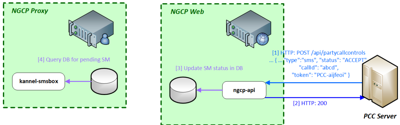
Figure 149: Short Message Accepted by PCC
