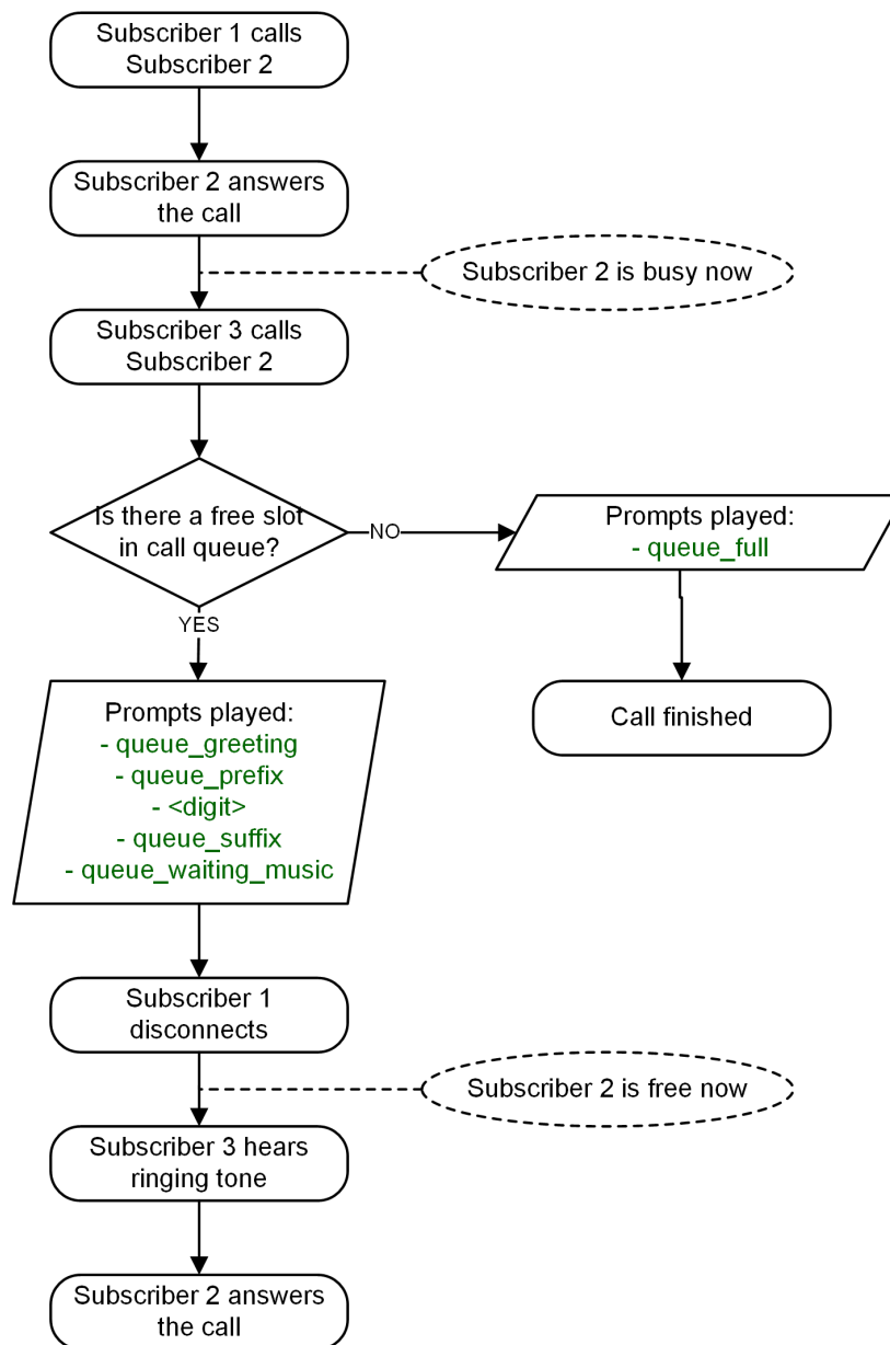
Figure 129: Flowchart of Call Queue
