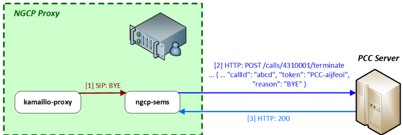
Figure 145: Call Termination with PCC
