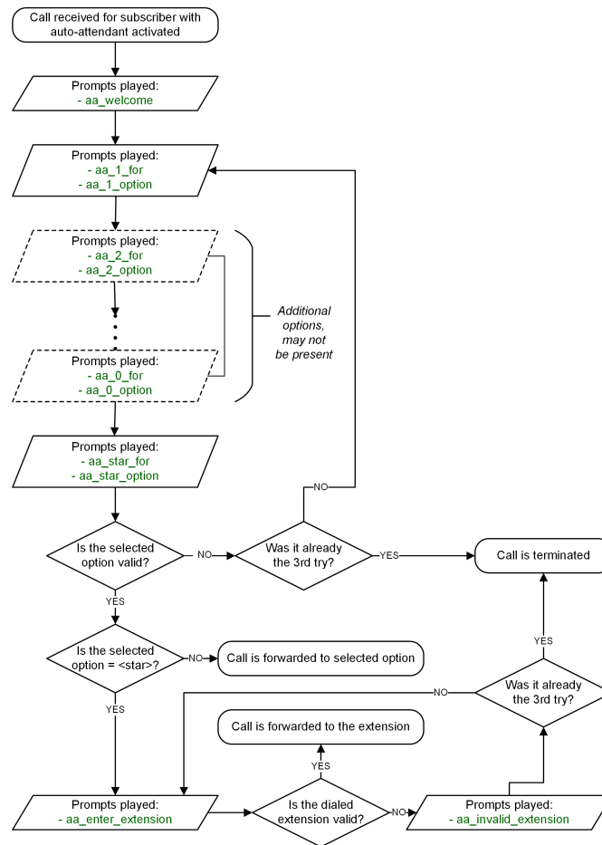
Figure 125: Flowchart of Auto-Attendant
