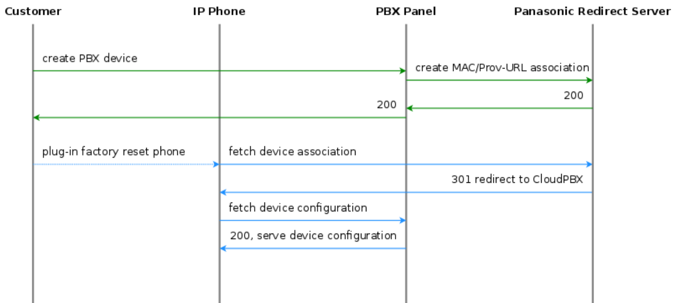
Figure 132: Initially bootstrap a Panasonic phone
