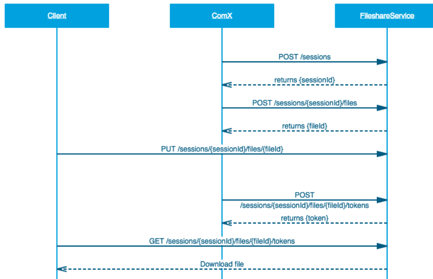
Figure 159: Sequence Simple
