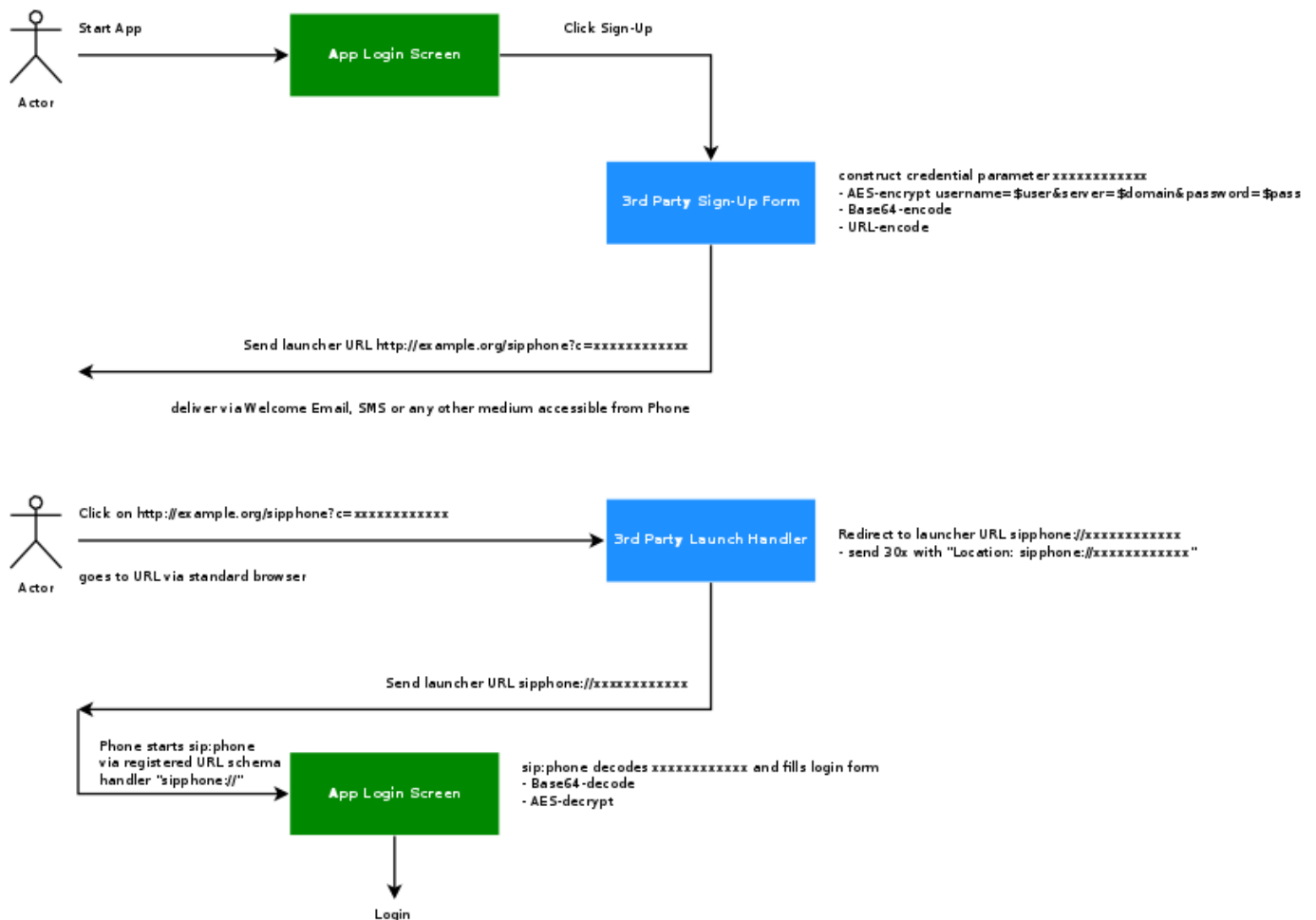
Figure 135: Provisioning Push Workflow
