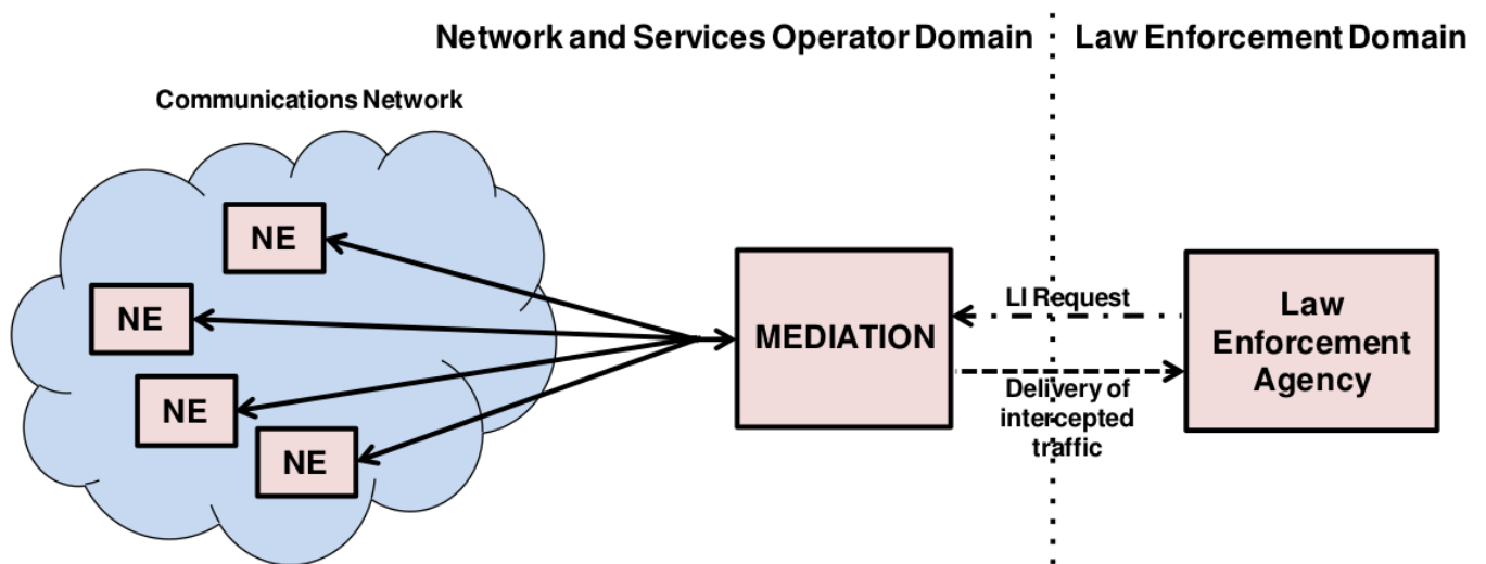
Figure 137: LI: High Level Overview
