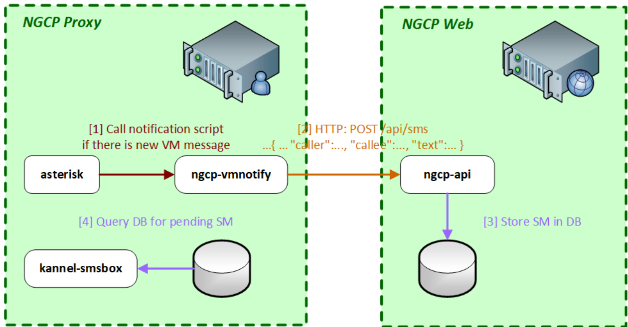
Figure 147: Voicemail Notification with SMS
