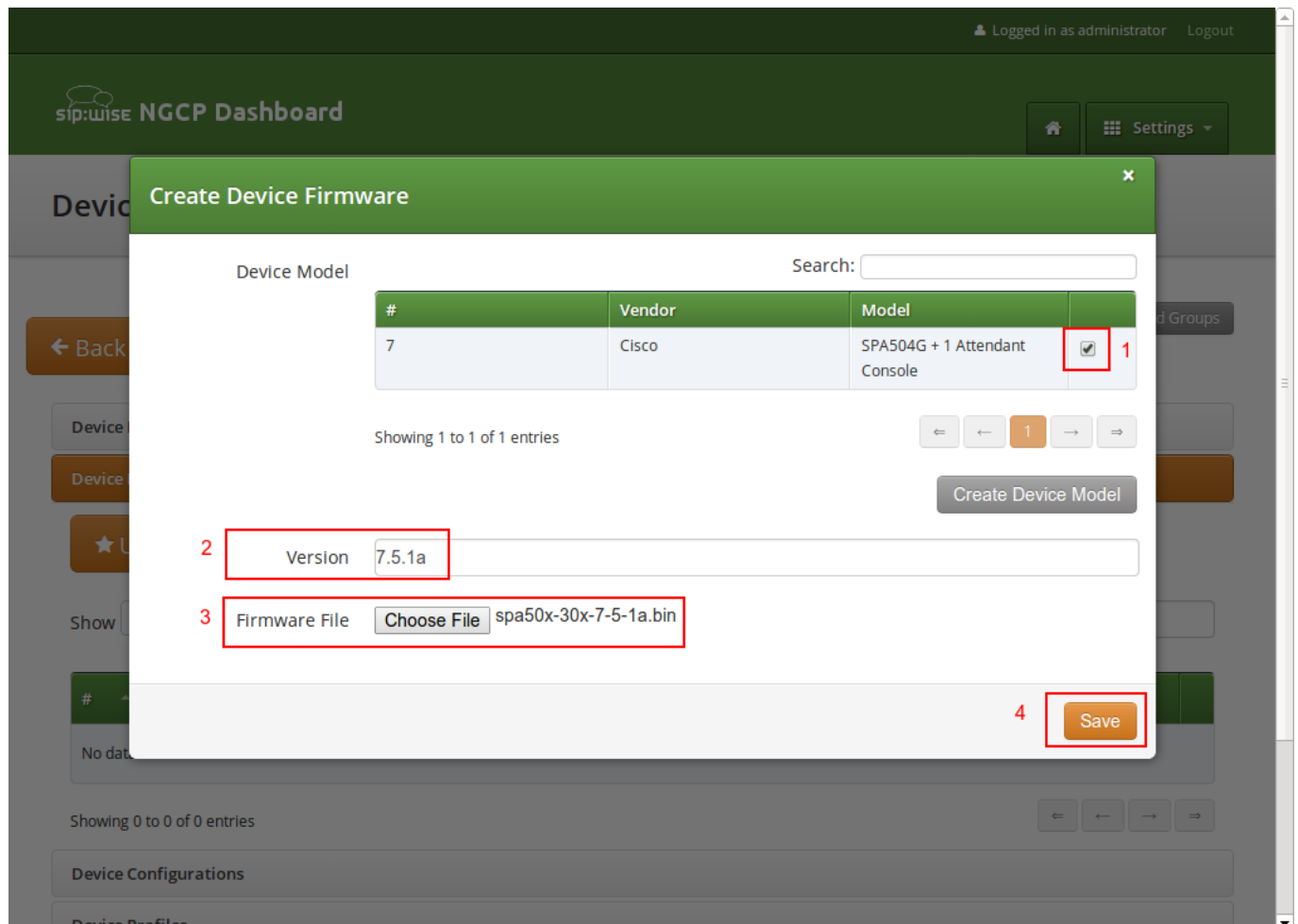
Figure 94: Upload Device Firmware
