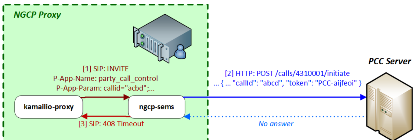
Figure 143: Call Initiation Timeout with PCC
