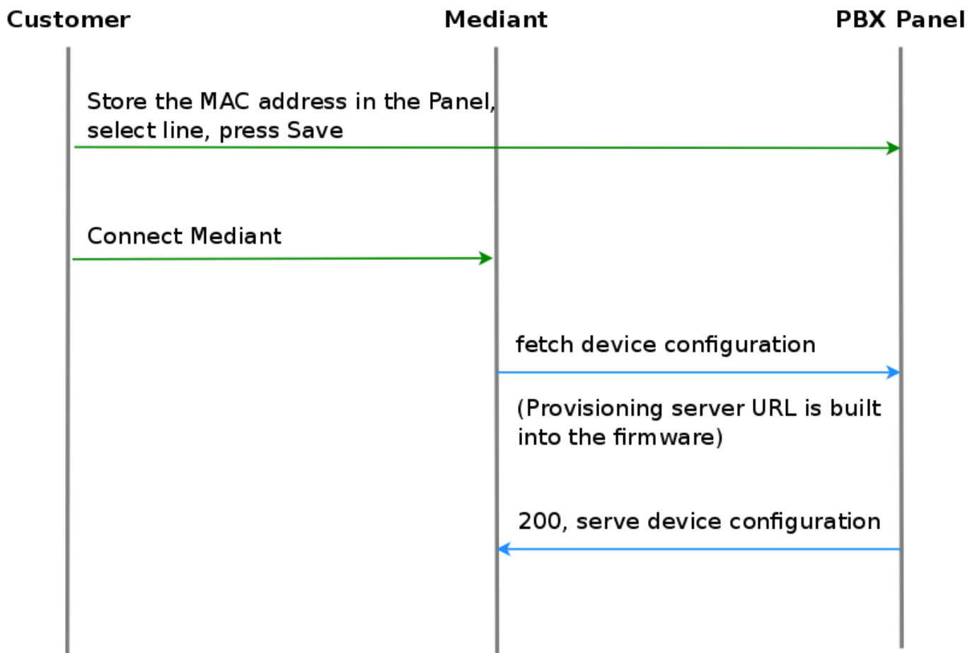
Figure 134: Initially bootstrap a Mediant gateway
