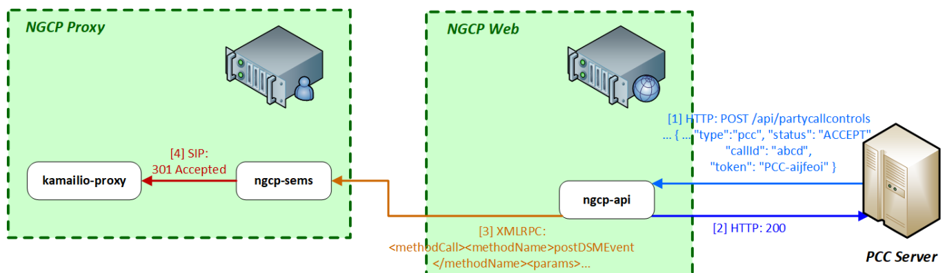
Figure 144: Call Accepted by PCC
