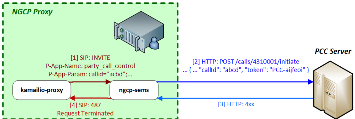
Figure 142: Call Initiation Error with PCC
