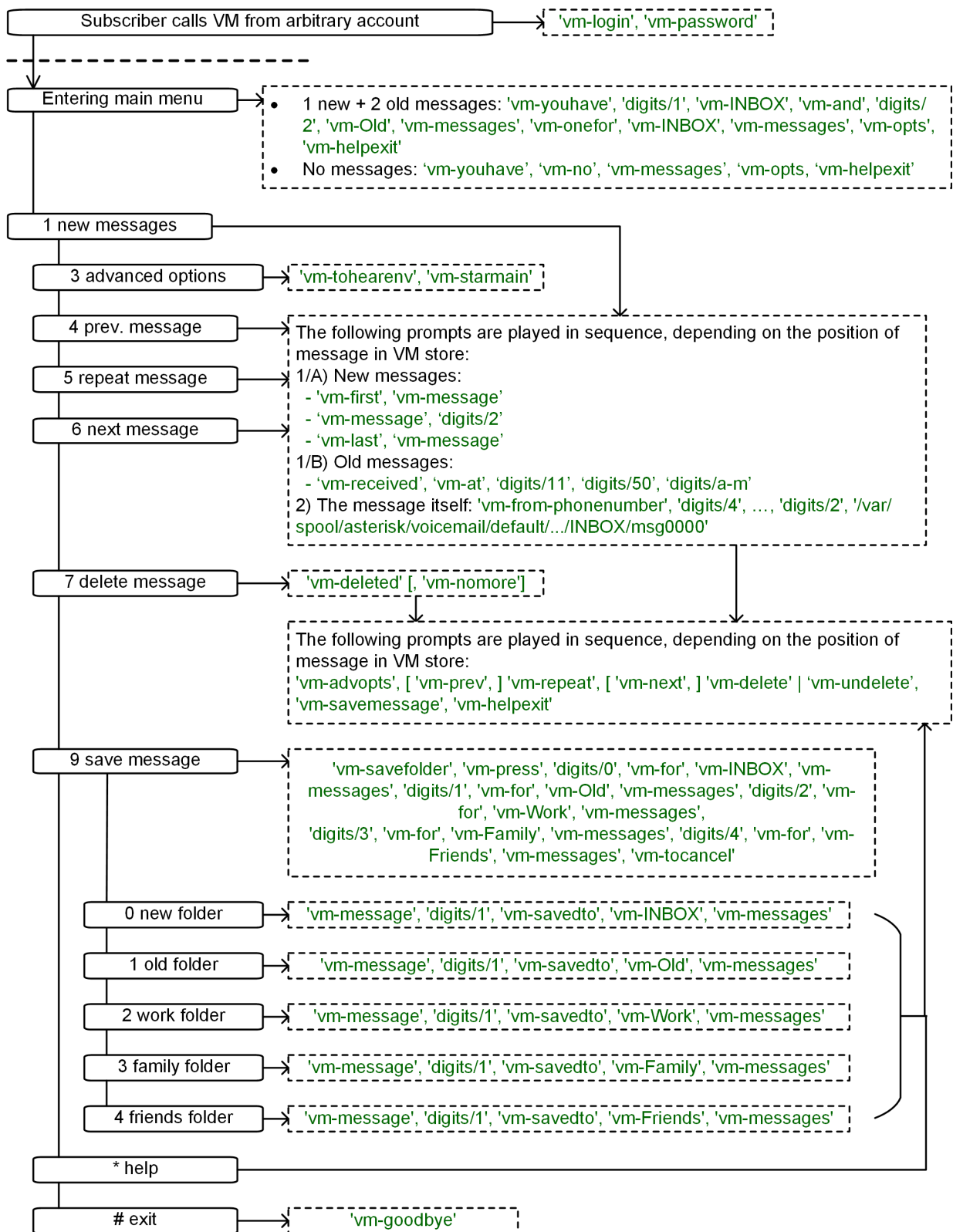
Figure 41: Flowchart of Listening to New Messages
