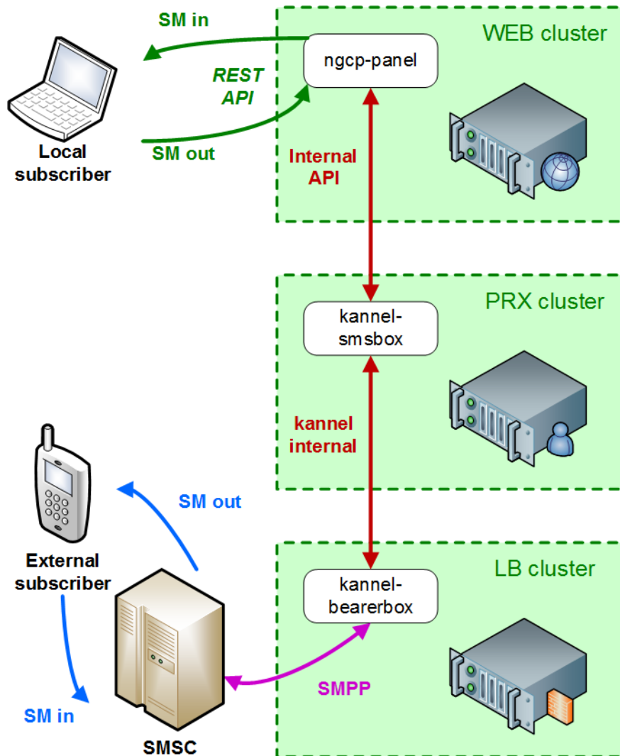
Figure 52: SMS Interactions on NGCP
