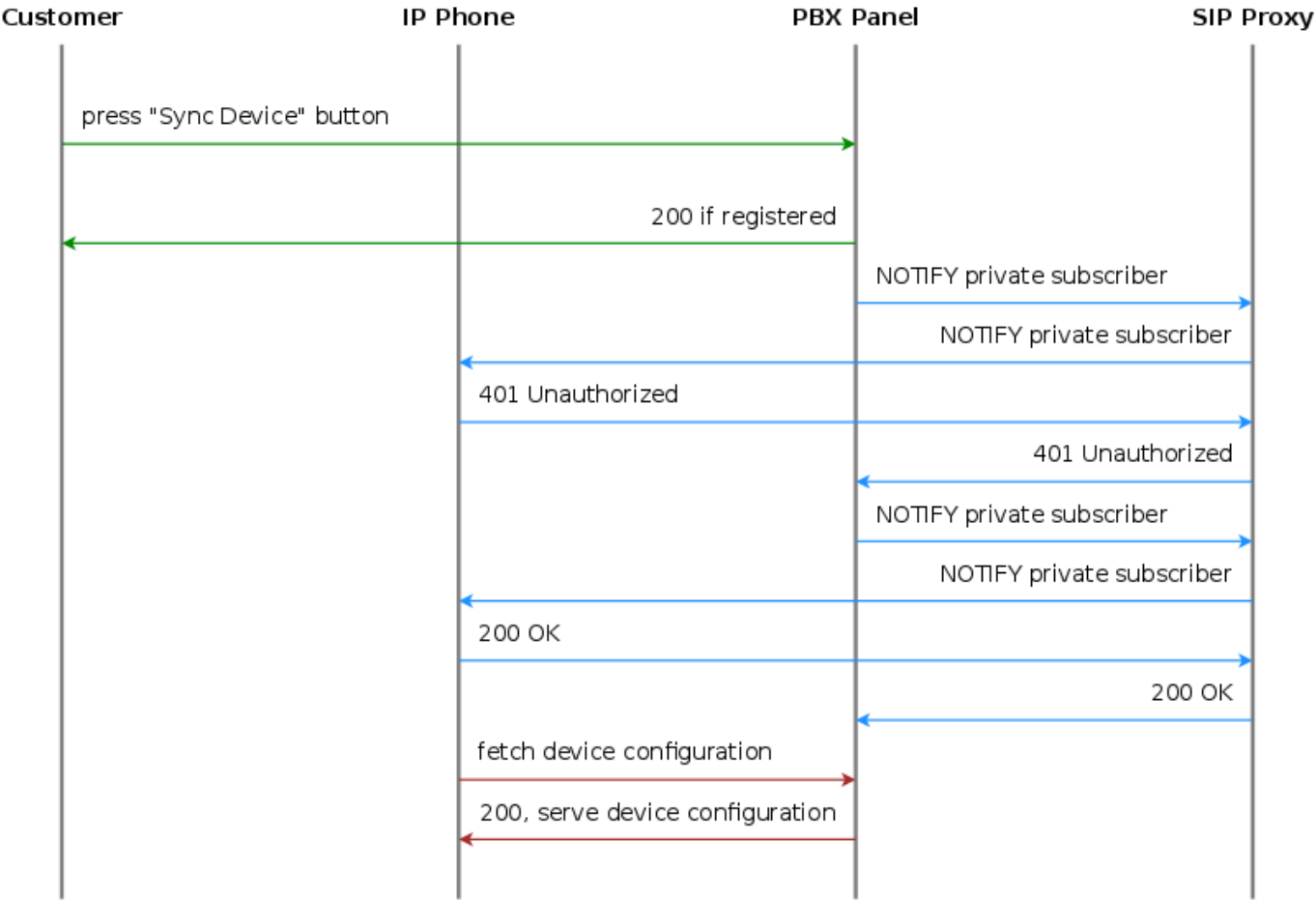
Figure 134: Resync a registered PBX device
