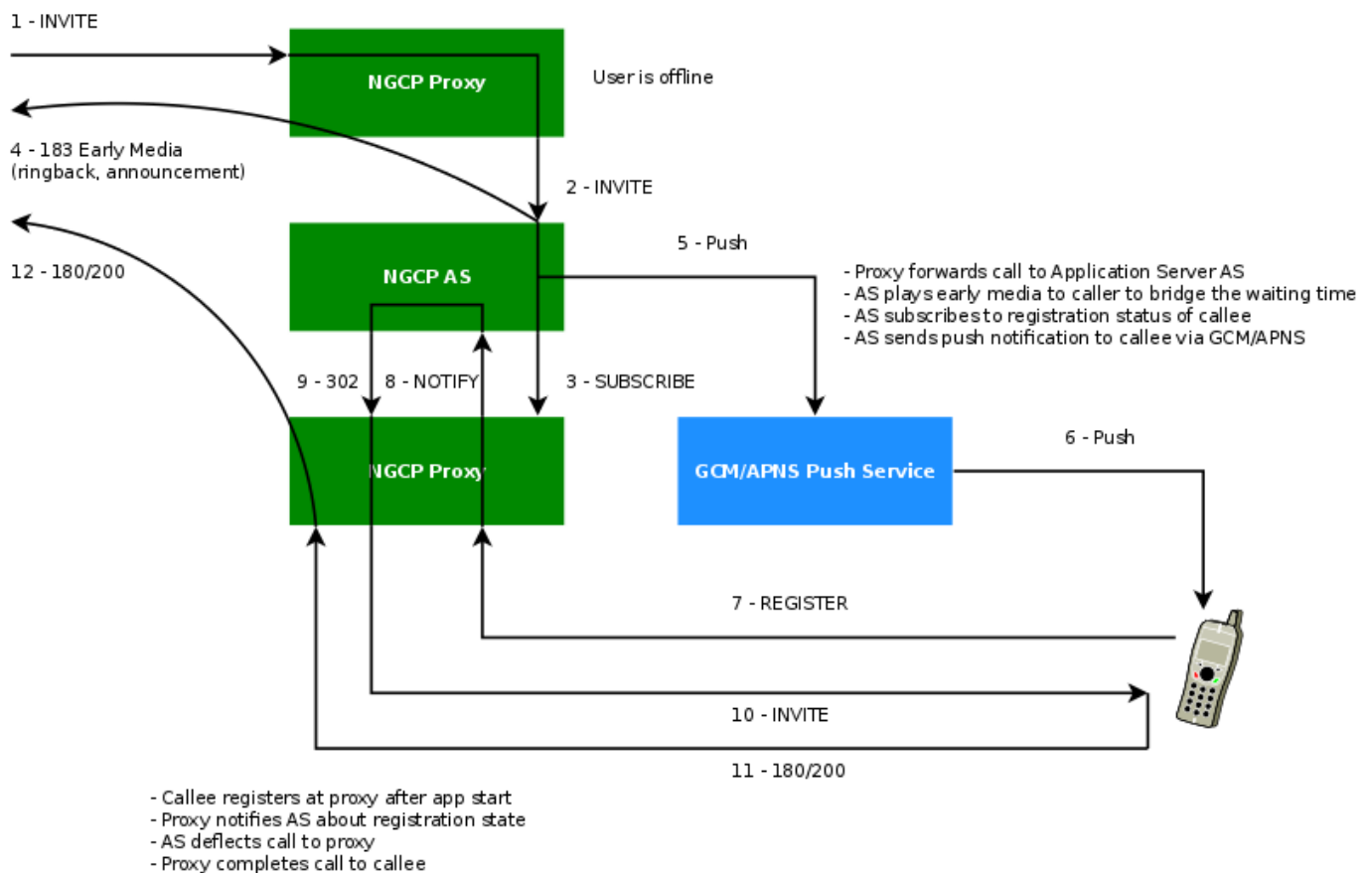
Figure 137: Mobile Push Workflow
