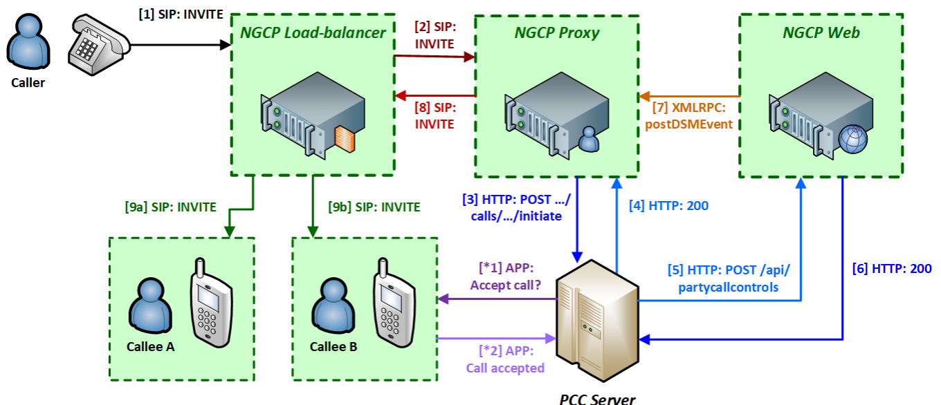
Figure 141: Overview of Party Call Control
