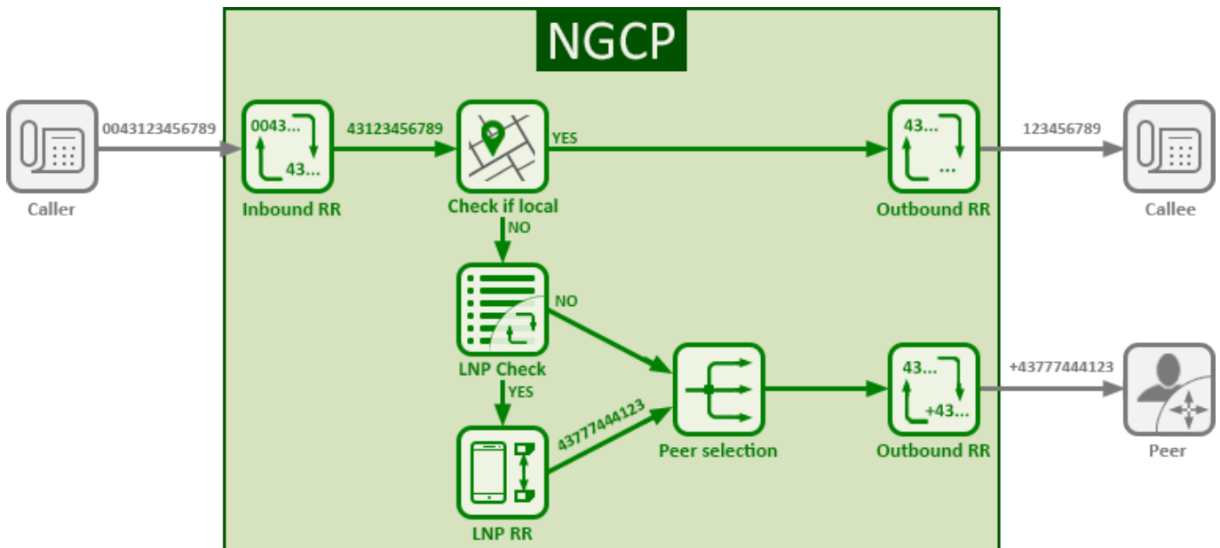
Figure 151: General Call Setup
