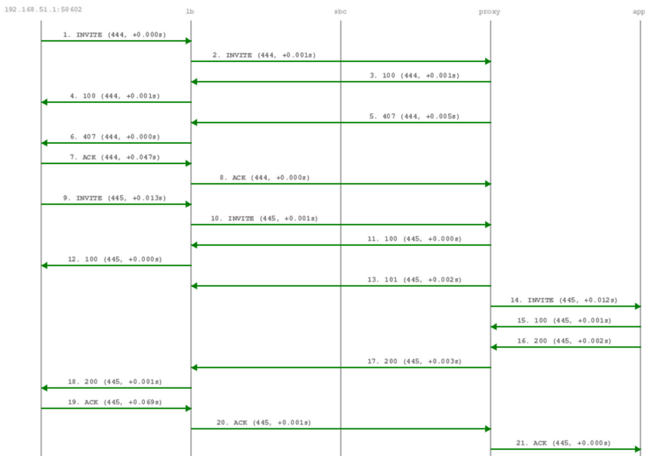
Figure 44: Voicebox Call-Flow
