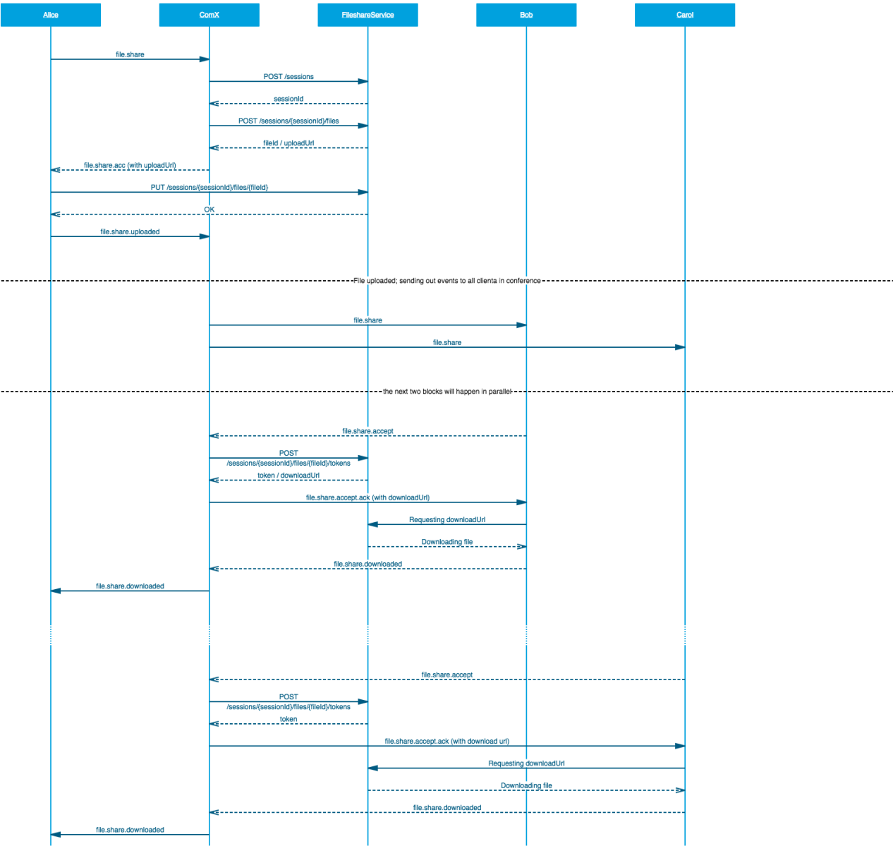
Figure 130: Sequence Detailed
