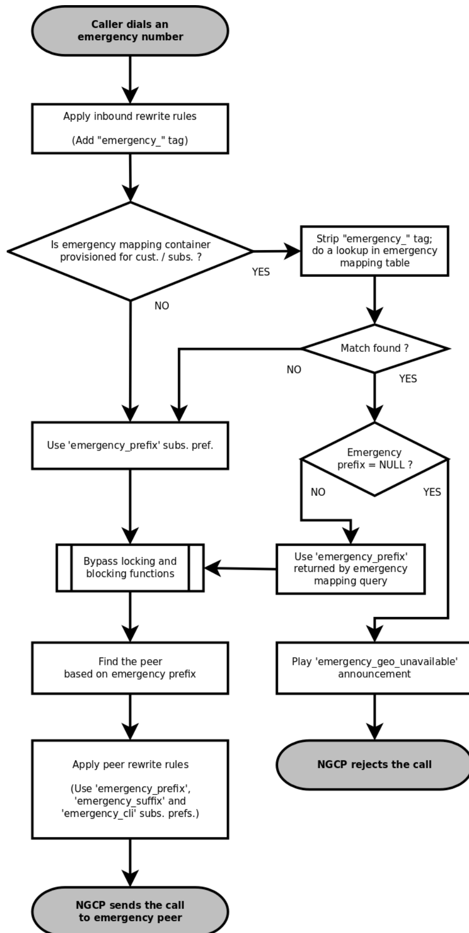
Figure 25: Emergency Call Handling with Mapping
