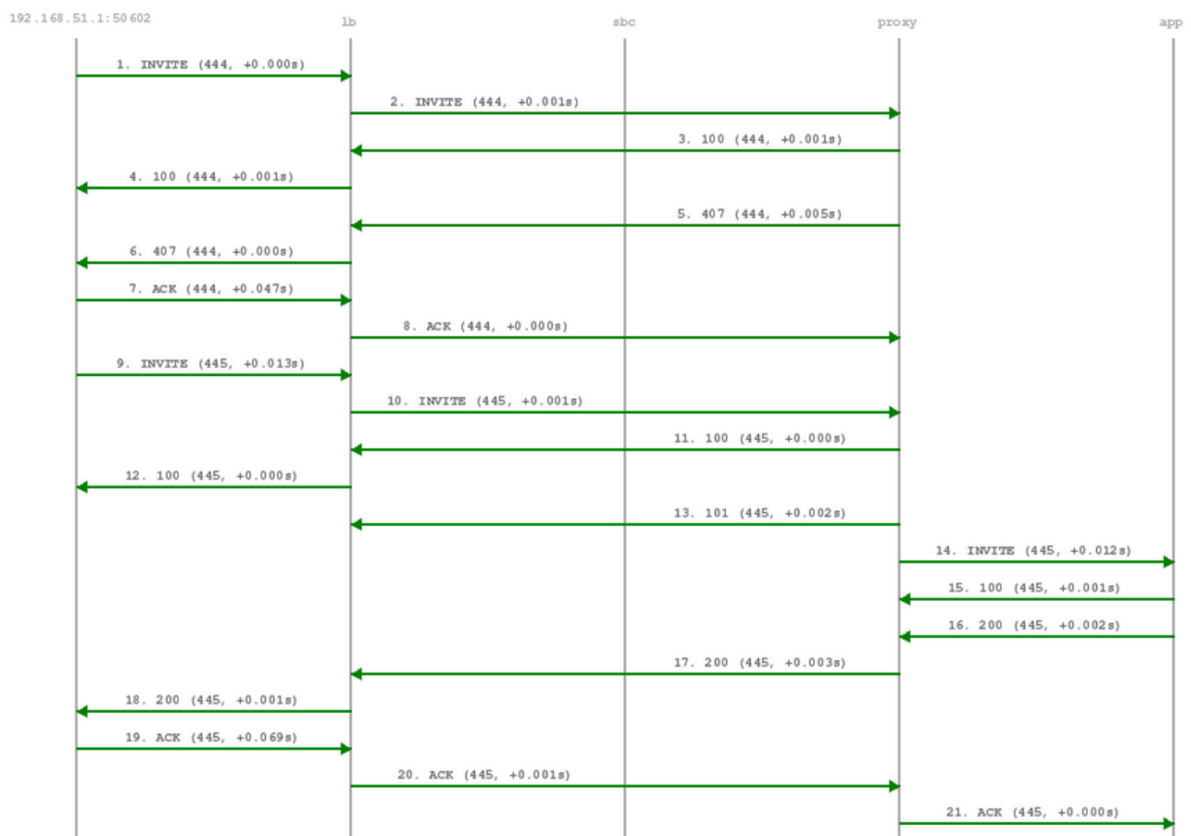
Figure 124: Voicebox Call-Flow
