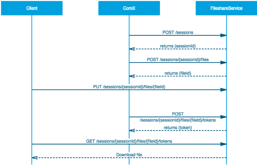
Figure 129: Sequence Simple
