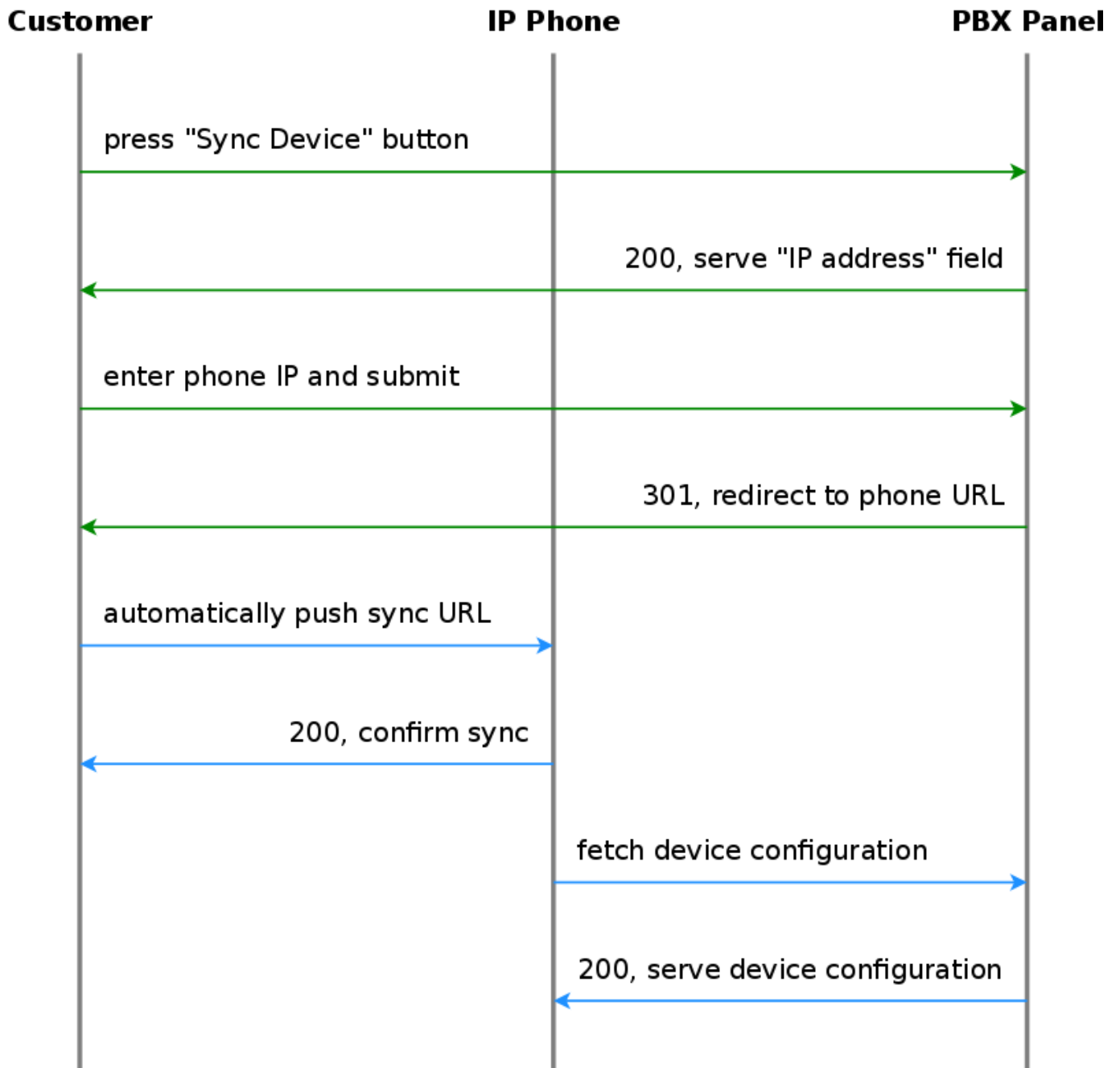
Figure 102: Initially bootstrap a PBX device
