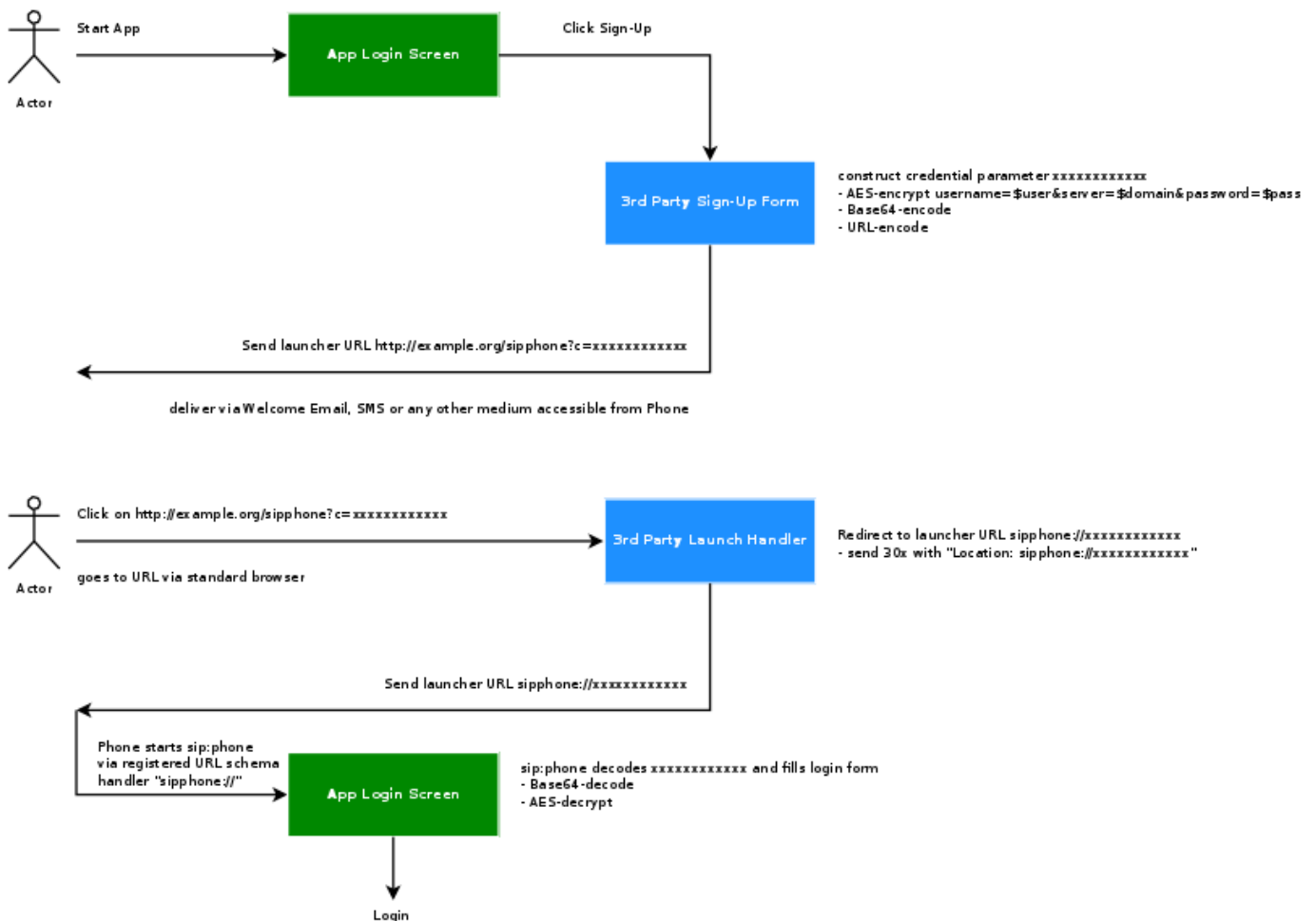
Figure 107: Provisioning Push Workflow
