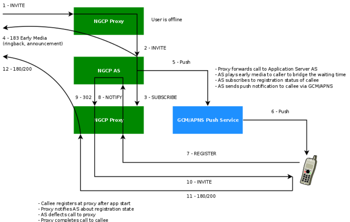
Figure 108: Mobile Push Workflow
