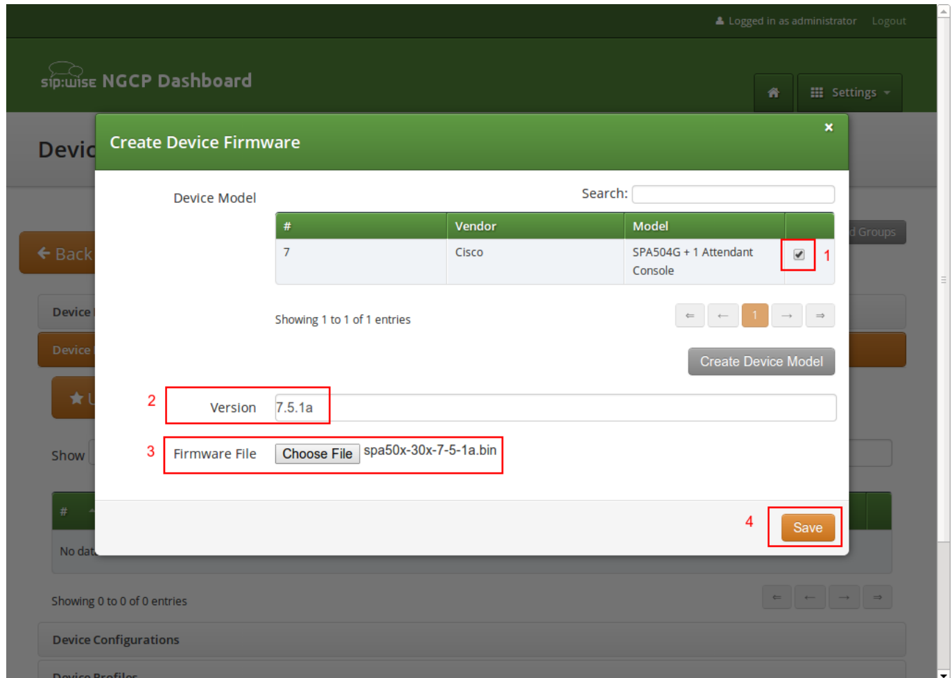
Figure 67: Upload Device Firmware
