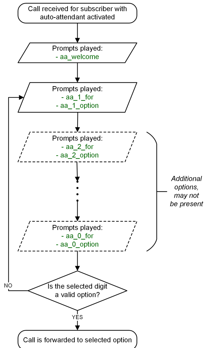
Figure 97: Flowchart of Auto Attendant
