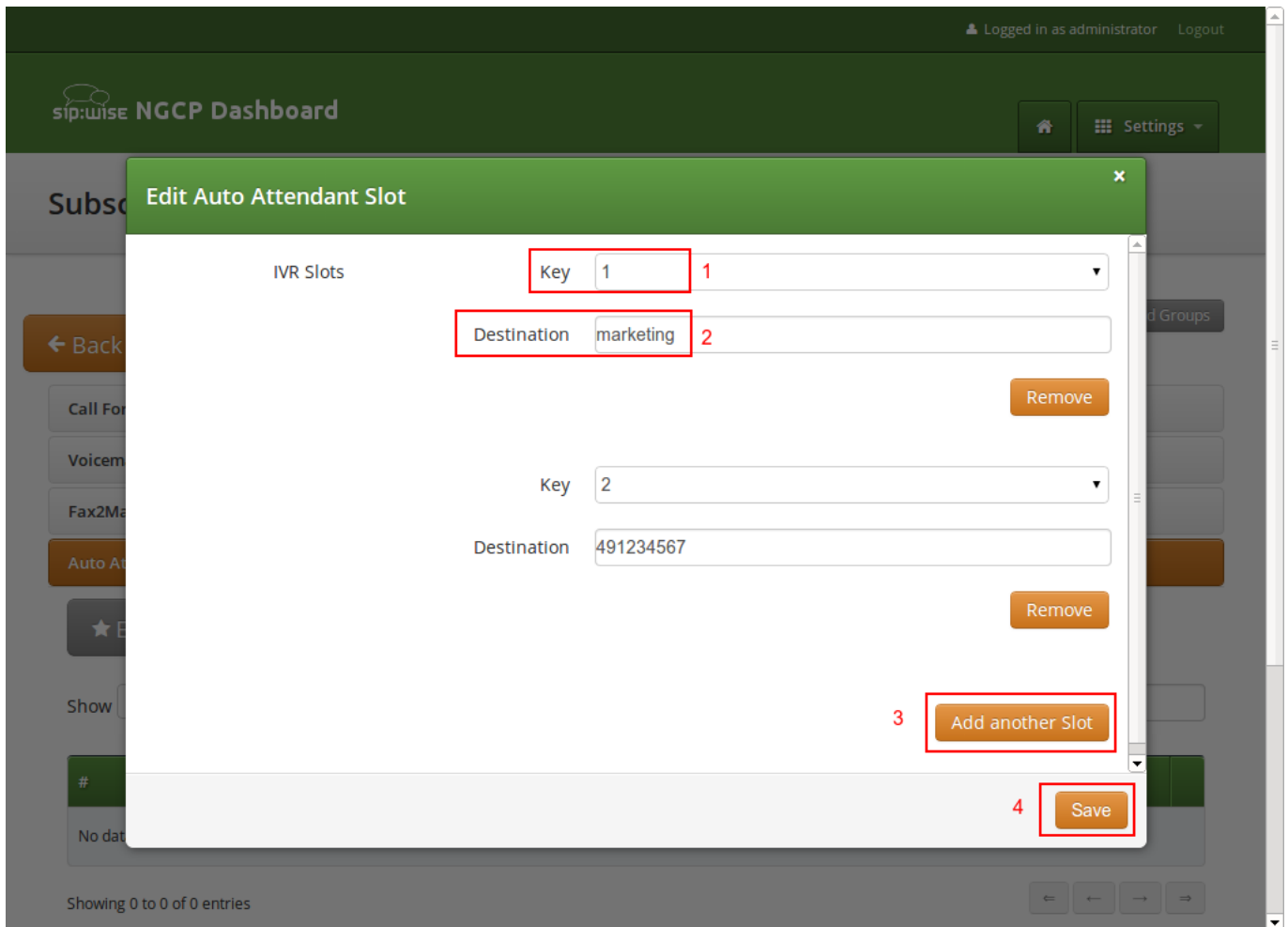
Figure 98: Define the Auto Attendant Slots
