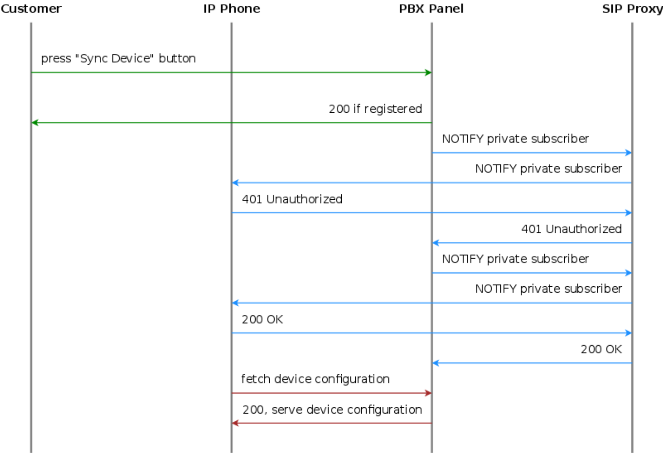
Figure 103: Resync a registered PBX device
