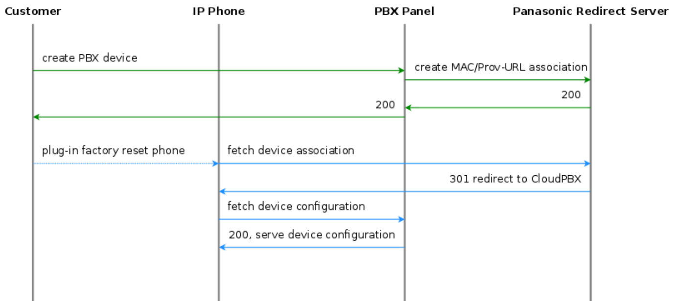
Figure 104: Initially bootstrap a Panasonic phone
