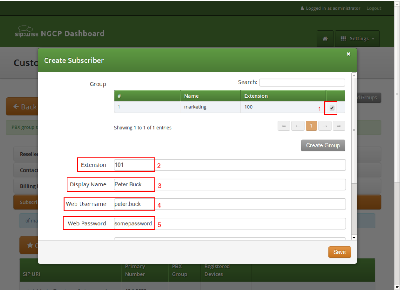
Figure 86: Finish PBX Subscriber Creation Part 1
