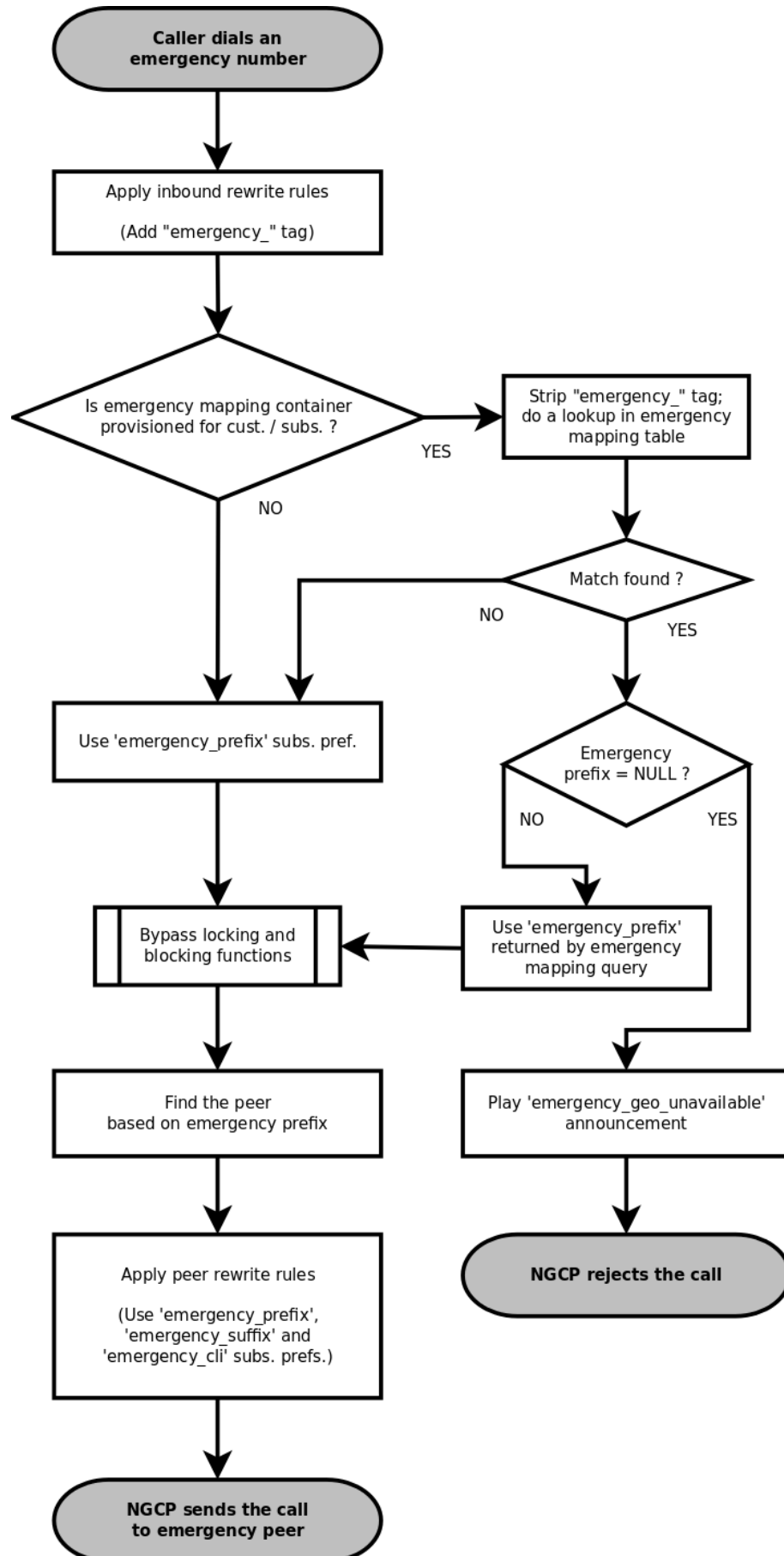
Figure 14: Emergency Call Handling with Mapping
