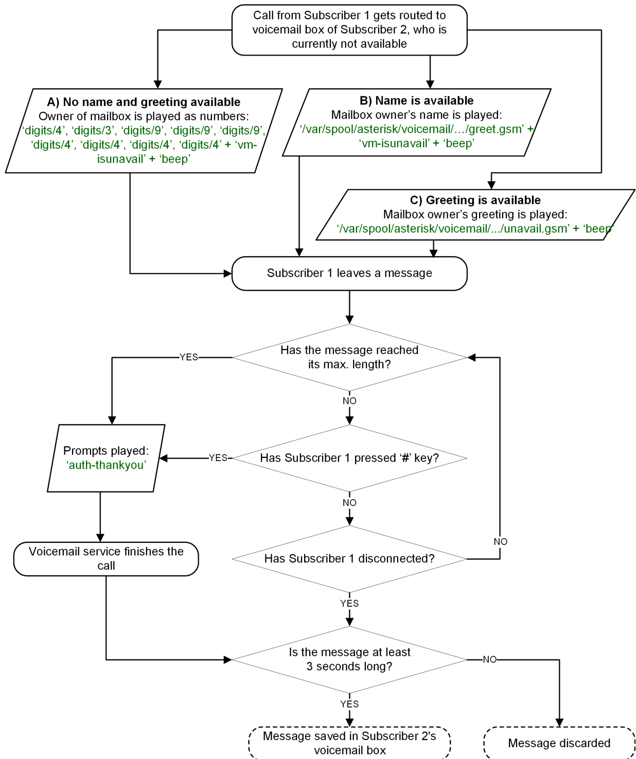
Figure 23: Flowchart of Leaving a Voice Message
