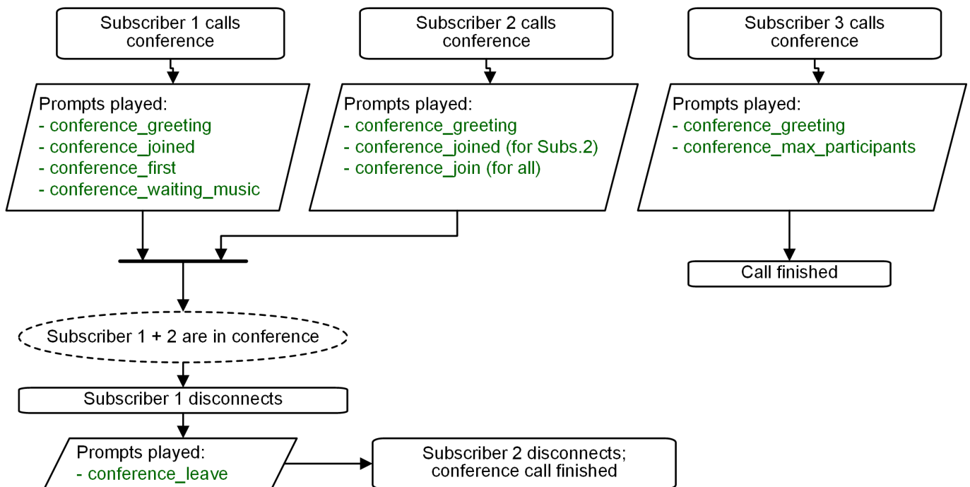
Figure 26: Flowchart of Conference without PIN
