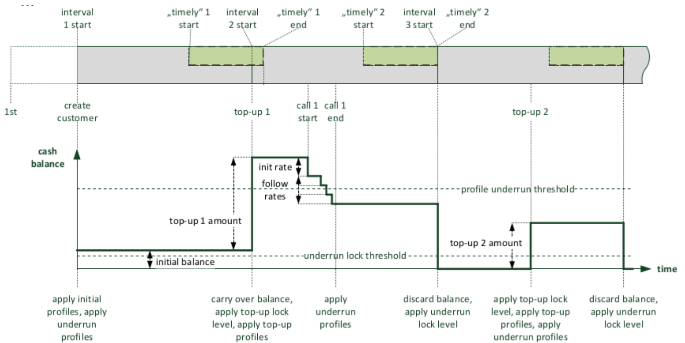
Figure 48: Example: Top-up Interval and Timely Carry-over
