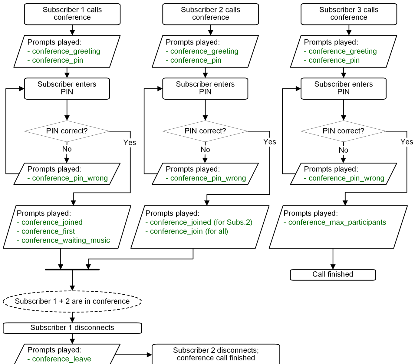
Figure 27: Flowchart of Conference with PIN Validation
