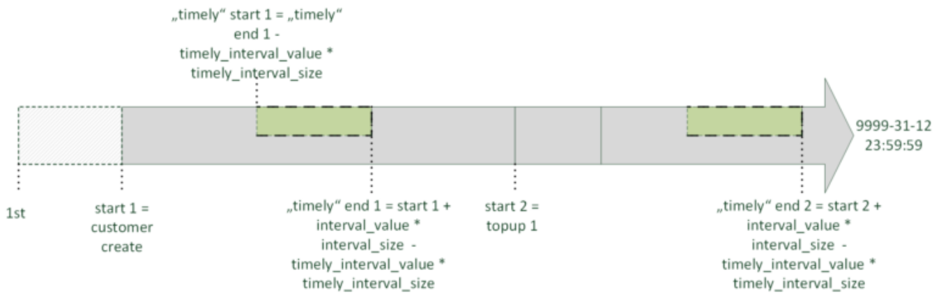
Figure 42: Interval Start Mode: topup
