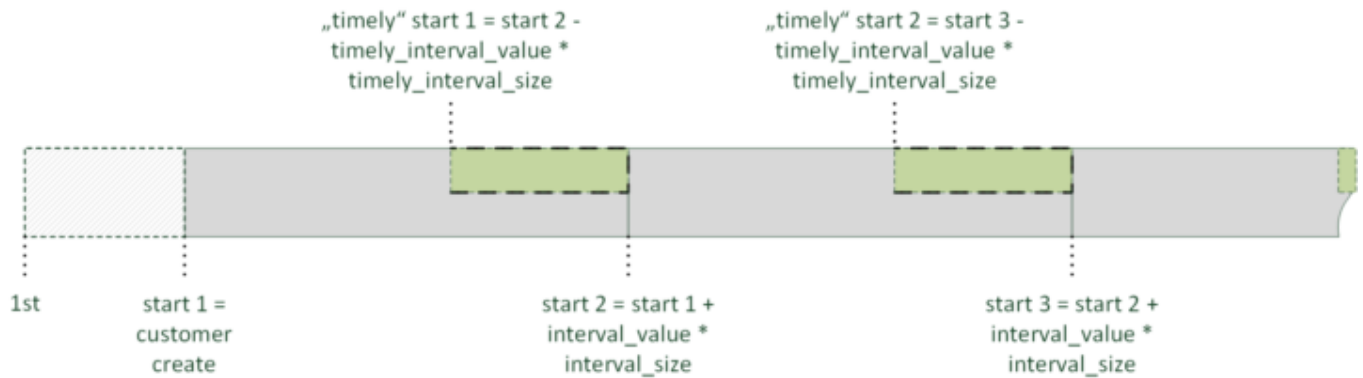
Figure 40: Interval Start Mode: create
