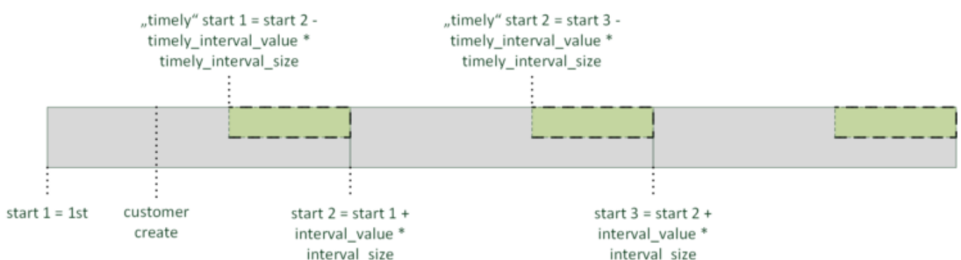
Figure 39: Interval Start Mode: 1st
