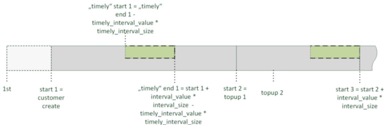
Figure 41: Interval Start Mode: topup_interval
