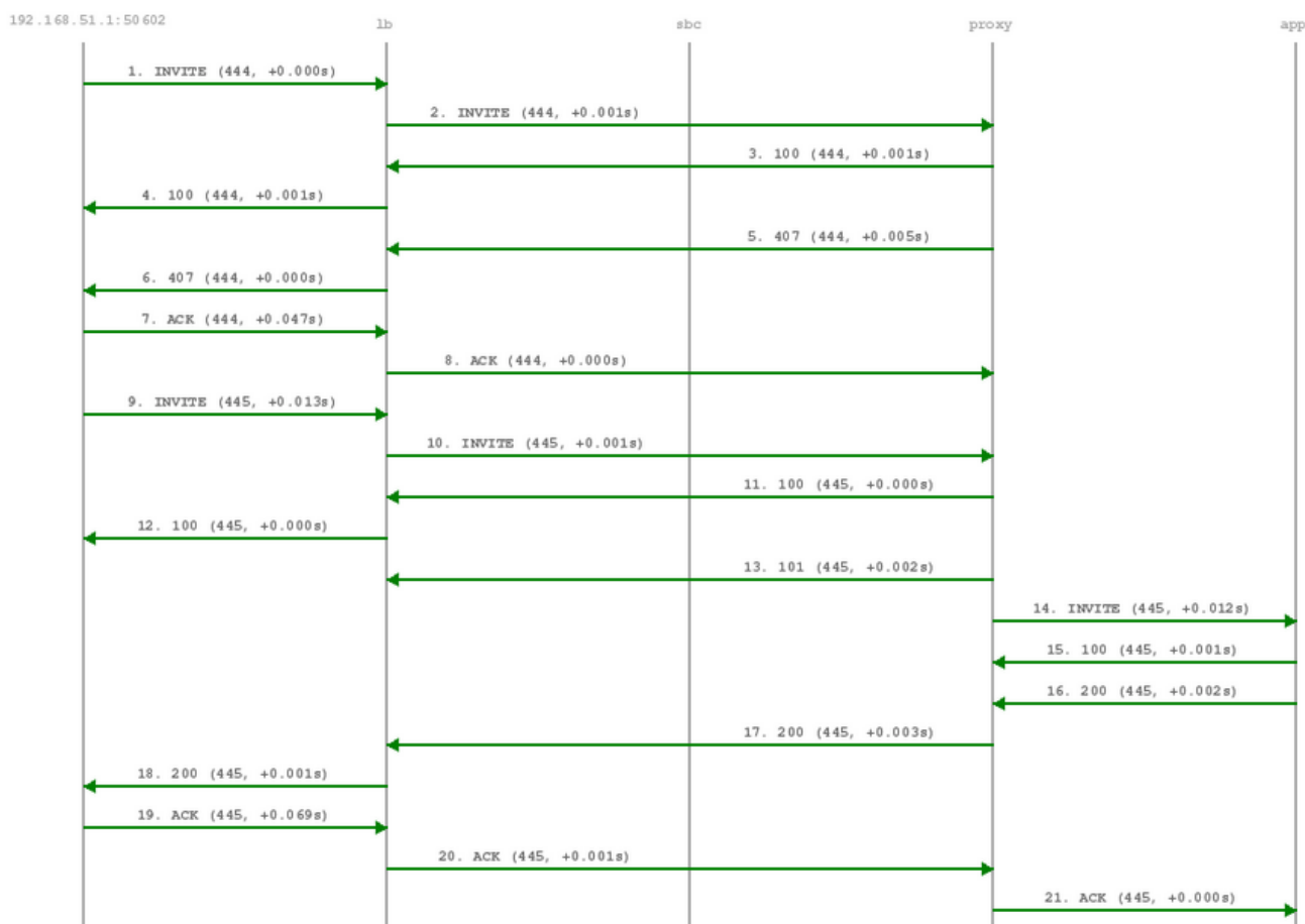
Figure 123: Voicebox Call-Flow
