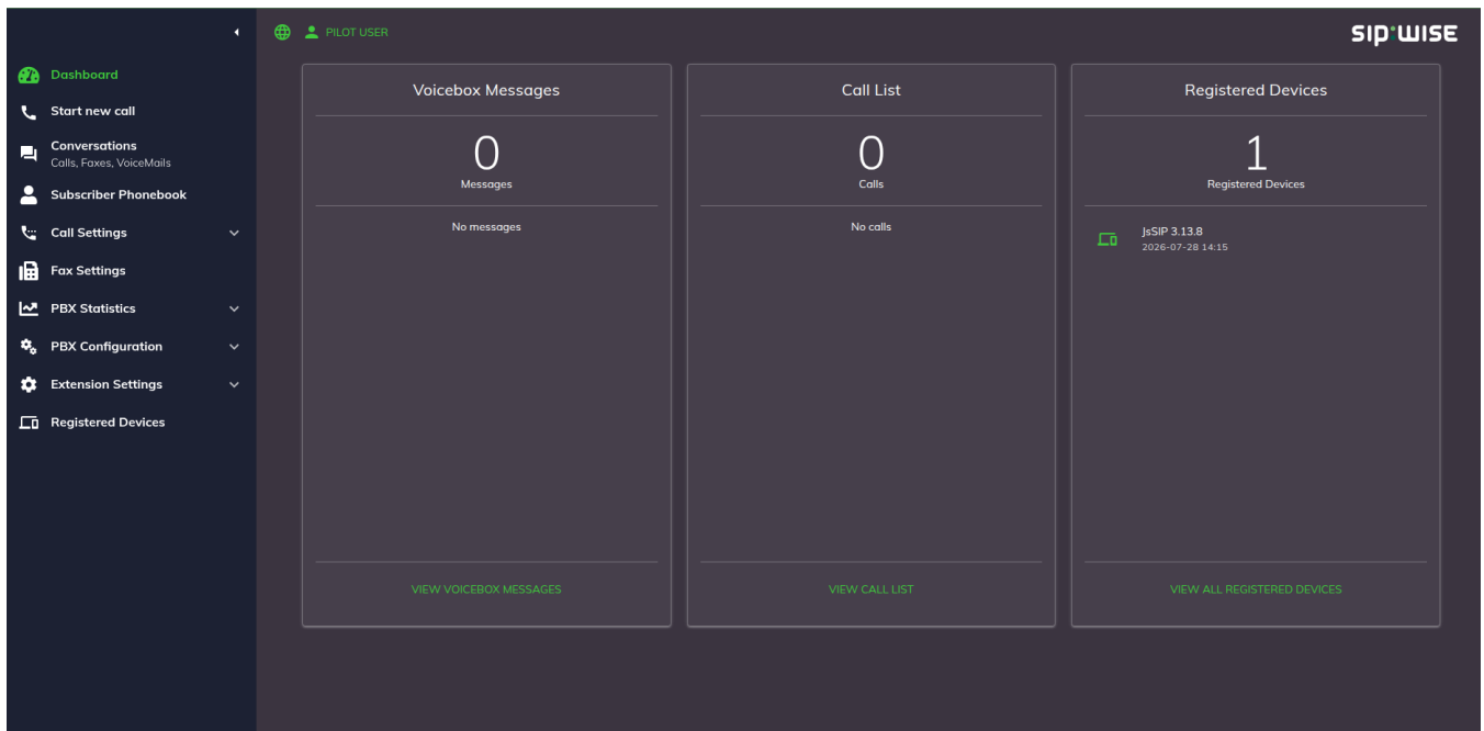
Figure 9. The Dashboard
