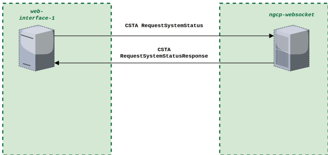
Figure 205. CSTA RequestSystemStatus messages exchange
