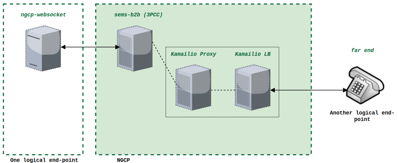
Figure 216. Two logical endpoints in the architecture
