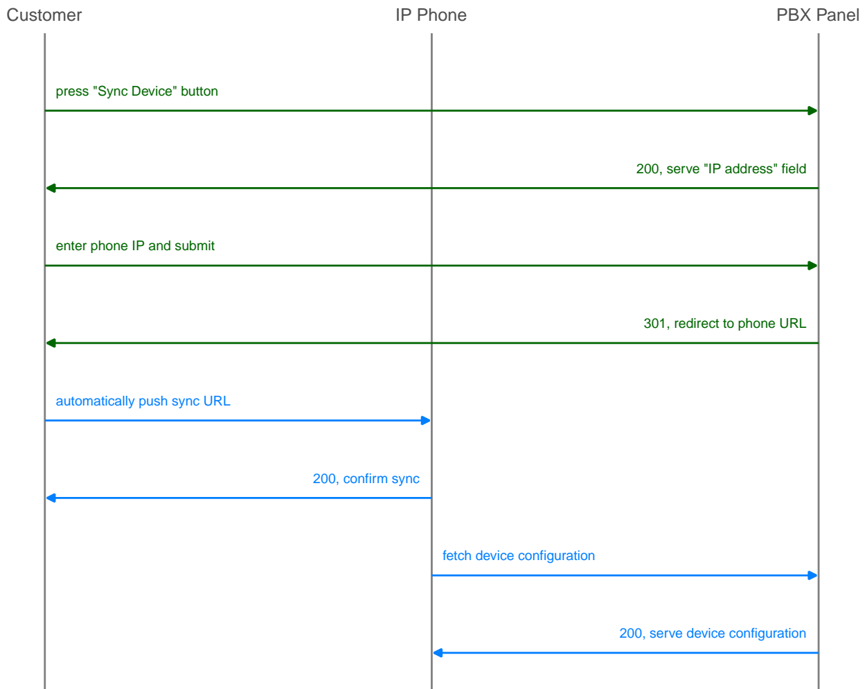
Figure 181. Initially bootstrap a PBX device
