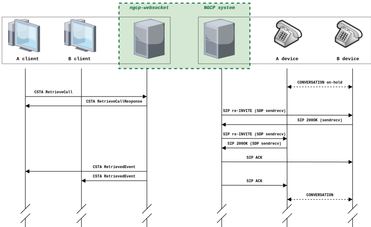
Figure 212. Successful RetrieveCall scenario using SIP re-INVITE
