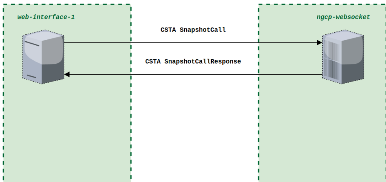
Figure 214. Snapshot Call scenario
