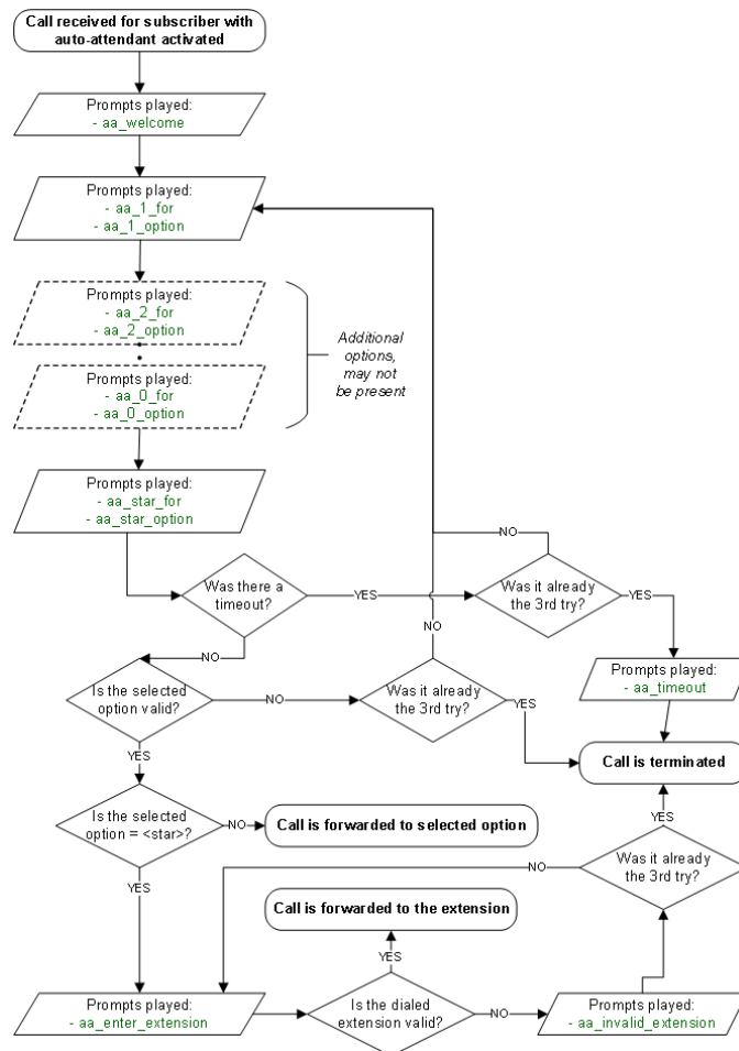
Figure 172. Flowchart of Auto-Attendant
