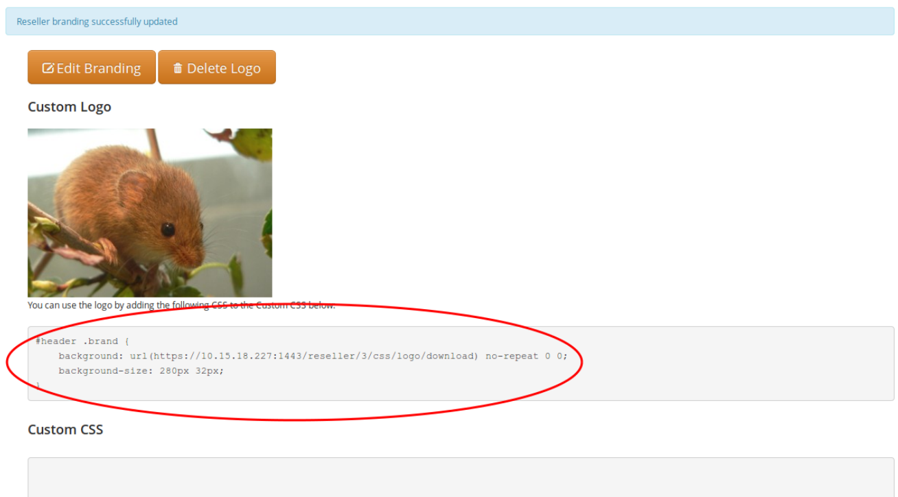
Figure 224. CSC Customisation Step 2: Copy CSS code
