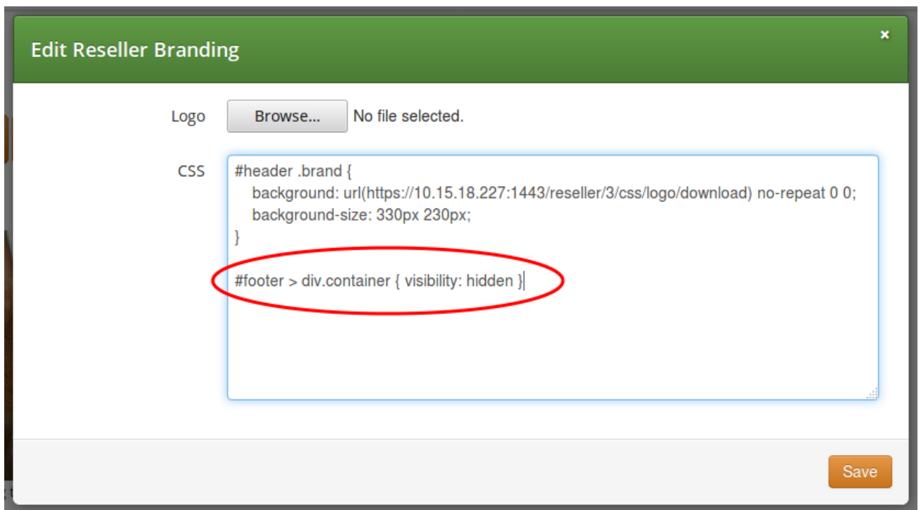
Figure 226. CSC Customisation: Hide copyright notice
