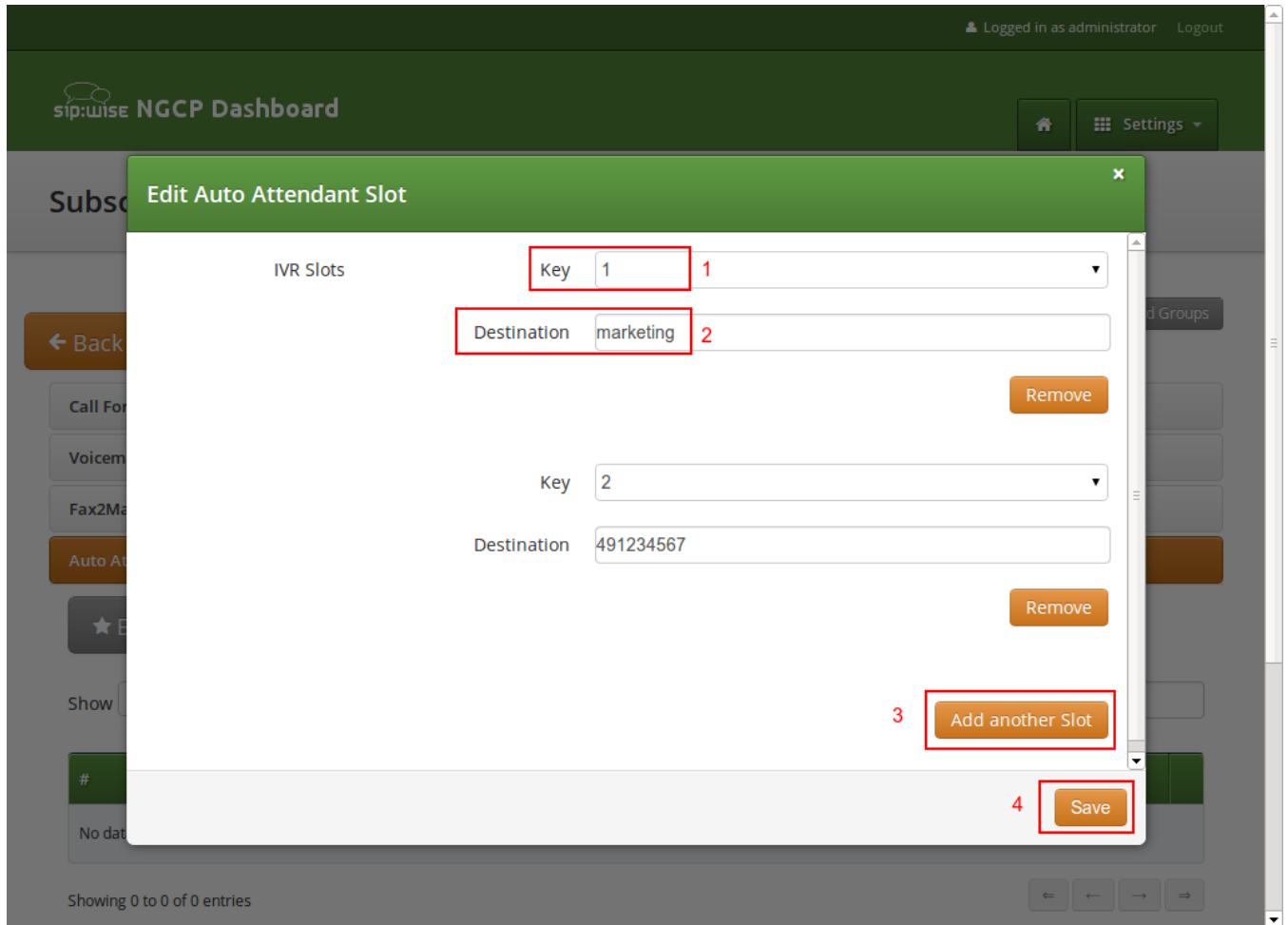
Figure 173. Define the Auto-Attendant Slots
