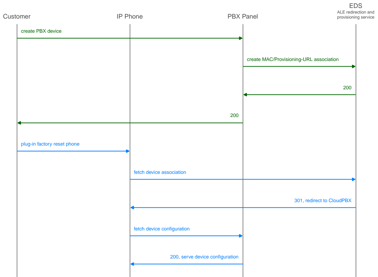
Figure 180. Initially bootstrap an ALE phone
