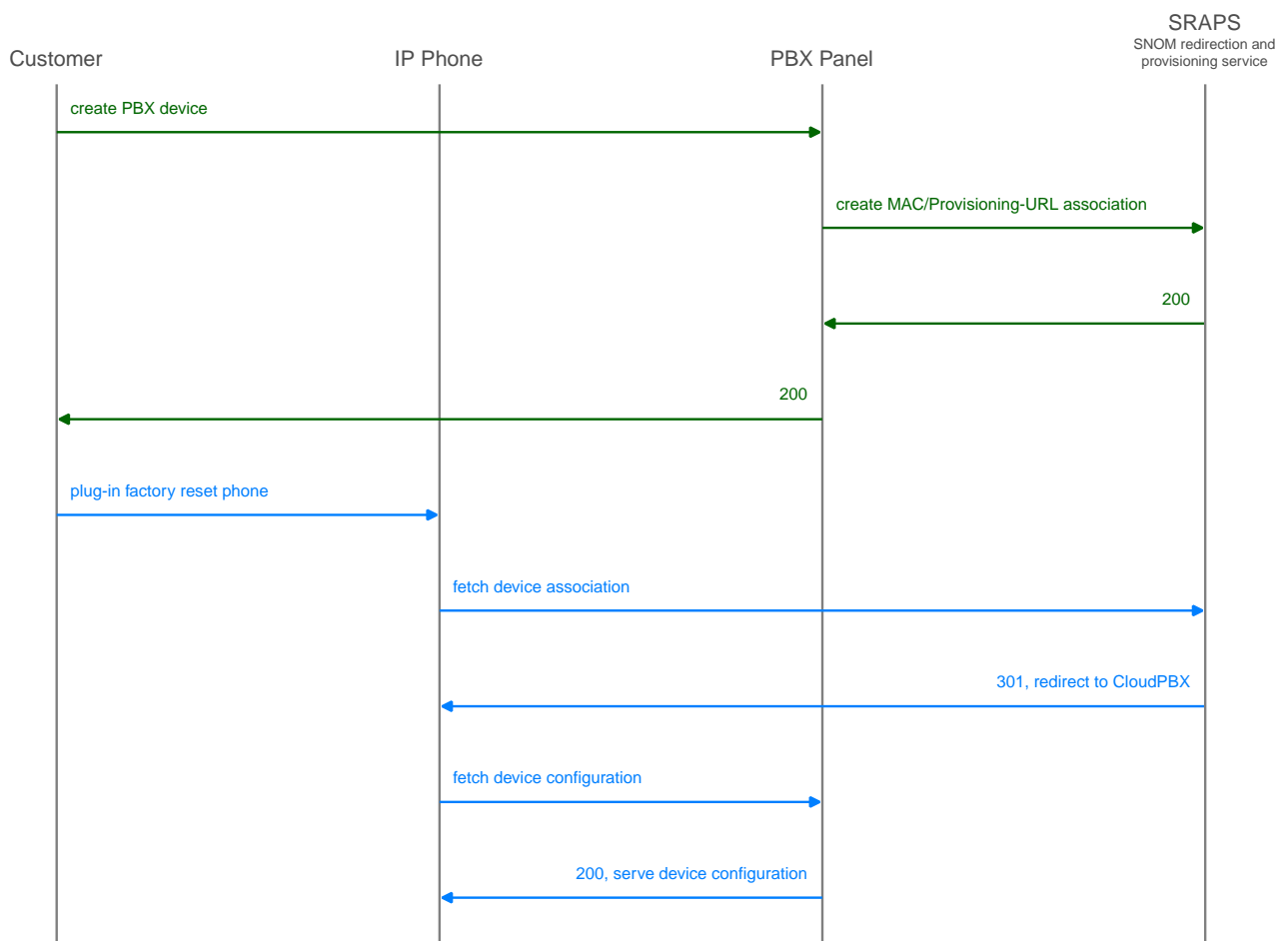
Figure 184. Initially bootstrap a SNOM phone
