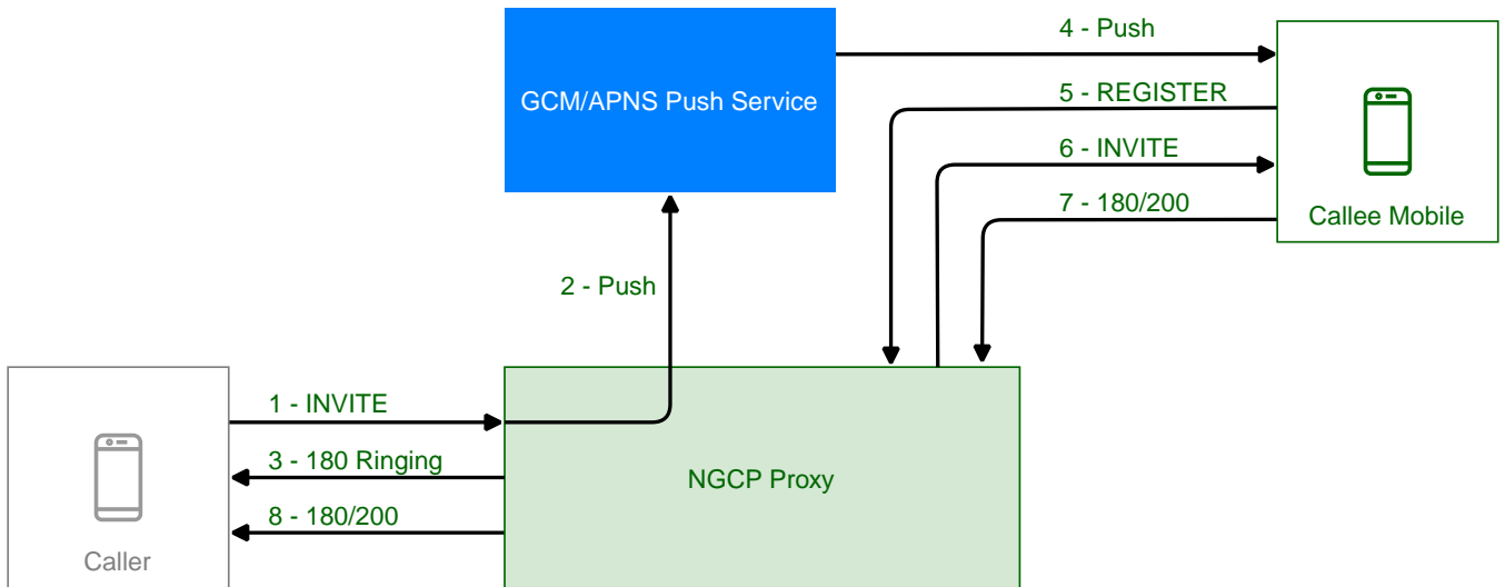
Figure 200. Mobile Push Workflow
