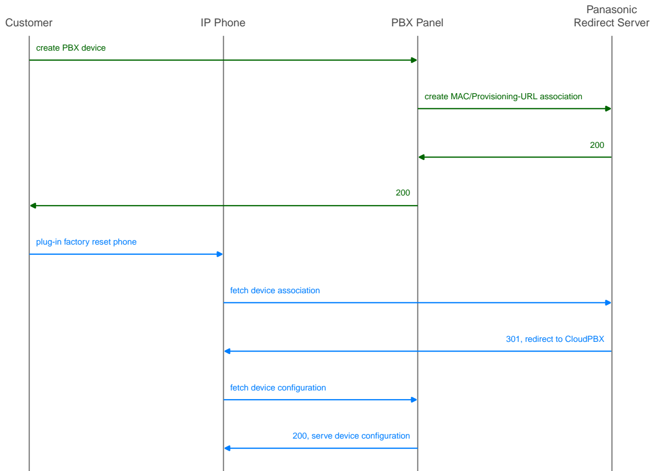
Figure 183. Initially bootstrap a Panasonic phone
