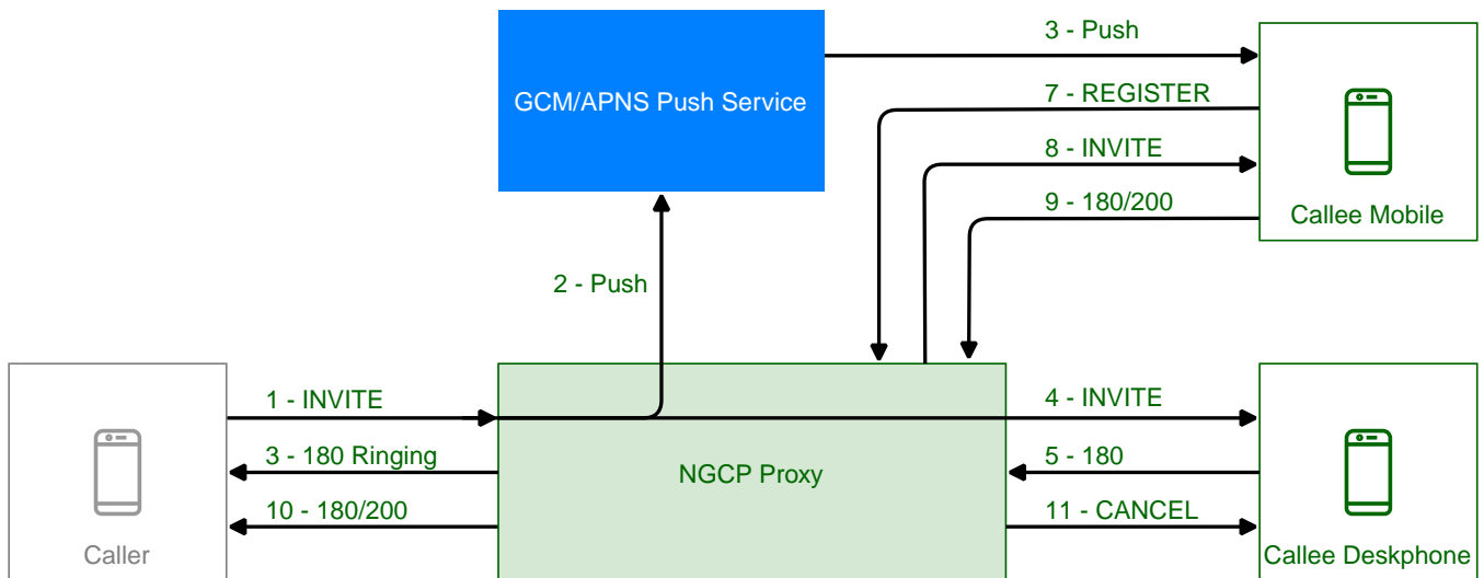
Figure 201. Parallel Mobile Push Workflow
