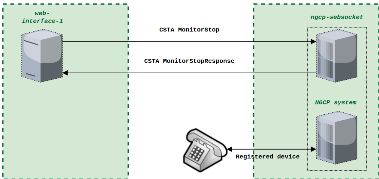
Figure 207. CSTA MonitorStop messages exchange
