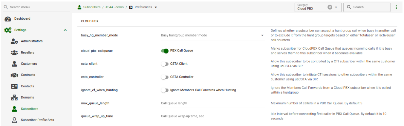
Figure 178. Call Queue Preferences
