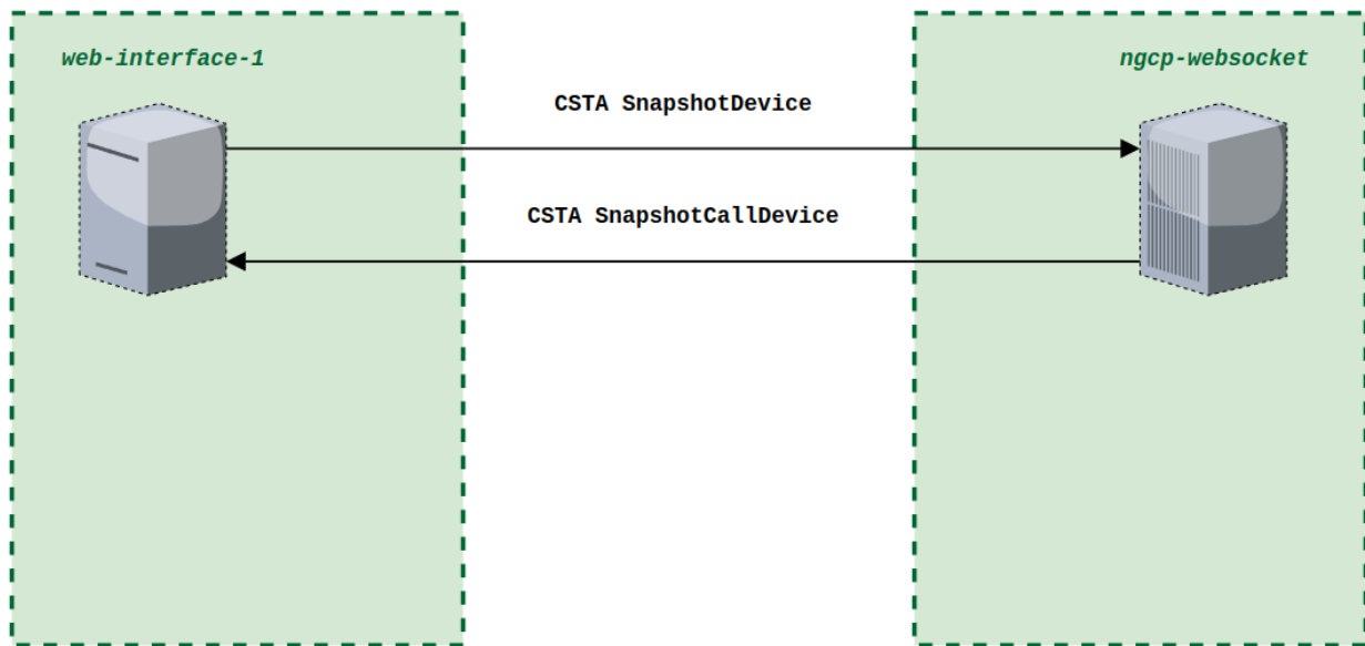
Figure 215. Snapshot Call scenario for a device
