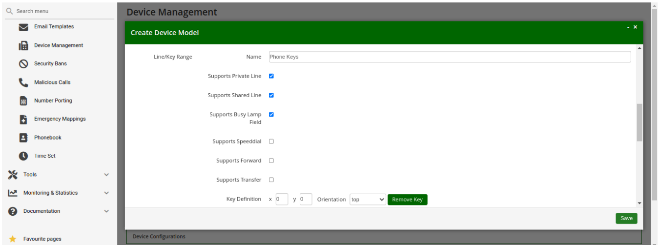
Figure 190. Create Device Model - Lines
