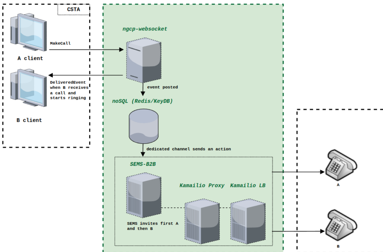
Figure 218. 3PCC dialog initiation
