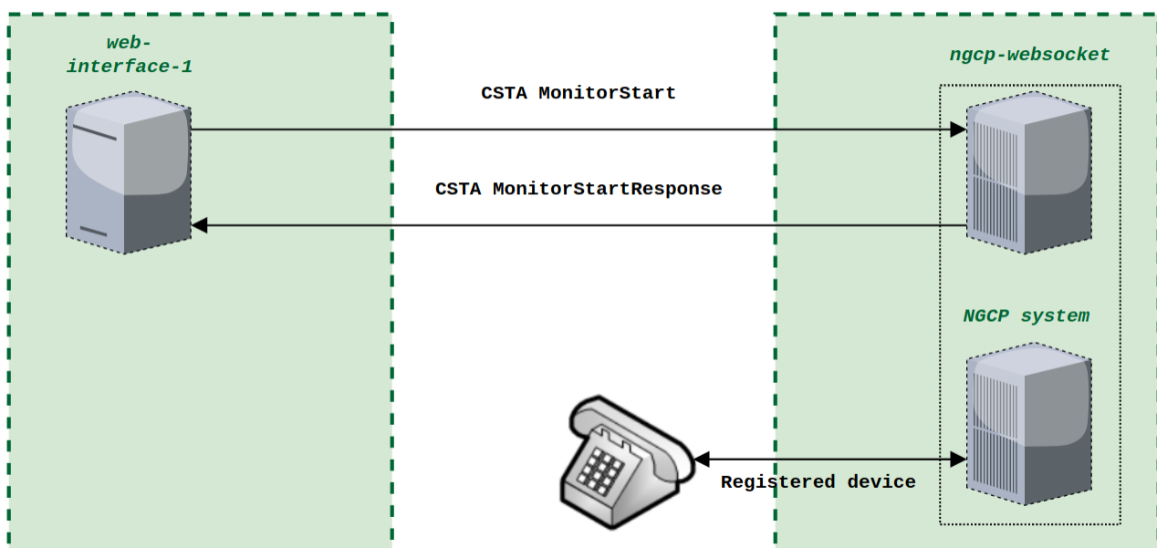
Figure 206. CSTA MonitorStart messages exchange
