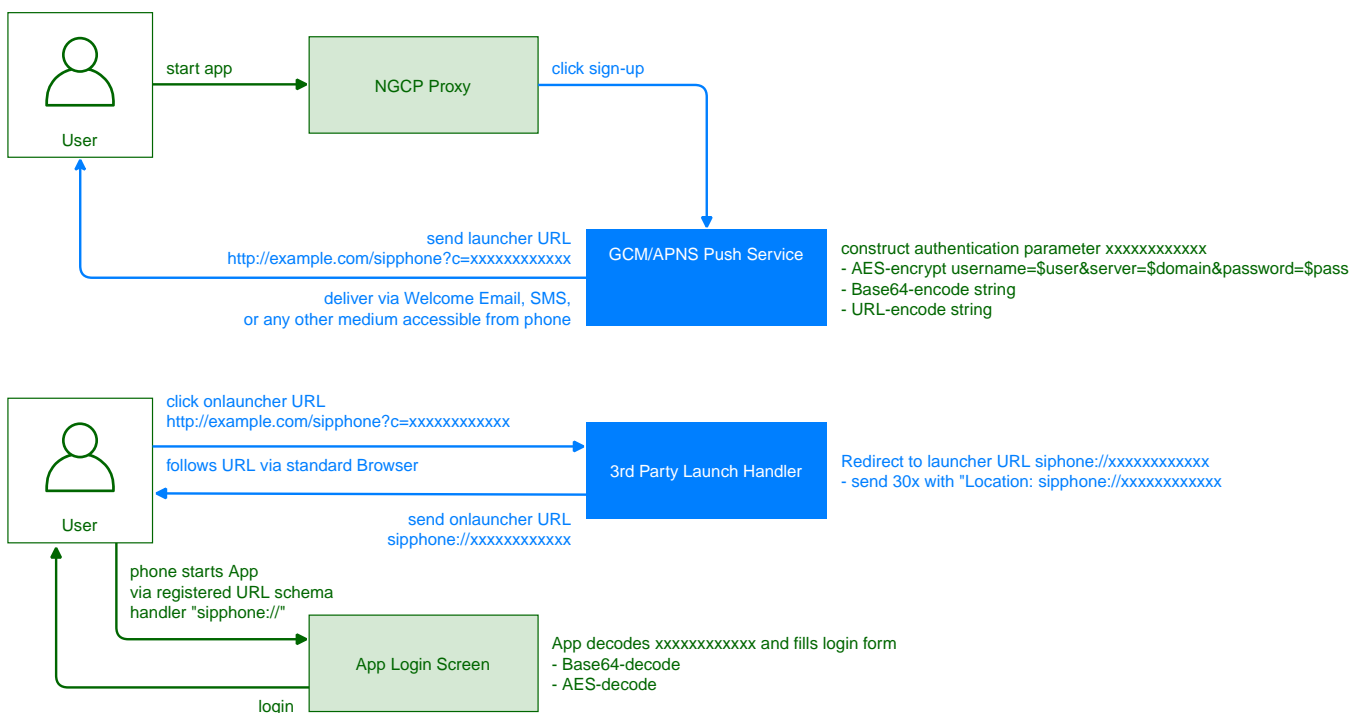
Figure 199. Provisioning Push Workflow
