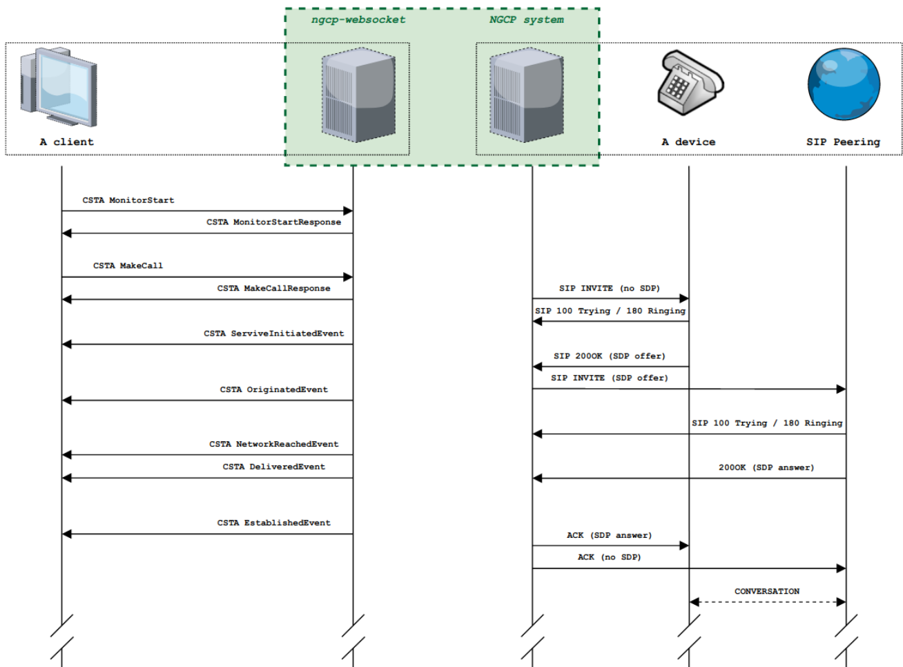
Figure 210. CSTA MakeCall with a SIP Peering, messages exchange
