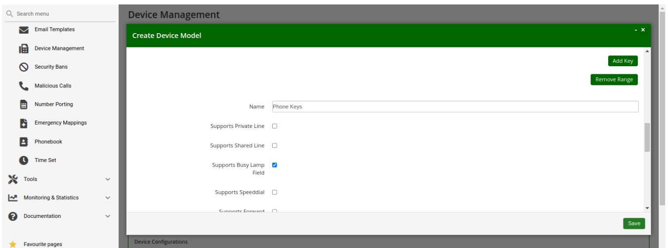
Figure 191. Create Device Model - Add a Line
