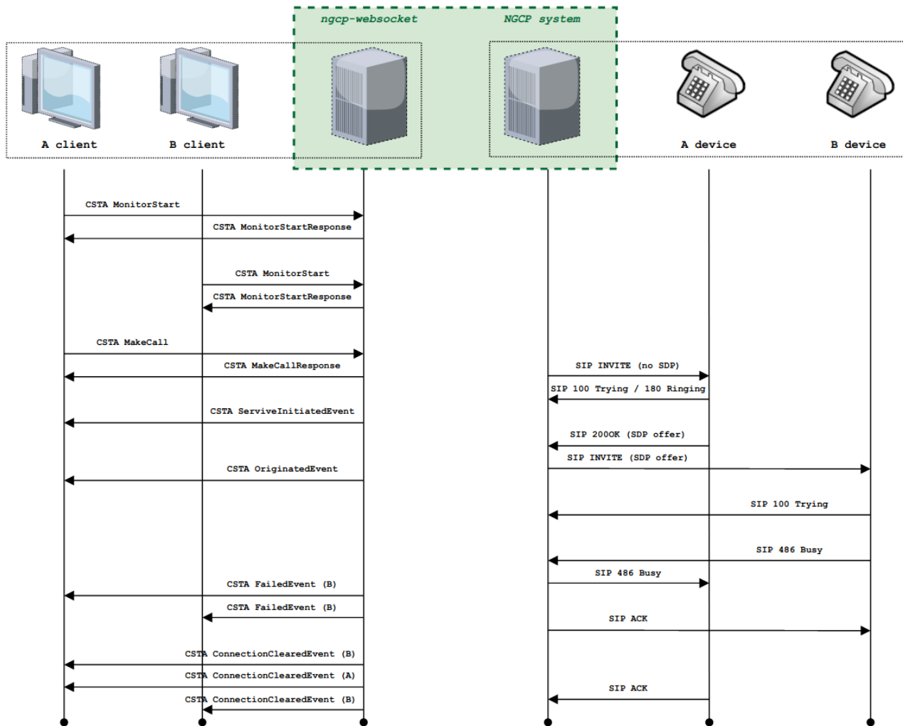
Figure 209. Failed MakeCall scenario (destination is busy)
