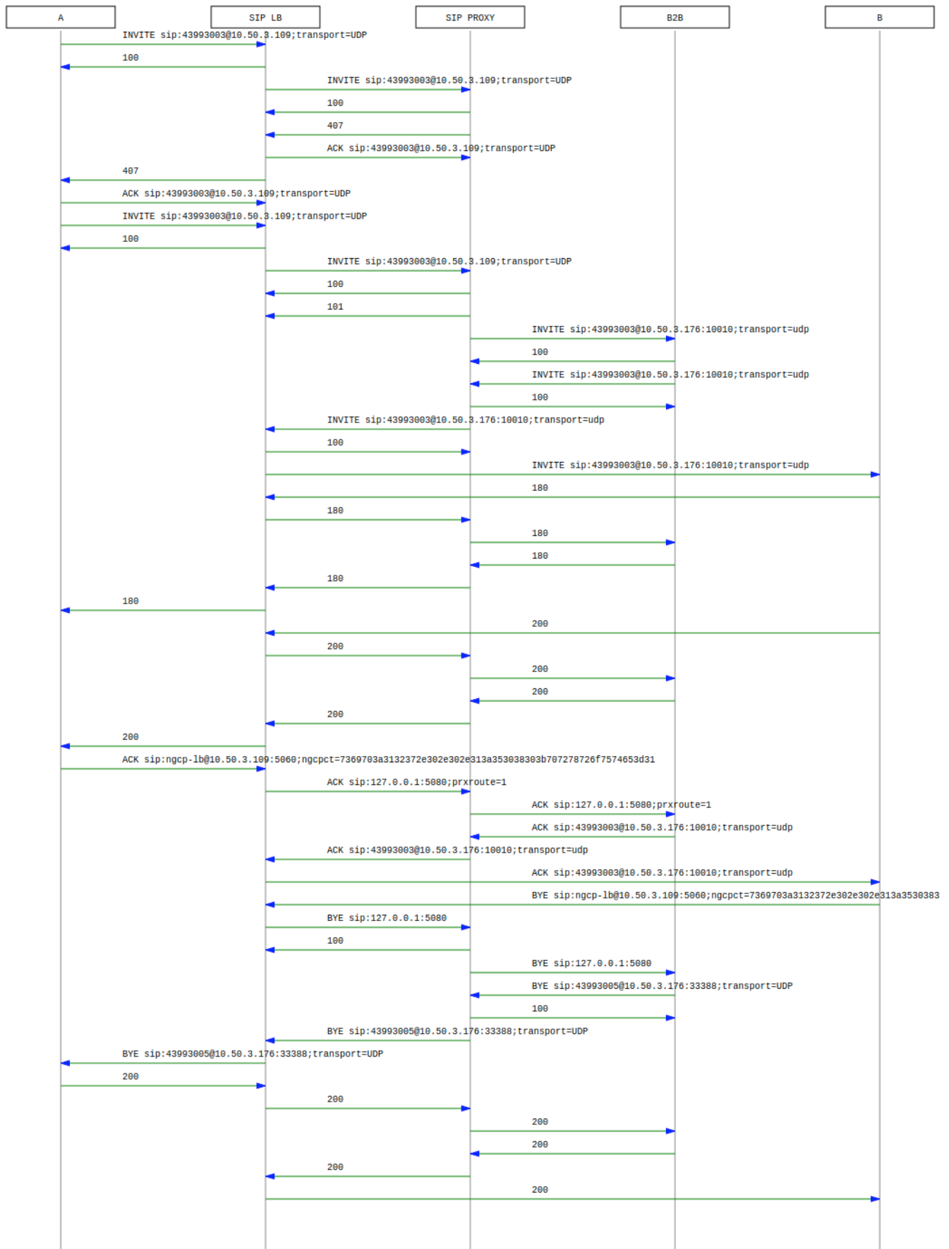
Figure 111. Basic Call Call-Flow
