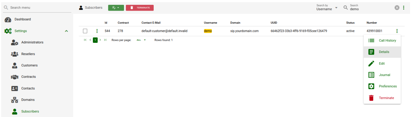
Figure 65. Subscriber Details
