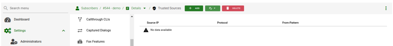
Figure 66. Trusted Sources
