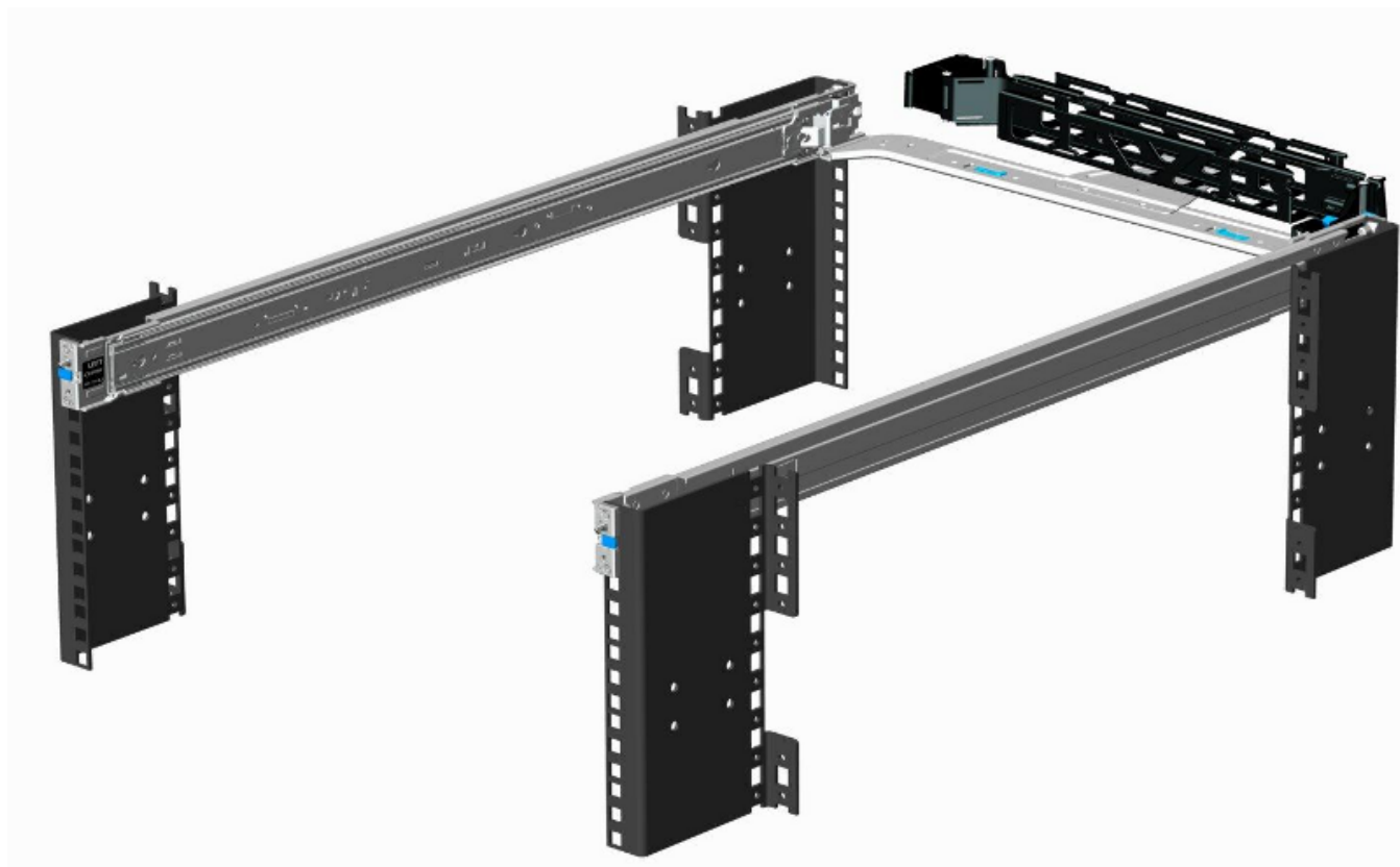
Figure 9. Rack-mounted Rails
