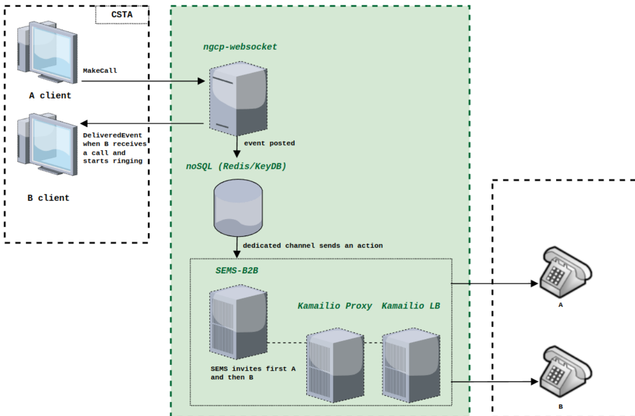
Figure 216. 3PCC dialog initiation
