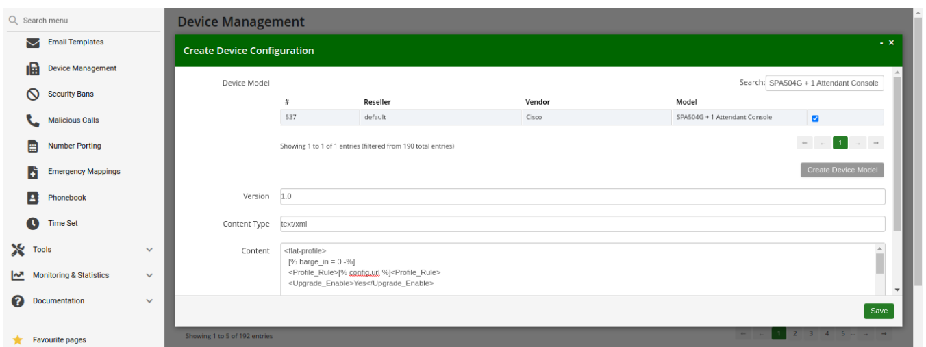
Figure 194. Upload Device Configuration
