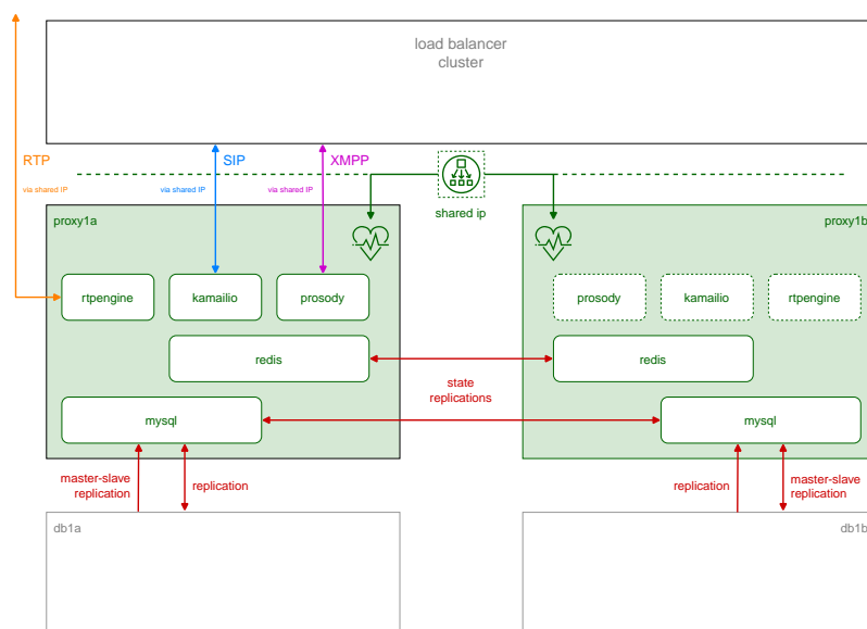
Figure 6. CARRIER Proxy Server Overview
