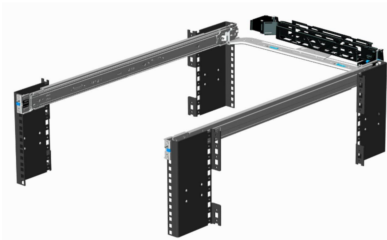
Figure 9. Rack-mounted Rails
