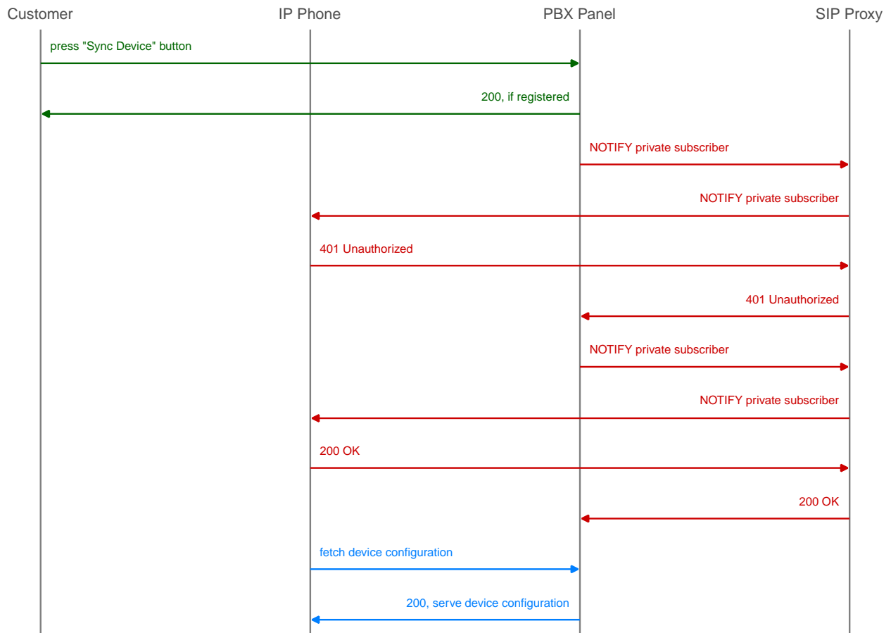
Figure 158. Resync a registered PBX device
