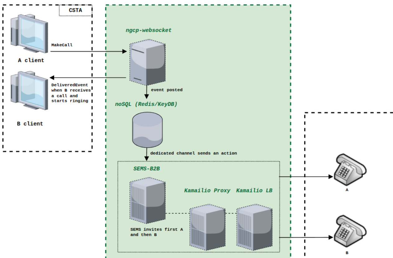
Figure 190. 3PCC dialog initiation
