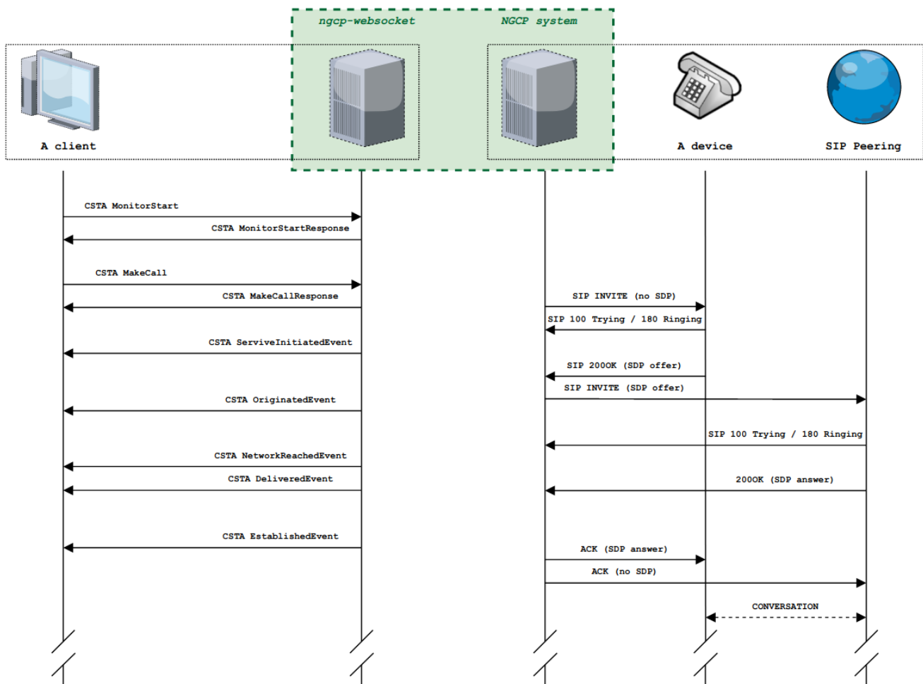
Figure 180. CSTA MakeCall with a SIP Peering, messages exchange
