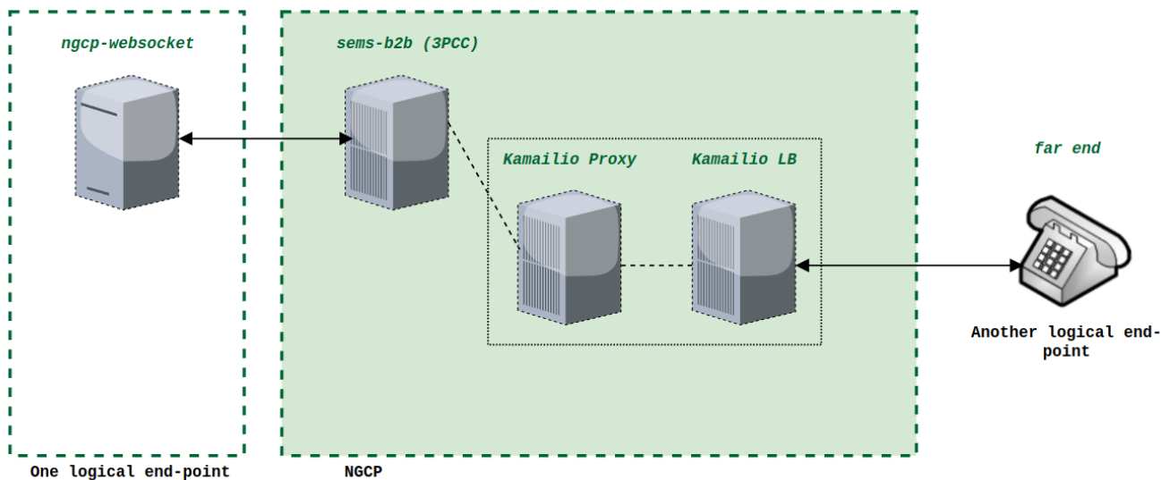
Figure 186. Two logical endpoints in the architecture
