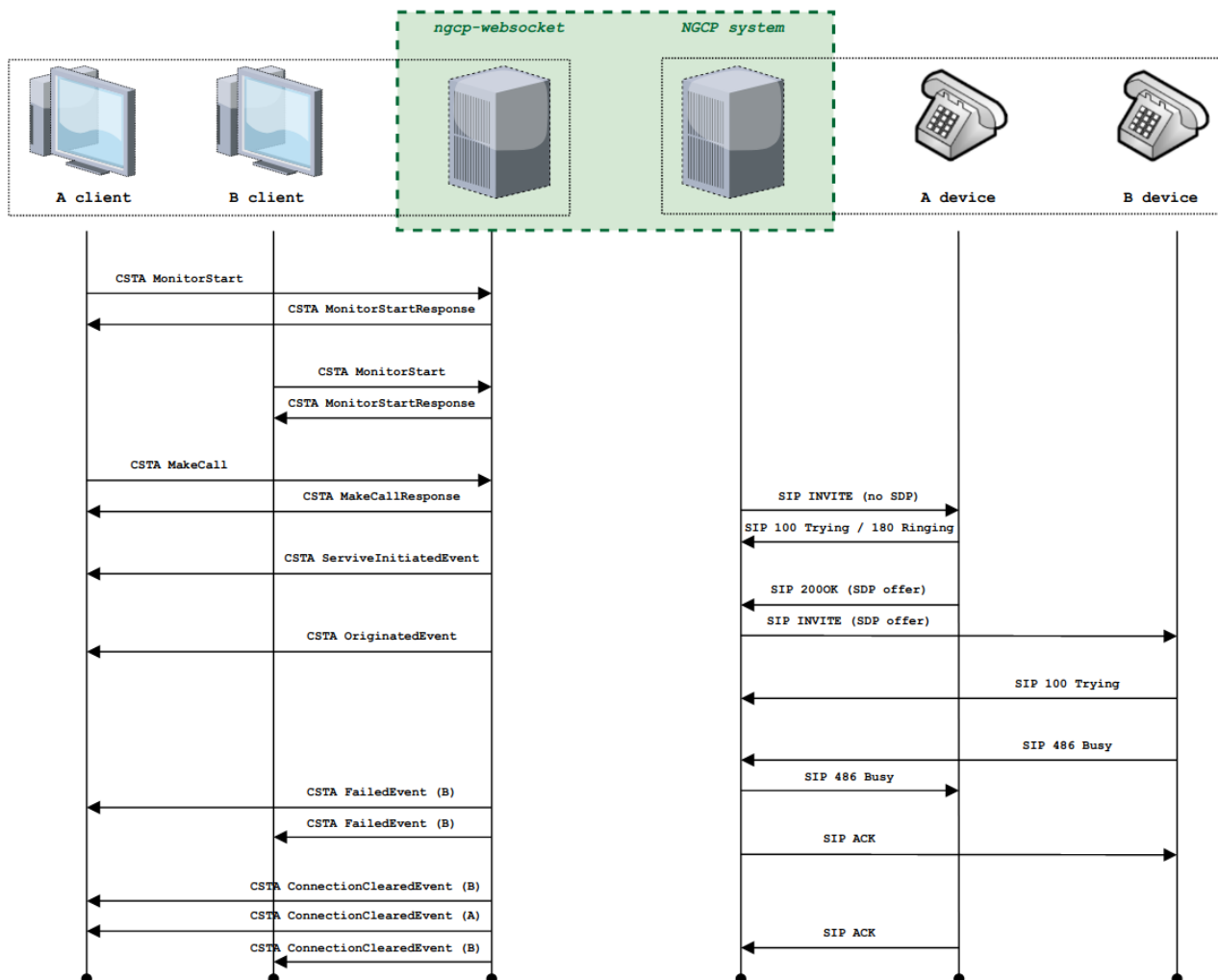
Figure 179. Failed MakeCall scenario (destination is busy)
