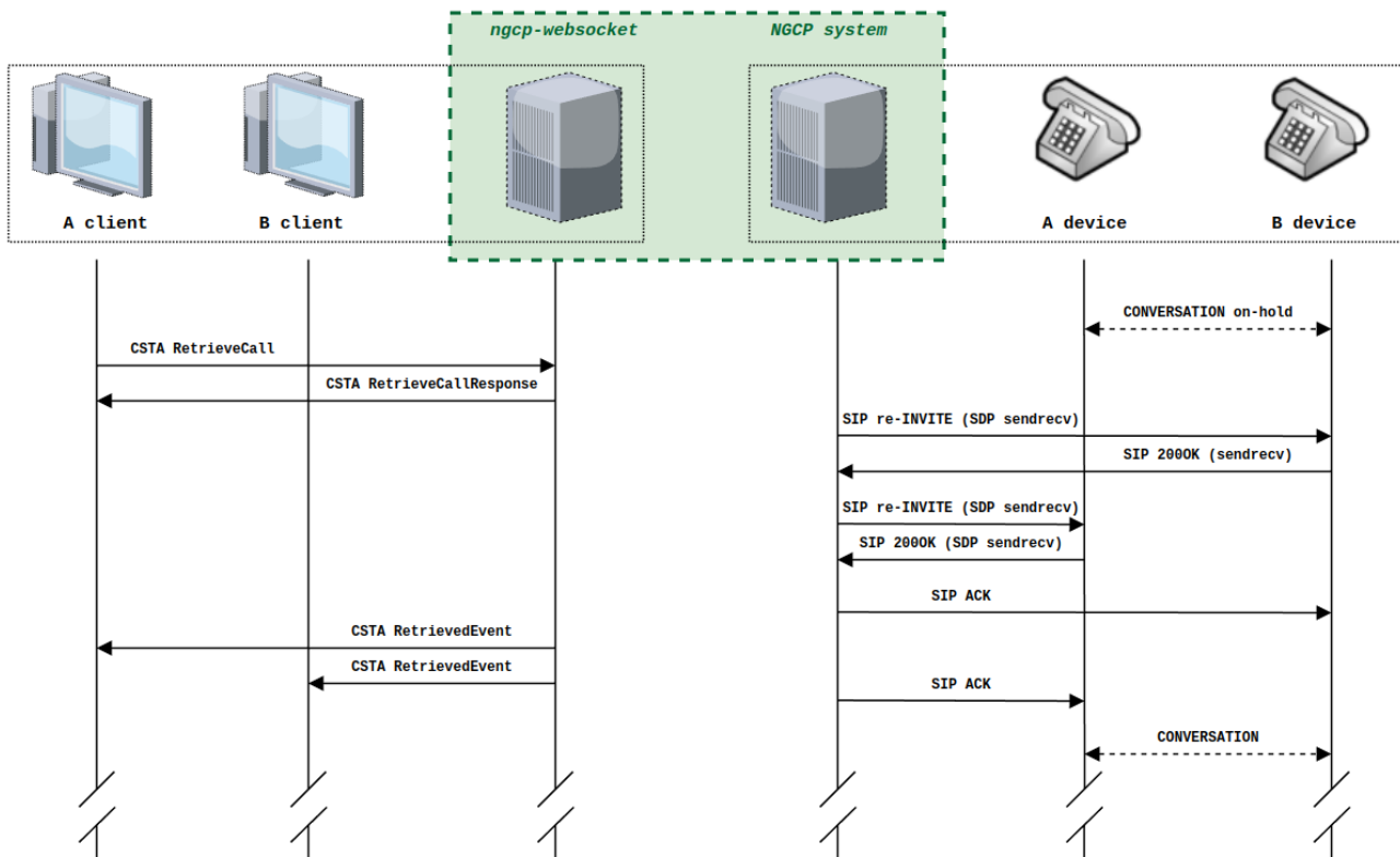
Figure 182. Successful RetrieveCall scenario using SIP re-INVITE
