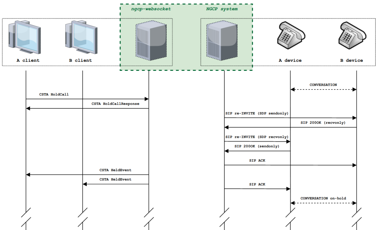
Figure 181. CSTA MakeCall with a SIP Peering, messages exchange
