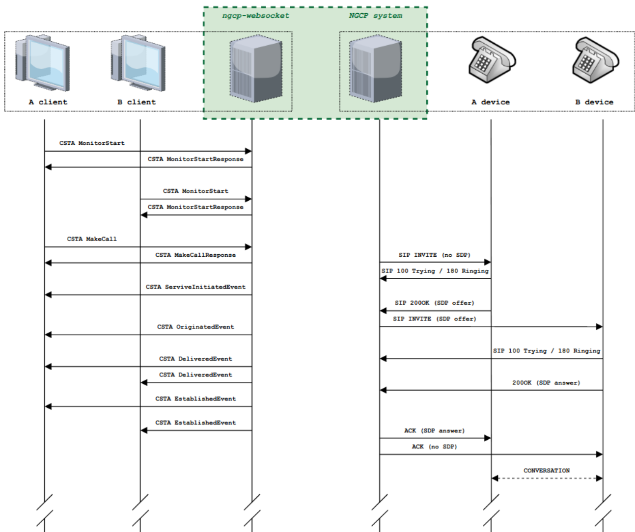
Figure 178. CSTA MakeCall messages exchange
