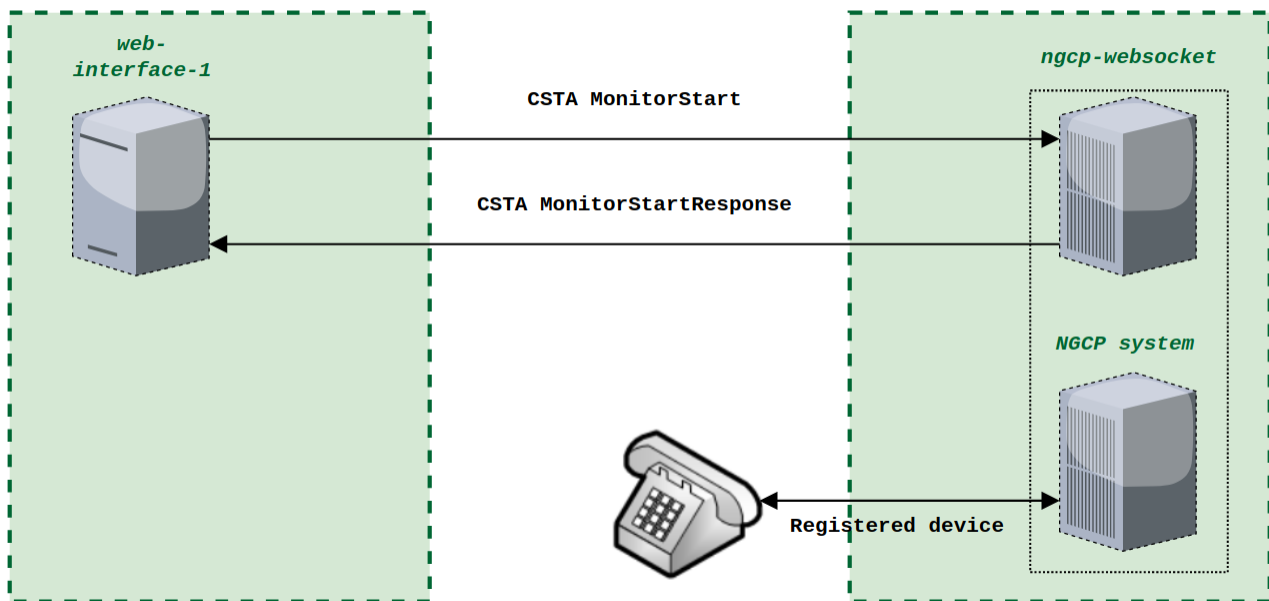
Figure 176. CSTA MonitorStart messages exchange
