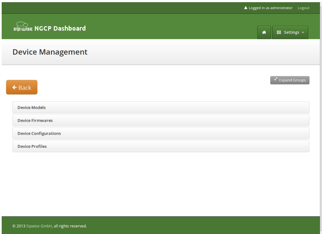
Figure 161. Device Management
