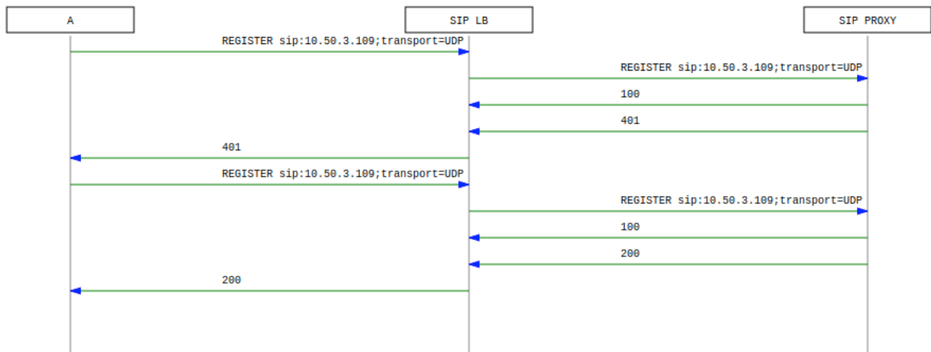
Figure 199. Registration Call-Flow
