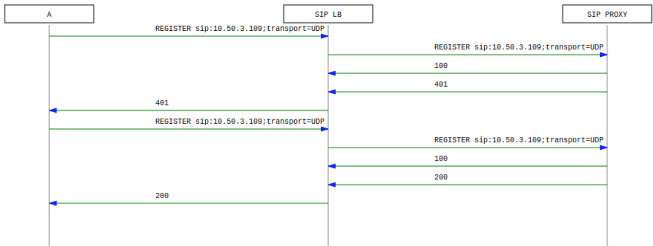
Figure 88. Registration Call-Flow
