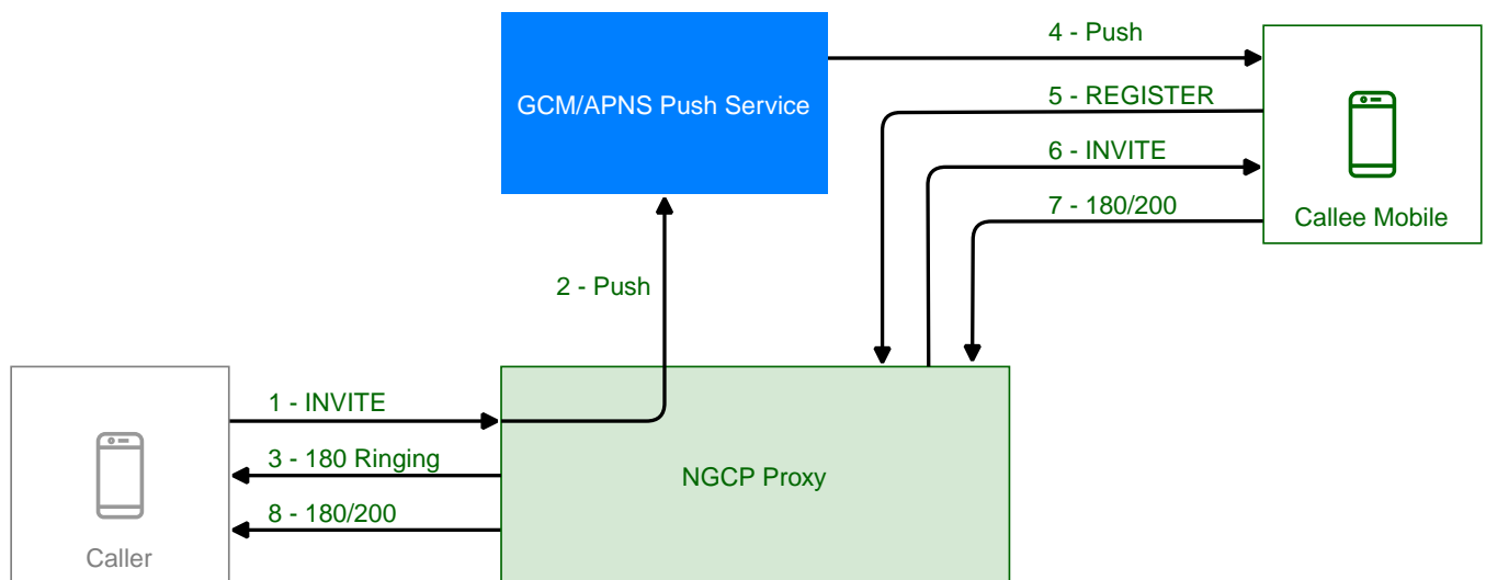
Figure 170. Mobile Push Workflow
