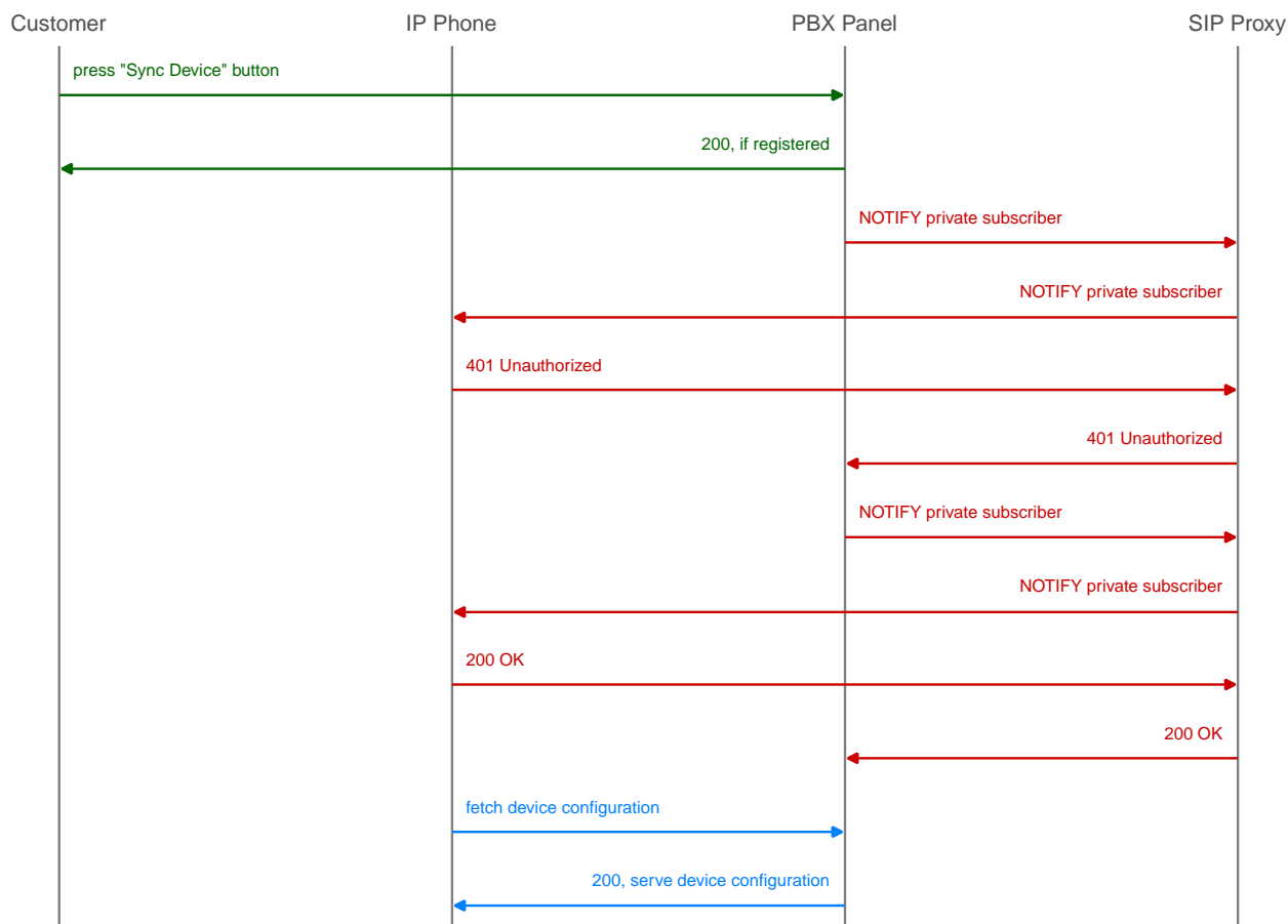
Figure 155. Resync a registered PBX device
