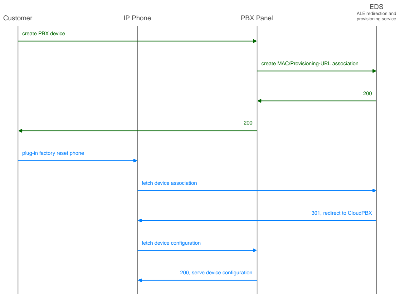
Figure 153. Initially bootstrap an ALE phone
