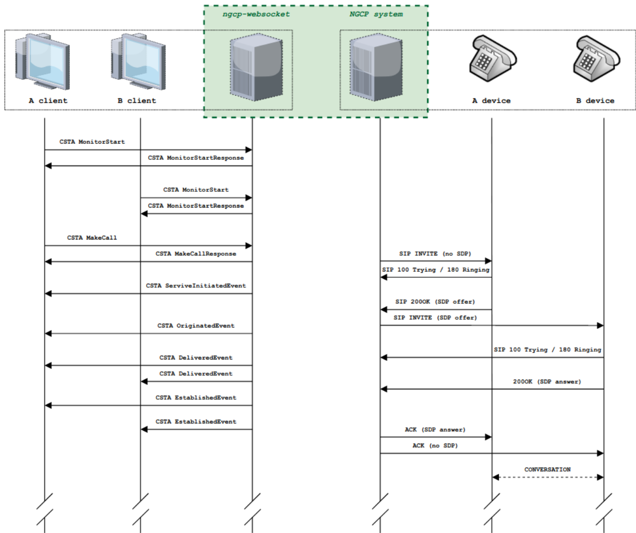
Figure 187. CSTA MakeCall messages exchange
