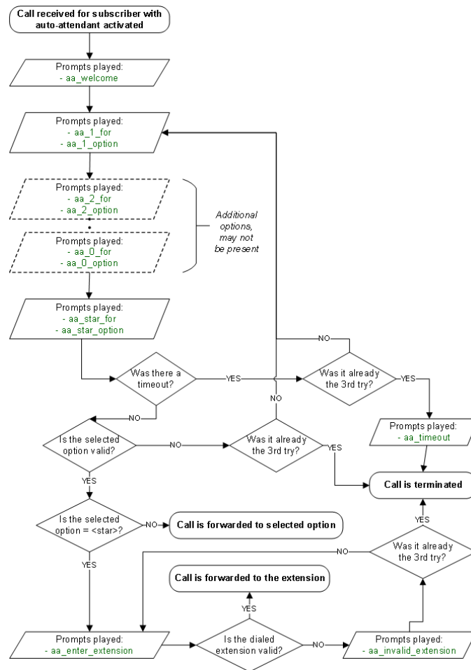
Figure 146. Flowchart of Auto-Attendant
