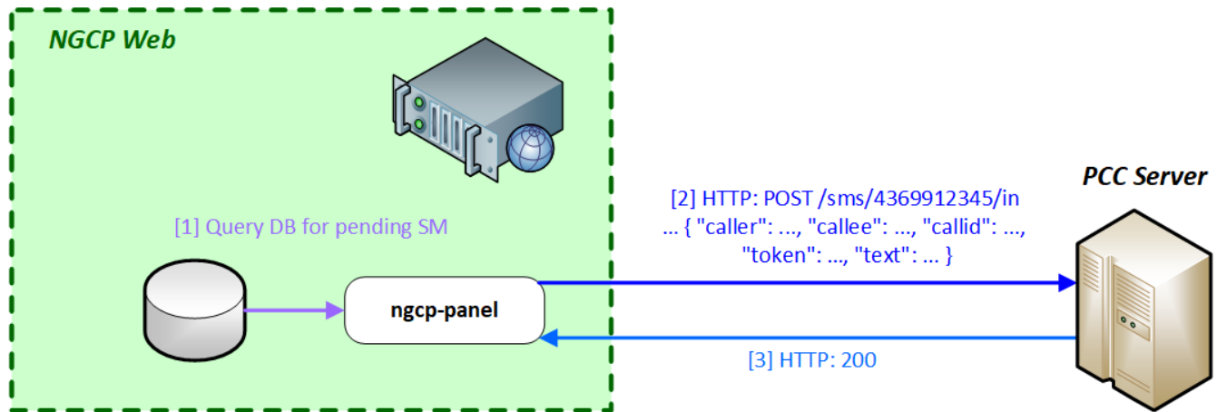
Figure 182. Short Message Notification with PCC
