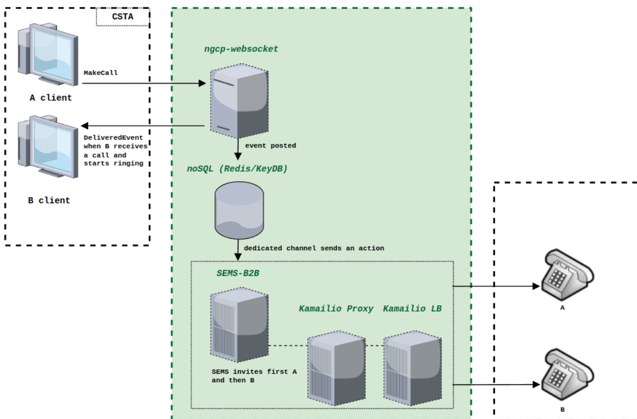
Figure 197. 3PCC dialog initiation
