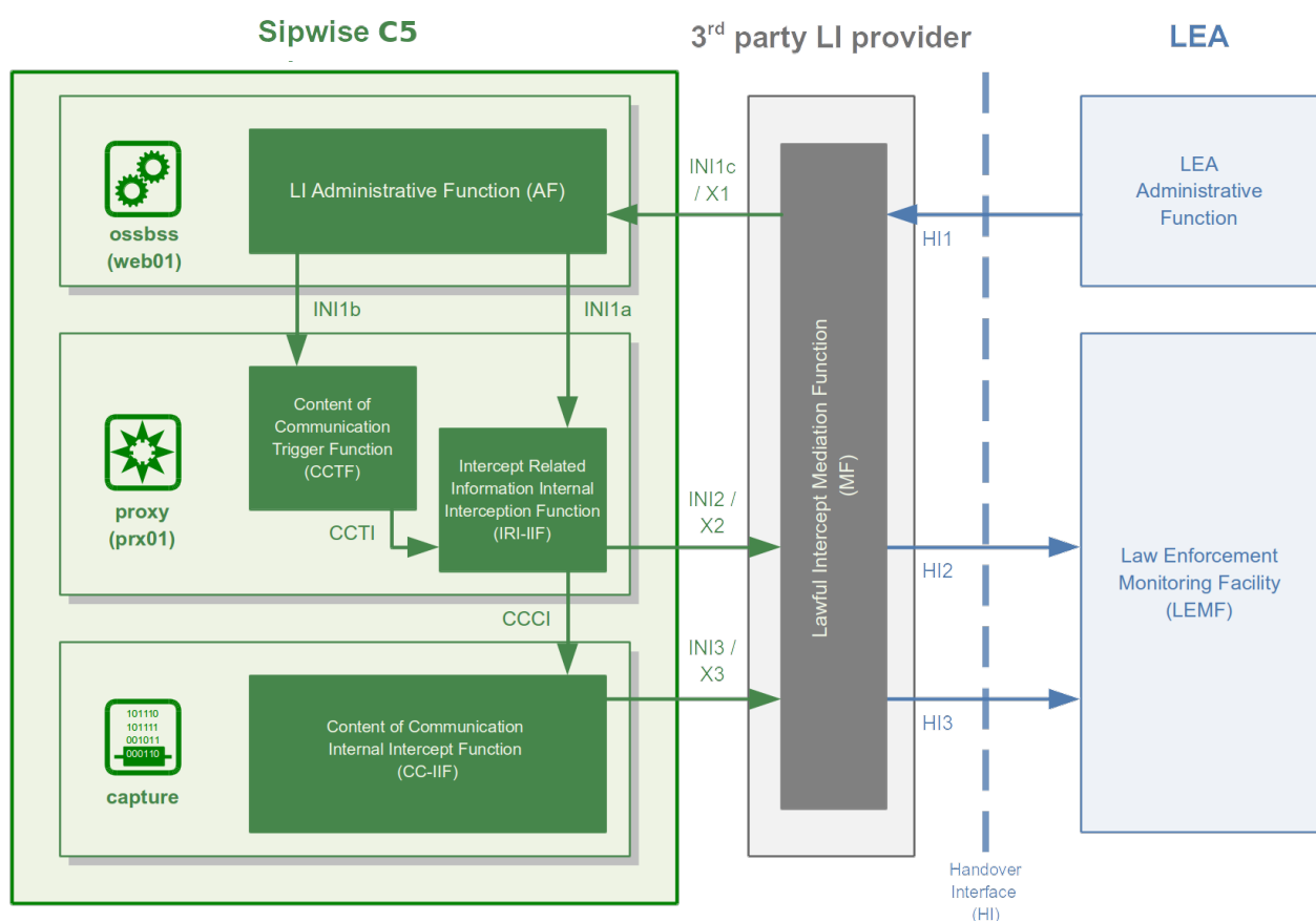
Figure 173. LI with 3rd Party Provider
