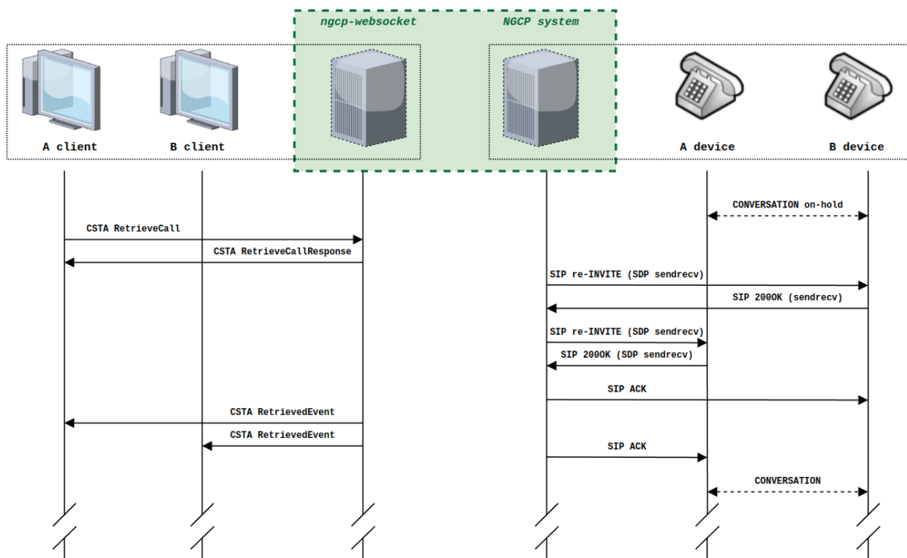
Figure 191. Successful RetrieveCall scenario using SIP re-INVITE
