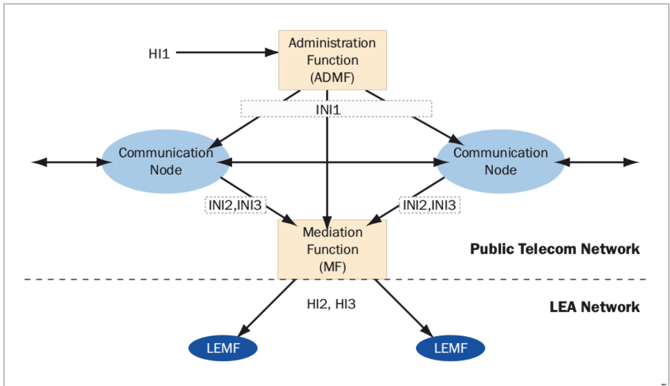
Figure 172. LI: ETSI Interfaces
