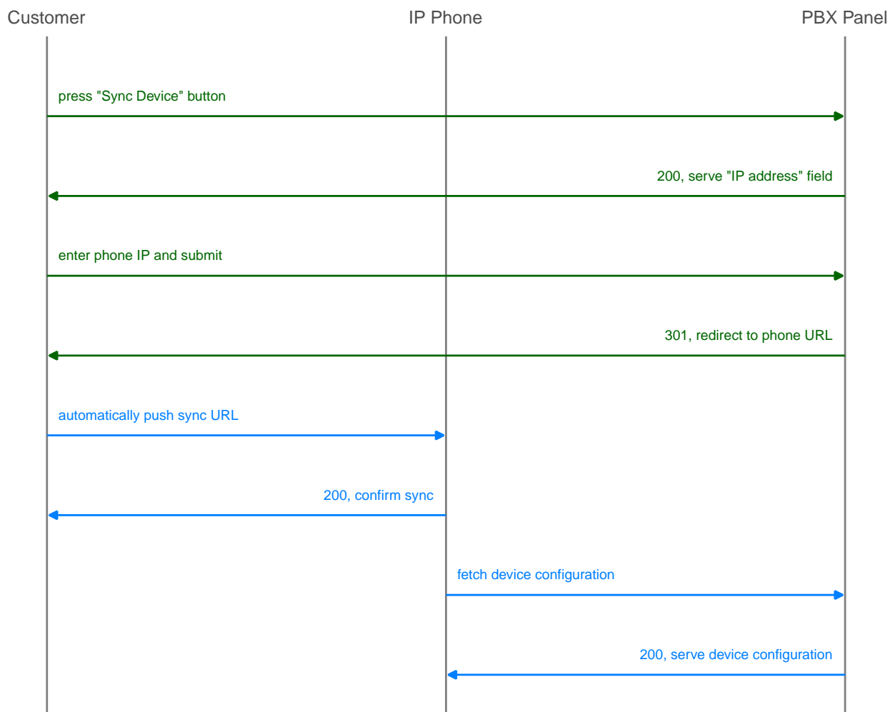
Figure 154. Initially bootstrap a PBX device
