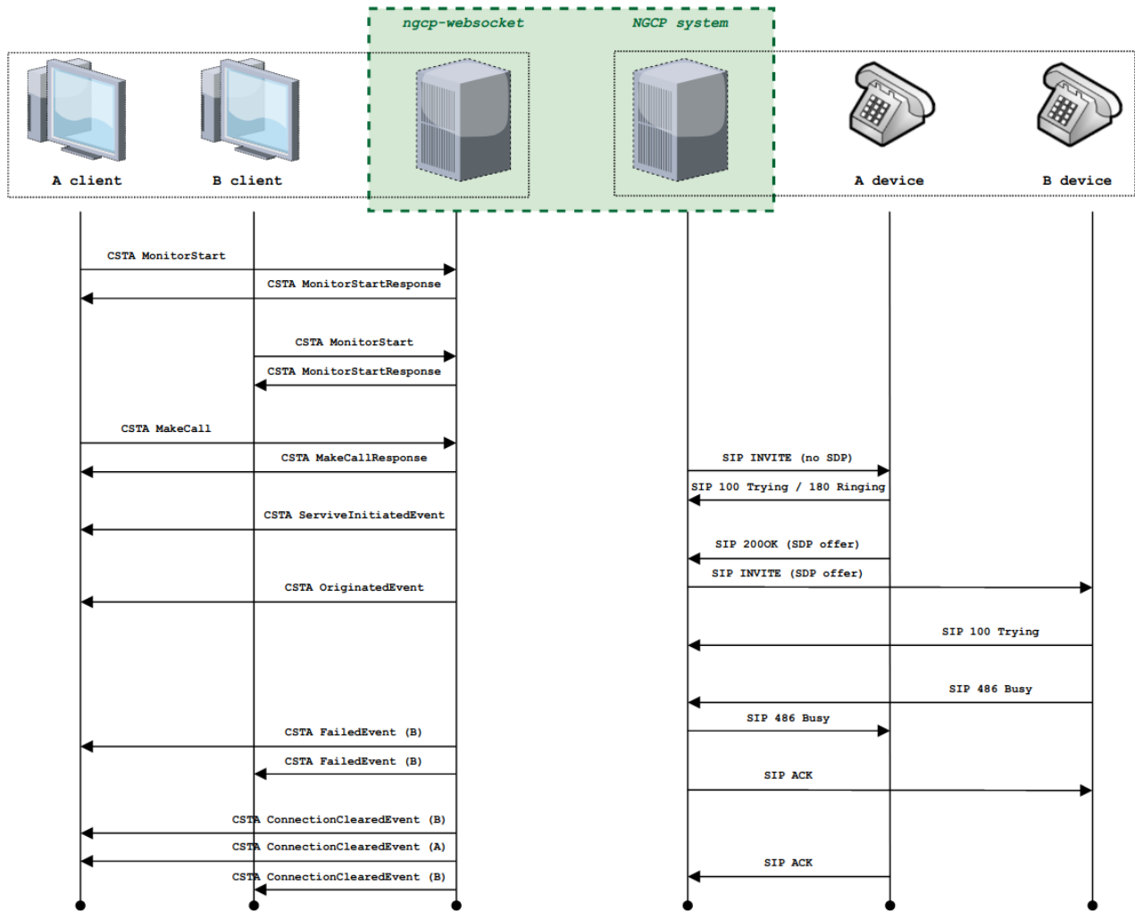
Figure 188. Failed MakeCall scenario (destination is busy)
