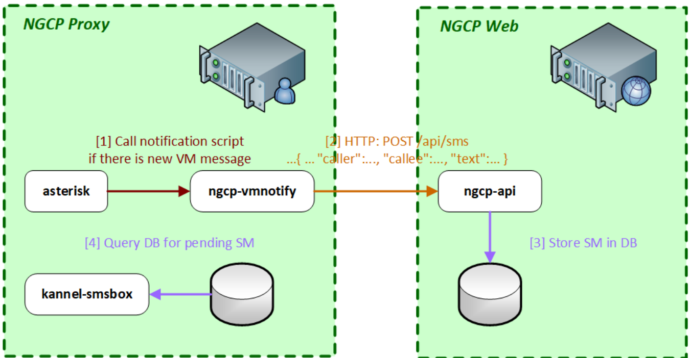
Figure 181. Voicemail Notification with SMS
