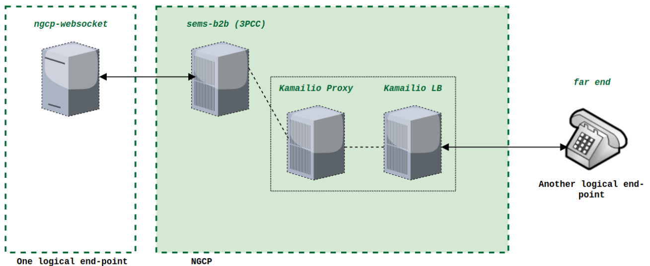
Figure 195. Two logical endpoints in the architecture
