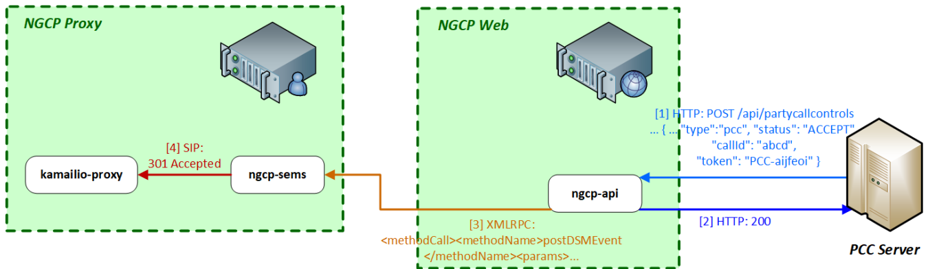
Figure 178. Call Accepted by PCC
