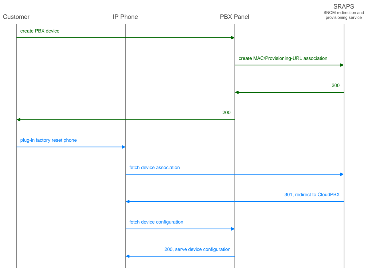
Figure 157. Initially bootstrap a SNOM phone
