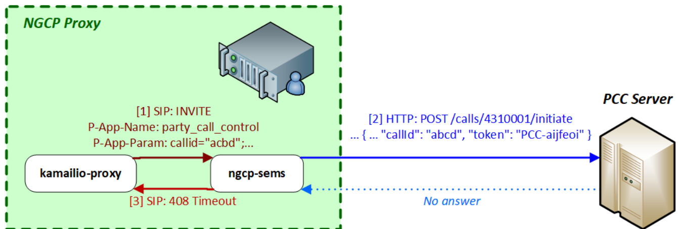
Figure 177. Call Initiation Timeout with PCC
