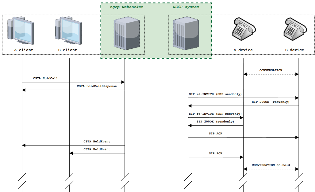
Figure 190. CSTA MakeCall with a SIP Peering, messages exchange
