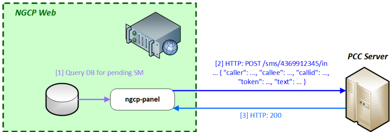
Figure 179. Short Message Notification with PCC
