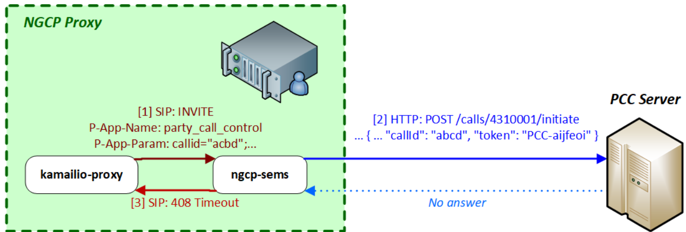
Figure 174. Call Initiation Timeout with PCC
