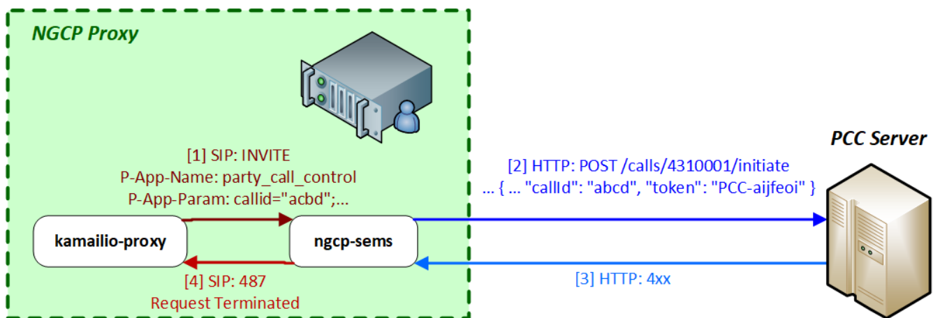
Figure 173. Call Initiation Error with PCC
