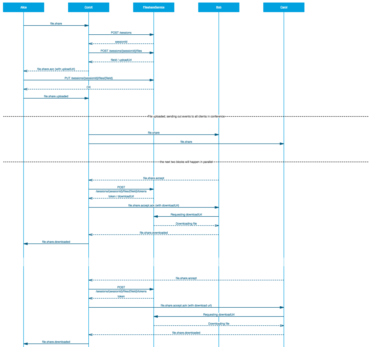
Figure 184. Sequence Detailed
