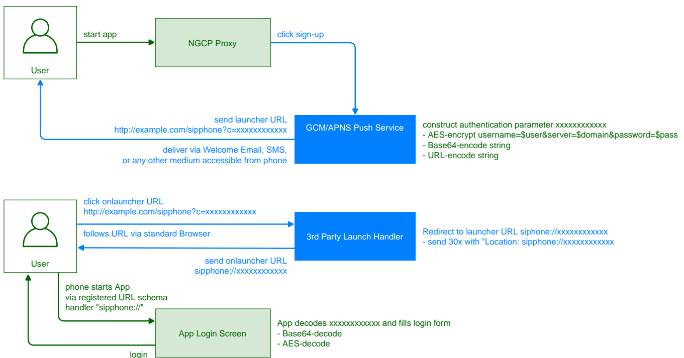
Figure 165. Provisioning Push Workflow
