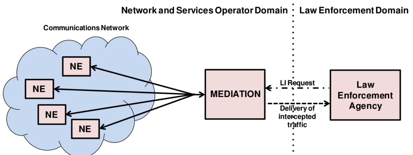
Figure 168. LI: High Level Overview
