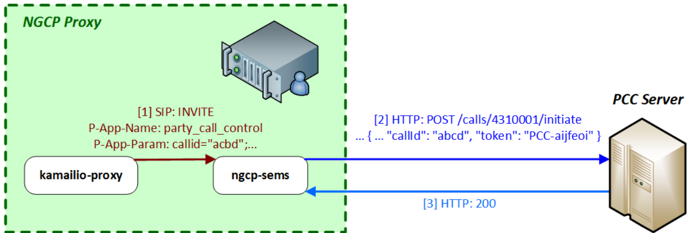
Figure 172. Successful Call Initiation with PCC
