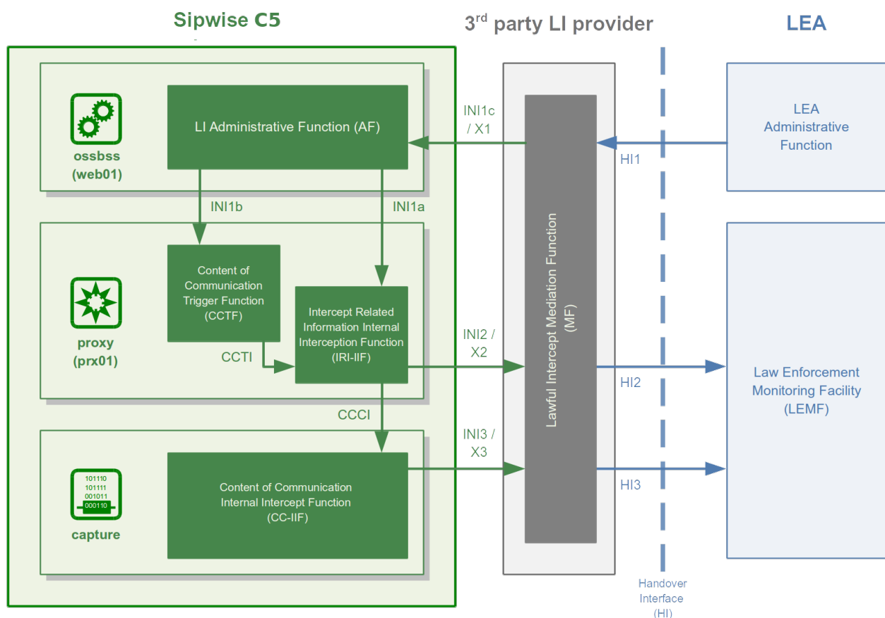
Figure 170. LI with 3rd Party Provider
