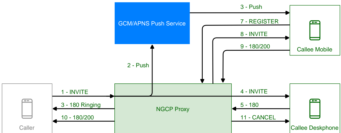
Figure 167. Parallel Mobile Push Workflow
