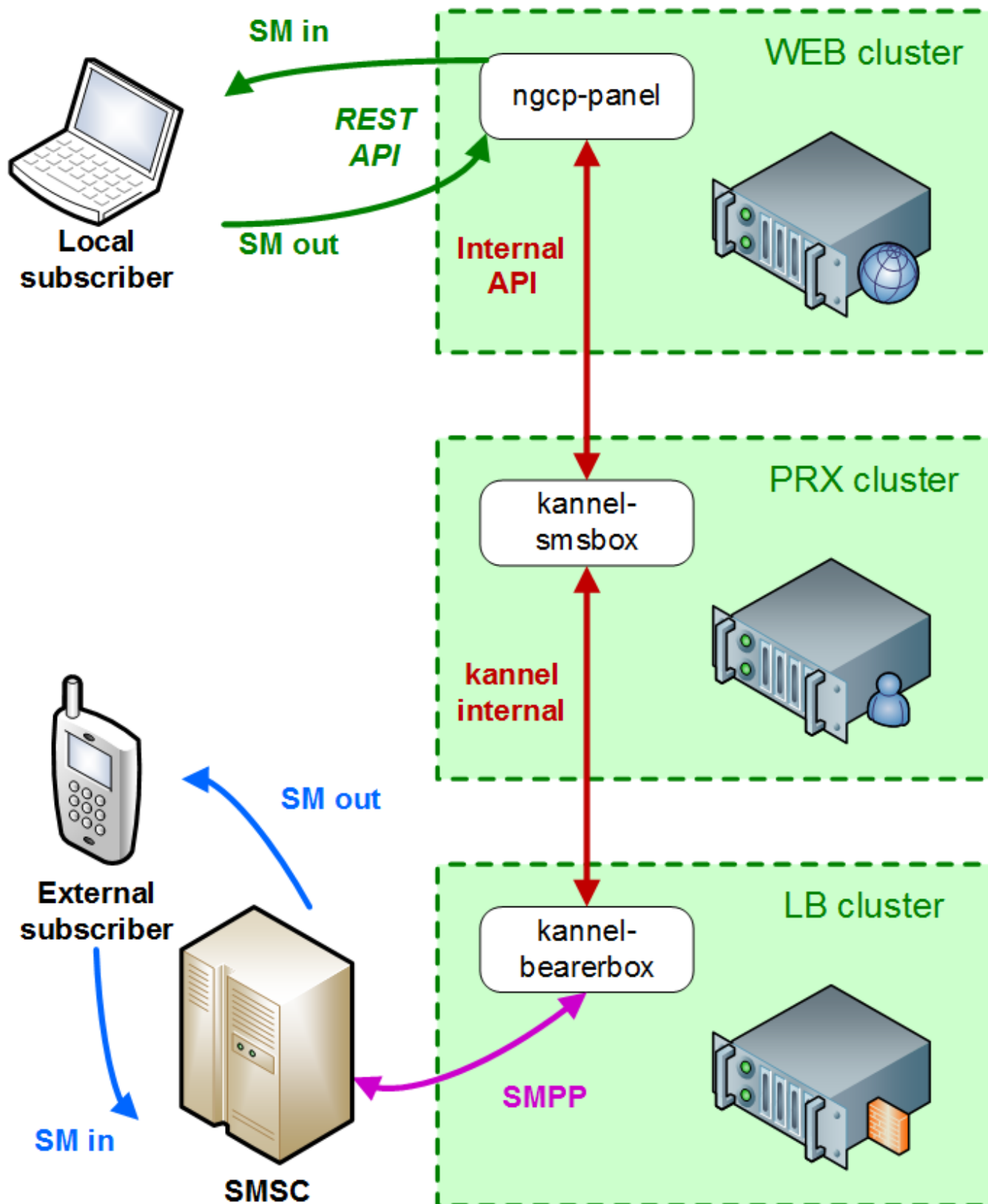
Figure 181. SMS Interaction
