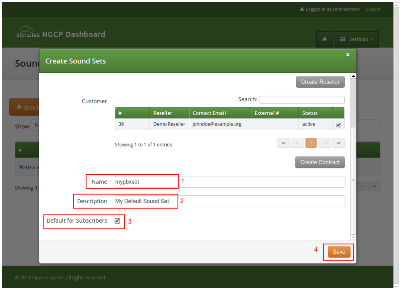
Figure 138. Create Customer Sound Set
