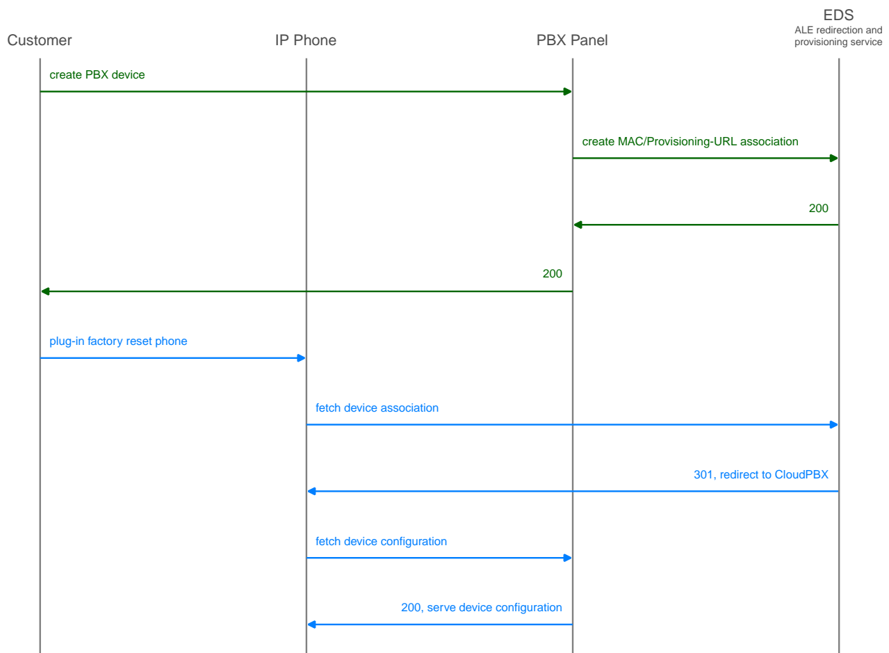
Figure 148. Initially bootstrap an ALE phone
