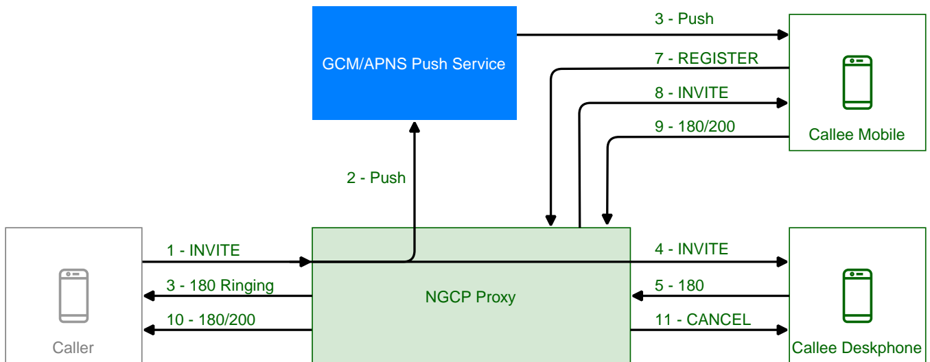
Figure 165. Parallel Mobile Push Workflow
