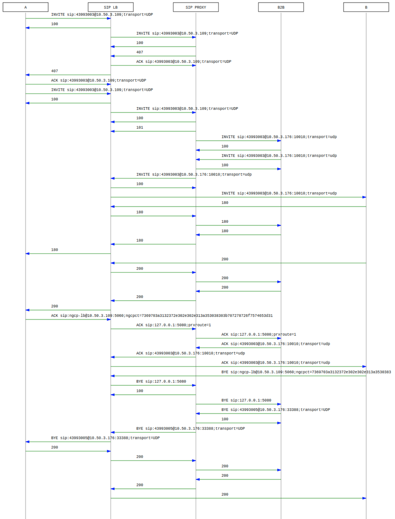
Figure 192. Basic Call Call-Flow
