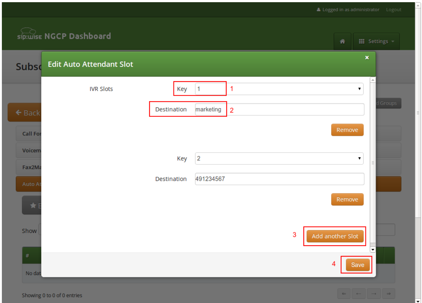
Figure 144. Define the Auto-Attendant Slots
