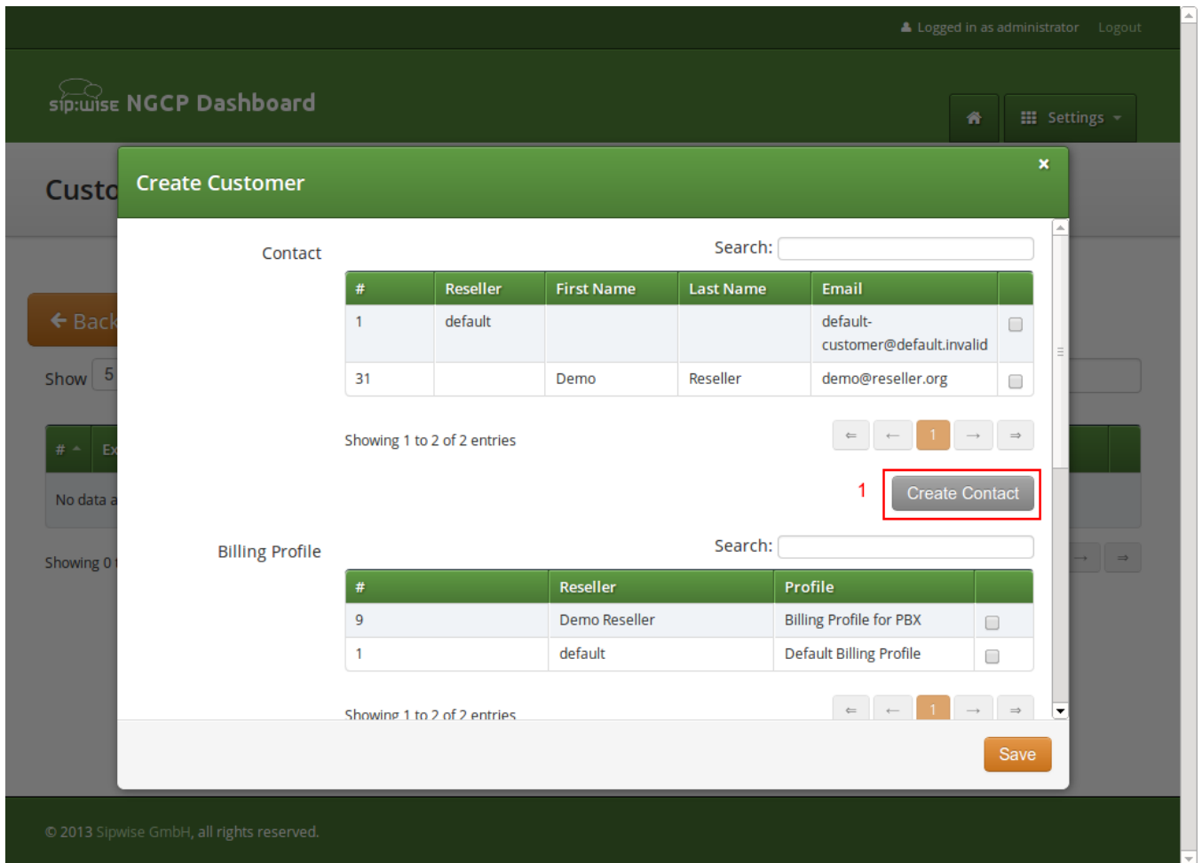
Figure 113. Create PBX Customer Part 1
