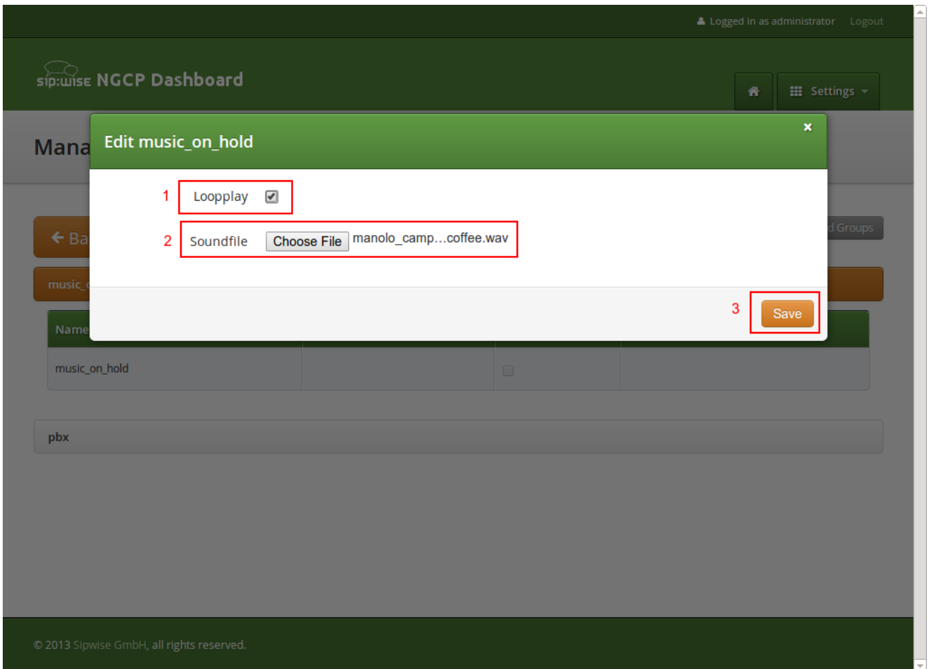
Figure 139. Upload MoH Sound File
