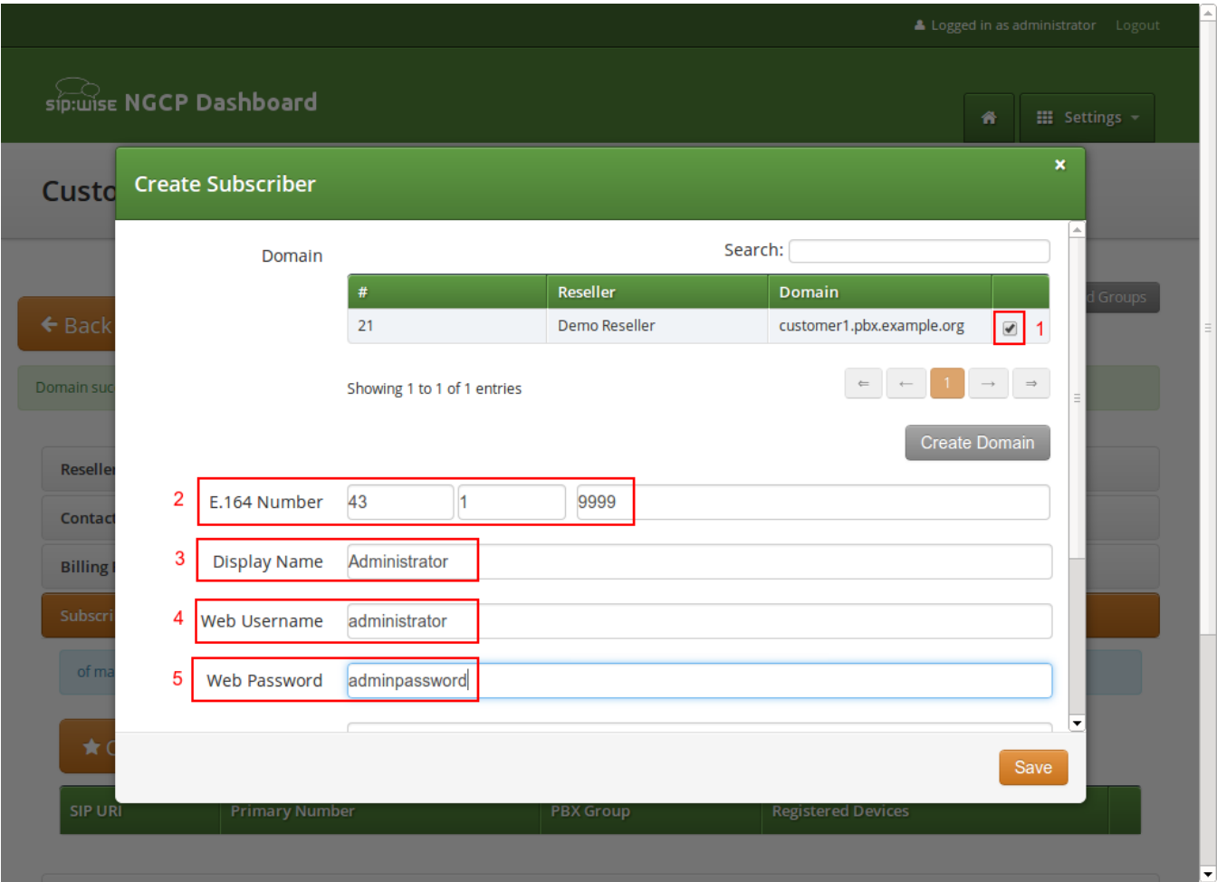
Figure 121. Create Pilot Subscriber Part 1
