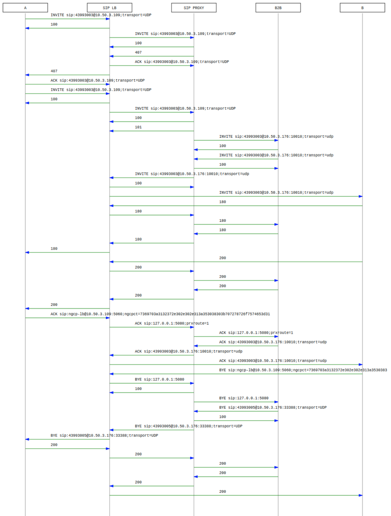
Figure 85. Basic Call Call-Flow
