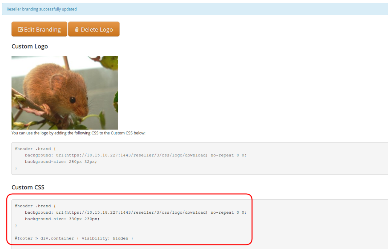
Figure 82. CSC Customisation: Custom data on panel
