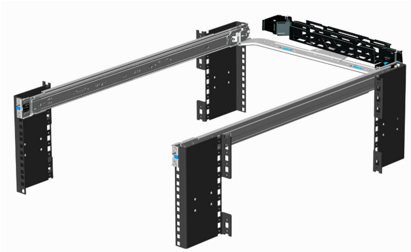
Figure 8. Rack-mounted Rails
